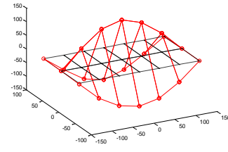
Butterfly Mode 1 f_6=80.058 Hz
