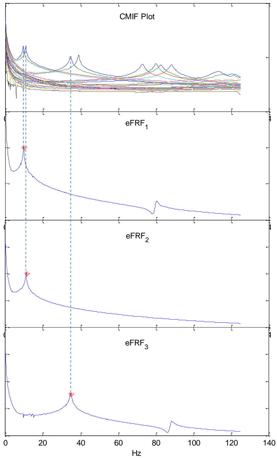
Figure 3.3: Decoupling Modes with eFRF Creation
