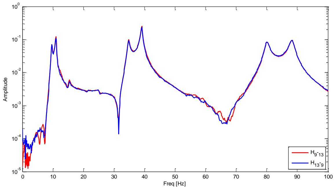
Figure 5.14: Reciprocity Check from Grid Impact Test
