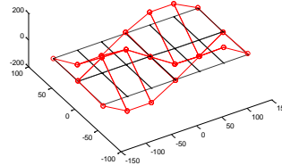
Butterfly Mode 2 f_8=88.324 Hz
