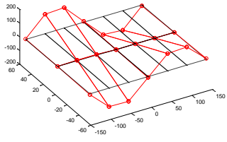
Torsion Mode 2 f_4=38.996 Hz
