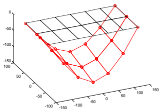
Bending Mode 1 f_1=9.570 Hz
