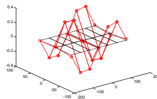
Butterfly Mode 2 f_8 = 88.737 \text{ Hz}
