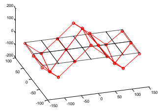
Bending Mode 3 f_5=72.831 Hz
