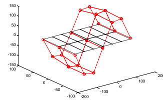
Bending Mode 2 f_3=34.714 Hz
