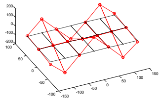
Torsion Mode 3 f_7=82.695 Hz
