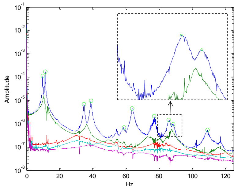
Figure 8.5: CMIF Plot - All sensors for Damage Case #2
