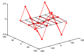
Torsion Mode 3 f_7 = 82.787 \text{ Hz}
