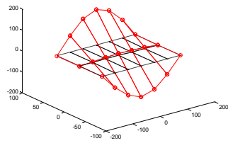
Torsion Mode 1 f_2=10.958 Hz
