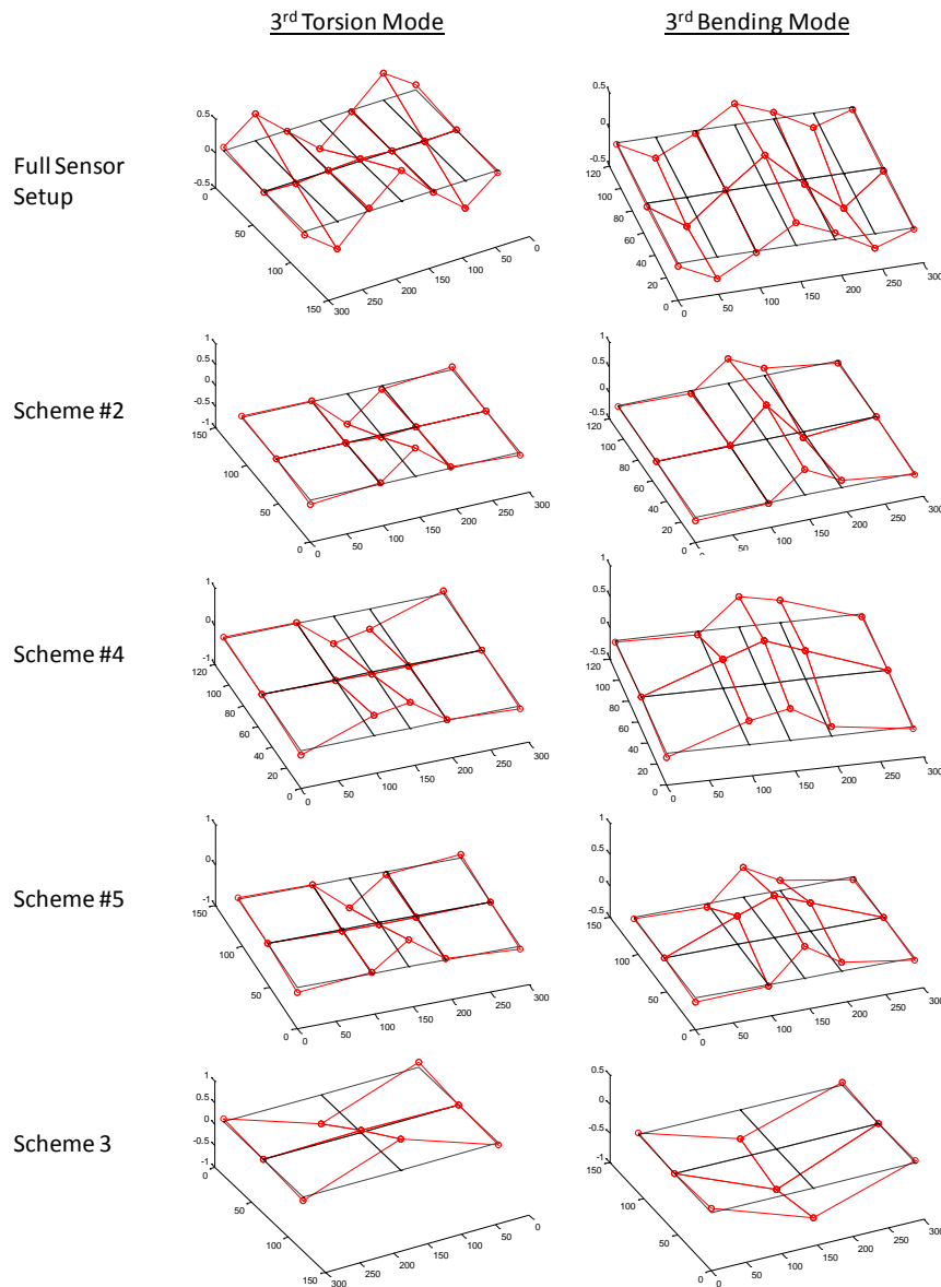
Figure 8.10: Spatial Resolution Example
