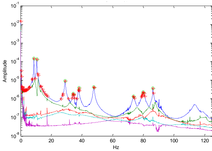
Figure 6.6: CMIF Plot – Shaker Test for Damage Case #1
