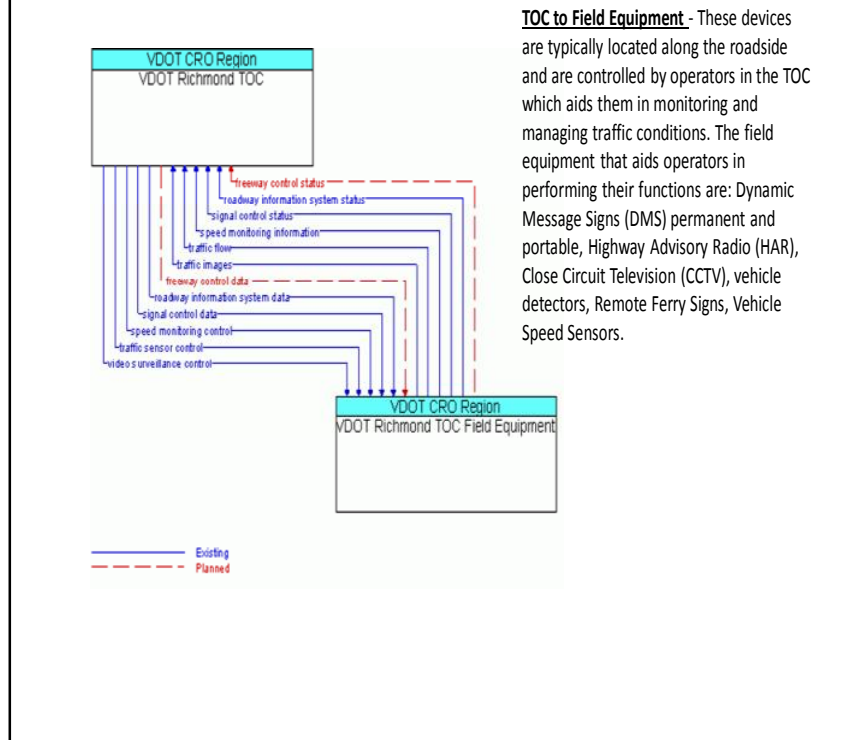
Figure 3.7 Traffic Operations Center to Field ITS Data Flow Diagram
