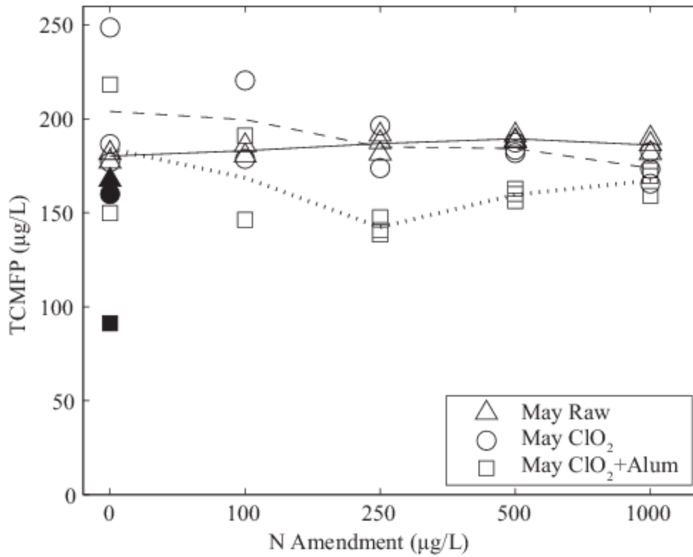
Figure 6 – Trichloromethane formation potential (TCMFP) as a function of nitrogen (N) amendment for May 30 raw and treated waters ( \text{ClO}_2 dose of 1 \text{ mg L}^{-1} as \text{Cl}_2 and alum dose of 40 \text{ mg L}^{-1} ). The P dose for all N-amended samples was 200 \text{ } \mu\text{g L}^{-1} . Lines represent triplicate averages; filled markers represent blank samples without any nutrient amendment.
