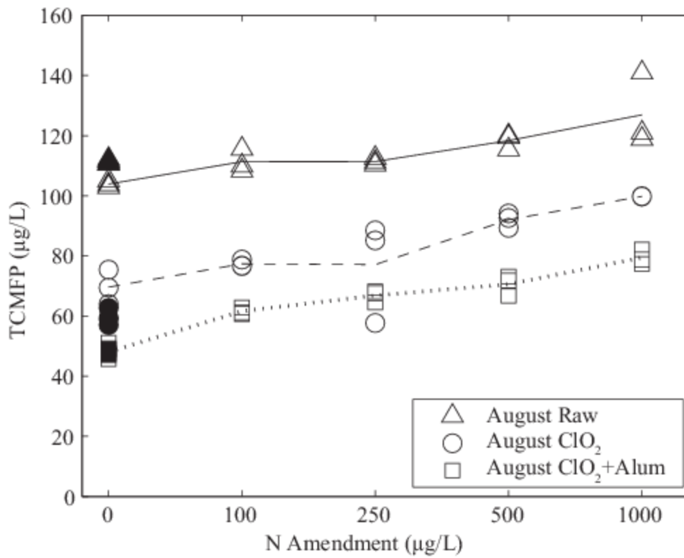
Figure 8 – Trichloromethane formation potential (TCMFP) as a function of nitrogen (N) amendment for August 19 raw and treated waters (ClO 2 dose of 2 mg L -1 as Cl 2 and alum dose of 80 mg L -1 ). The P dose for all N-amended samples was 200 µg L -1 . Lines represent triplicate averages; filled markers represent blank samples without any nutrient amendment.
