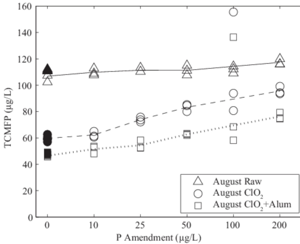
Figure 9 – Trichloromethane formation potential (TCMFP) as a function of phosphorus (P) amendment for August 19 raw and treated waters (ClO 2 dose of 2 mg L -1 as Cl 2 and alum dose of 80 mg L -1 ). The N dose for all P-amended samples was 2,000 µg L -1 . Lines represent triplicate averages except for the P = 100 µg L -1 dose, which was excluded. Filled markers represent blank samples without any nutrient amendment.
