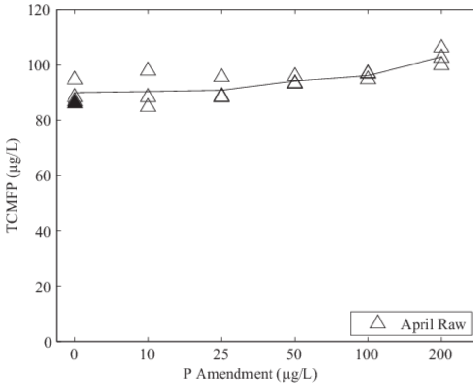
Figure 5 – Trichloromethane formation potential (TCMFP) as a function phosphorus (P) amendment for April 5 raw water. The N dose for all P-amended samples was 2,000 µg L -1 . Lines represent triplicate averages; filled markers represent blank samples without any nutrient amendment.
