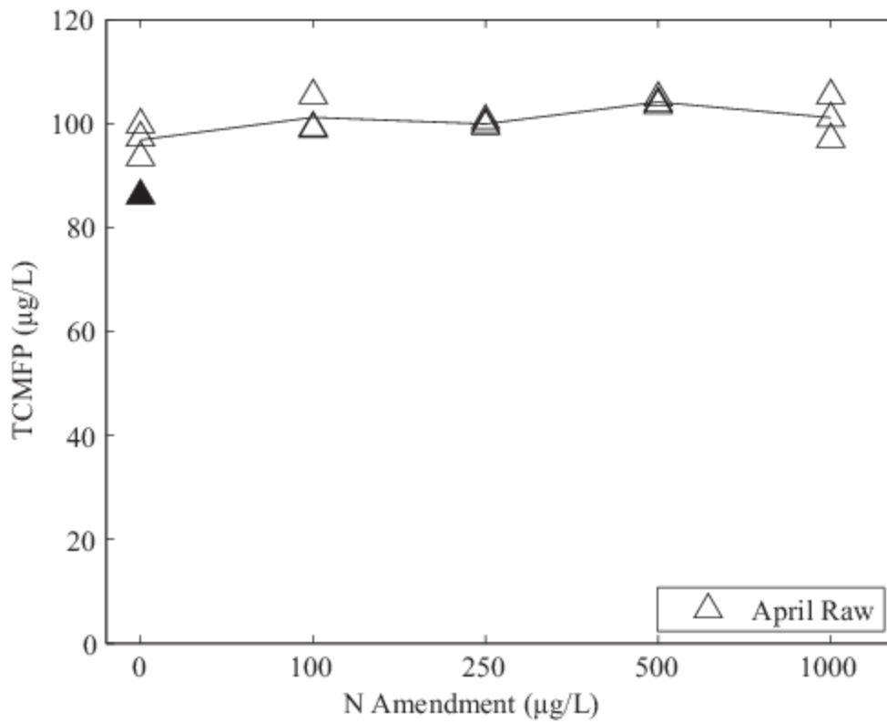
Figure 4 – Trichloromethane formation potential (TCMFP) as a function of nitrogen (N) amendment for April 5 raw water. The P dose for all N-amended samples was 200 \mu\text{g L}^{-1} . Lines represent triplicate averages; filled markers represent blank samples without any nutrient amendment.
