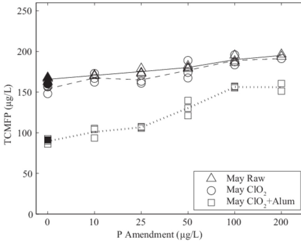
Figure 7 – Trichloromethane formation potential (TCMFP) as a function of phosphorus (P) amendment for May 30 raw and treated waters (ClO 2 dose of 1 mg L -1 as Cl 2 and alum dose of 40 mg L -1 ). The N dose for all P-amended samples was 2,000 µg L -1 . Lines represent triplicate averages; filled markers represent blank samples without any nutrient amendment.
