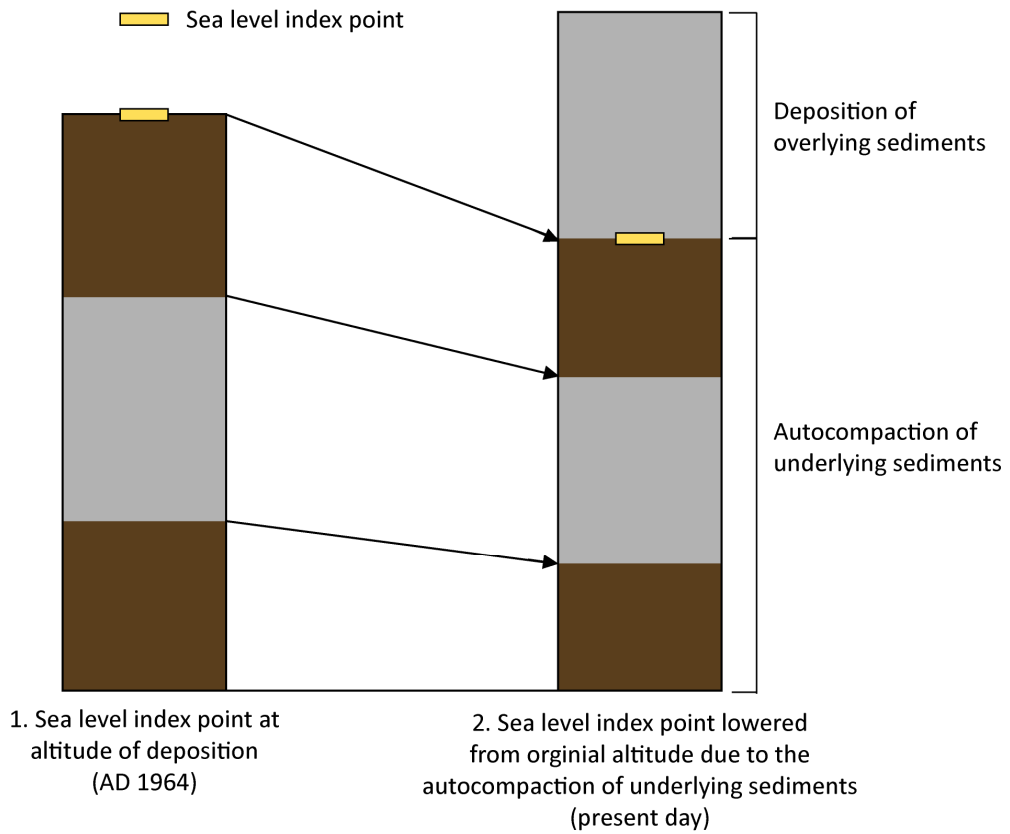
Figure 6.5 - The effect of autocompaction on a sea level index point. The sea level index point is lowered from the altitude of deposition due to the compaction of underlying sediments by the overburden sediments (modified from Brain (2006) Figure 2.10).
