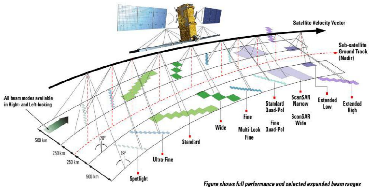
Figure 3.10: Radarsat-2 SAR beam modes of operation (Adapted from MDA, 2007).
