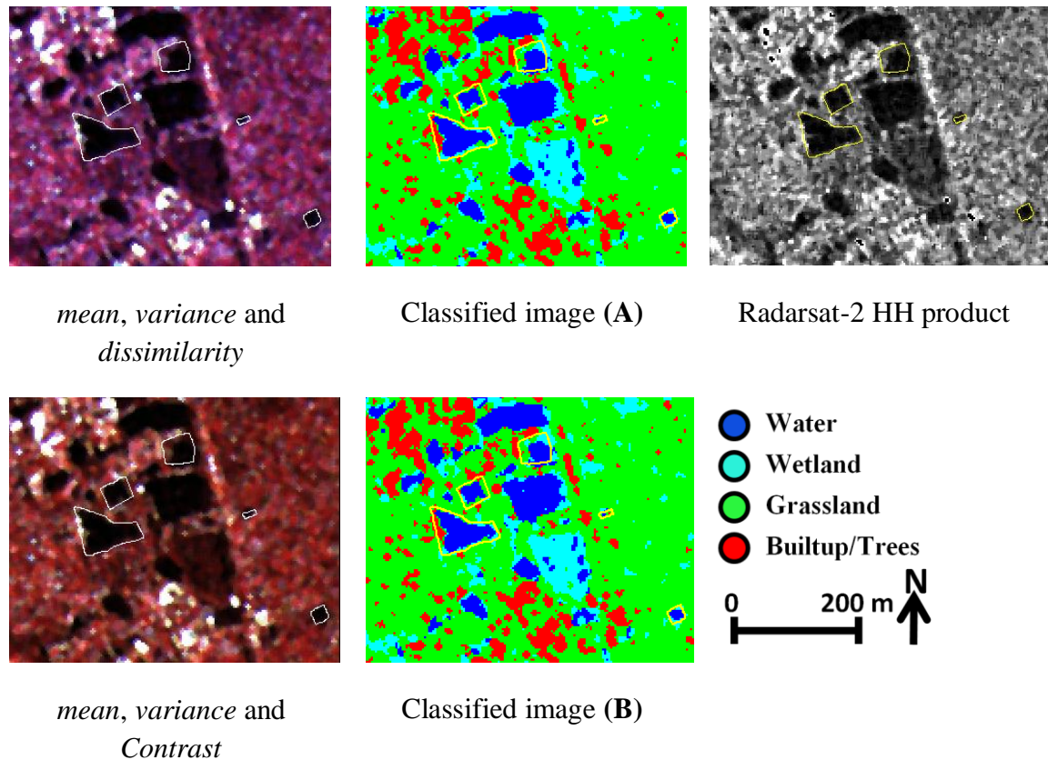
Figure 7.14: Supervised classification of Radarsat-2 HH produced after applying co-occurrence variables of (A) mean, variance and dissimilarity , and (B) mean, variance and contrast overlaid with dGPS data
