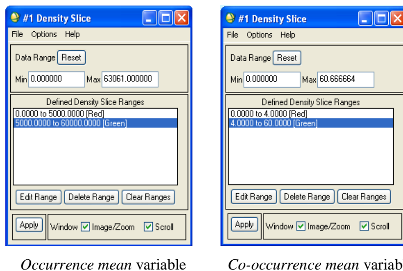
Figure 7.2: Defining density slice ranges for Water class using co-occurrence and occurrence mean variable - Radarsat-2-HH image.
