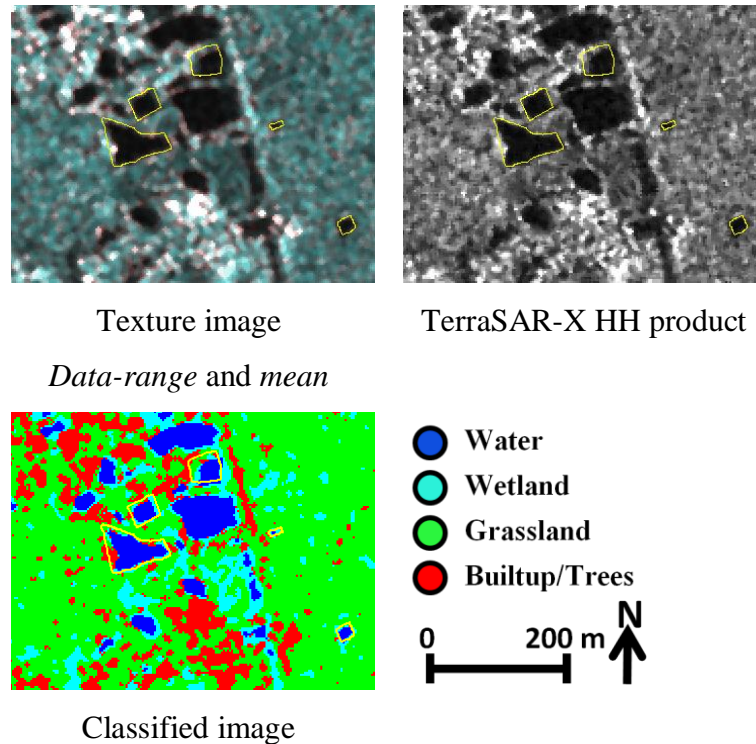
Figure 7.15: Supervised classification of occurrence data-range and mean texture image for TerraSAR-X HH Stripmap overlaid with dGPS data compared to the original SAR product and the texture image
