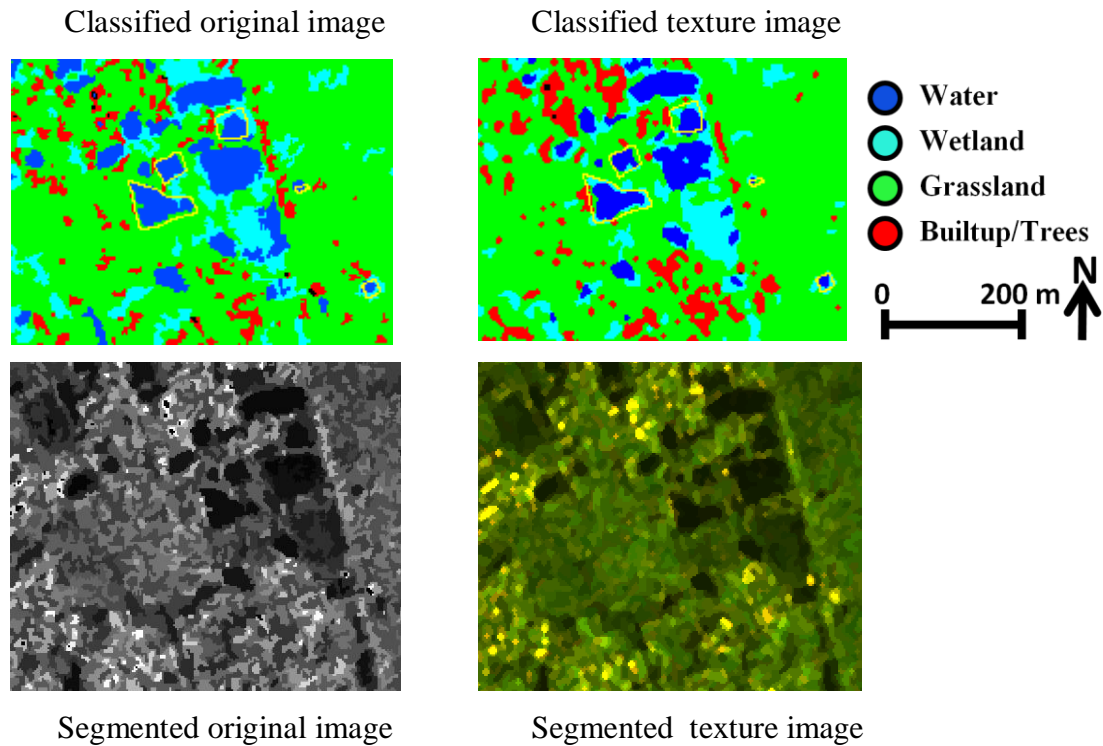
Figure 7.24: Comparison of object-oriented classification between original image and texture image ( occurrence data-range and mean ) of Radarsat-2 HH, along with the segmented images
