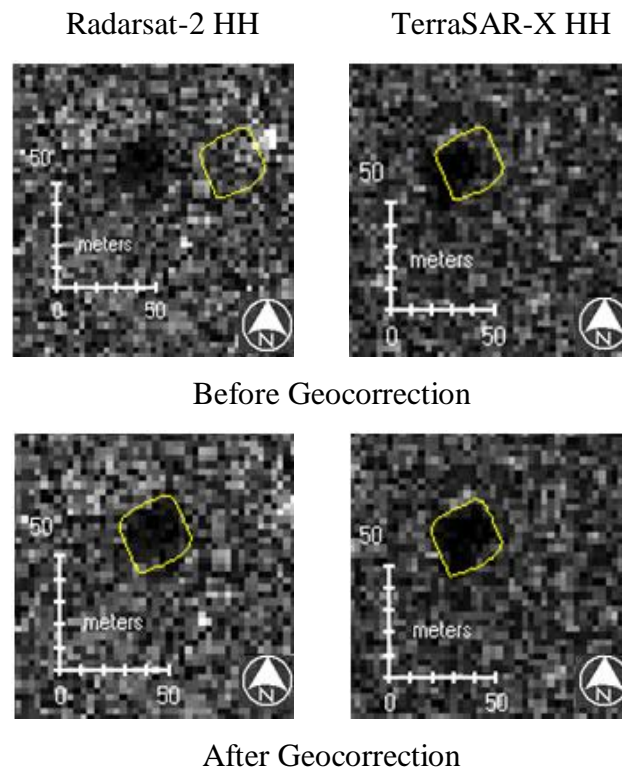
Figure 6.6: Radarsat-2 HH and TerraSAR-X HH products extracted before and after geocorrection (the dark area is a water body, while the yellow polygon is the dGPS data). Note Radarsat-2 has 46 m slight distortion while TerraSAR-X has only 8 m and both distortions are to the west.
