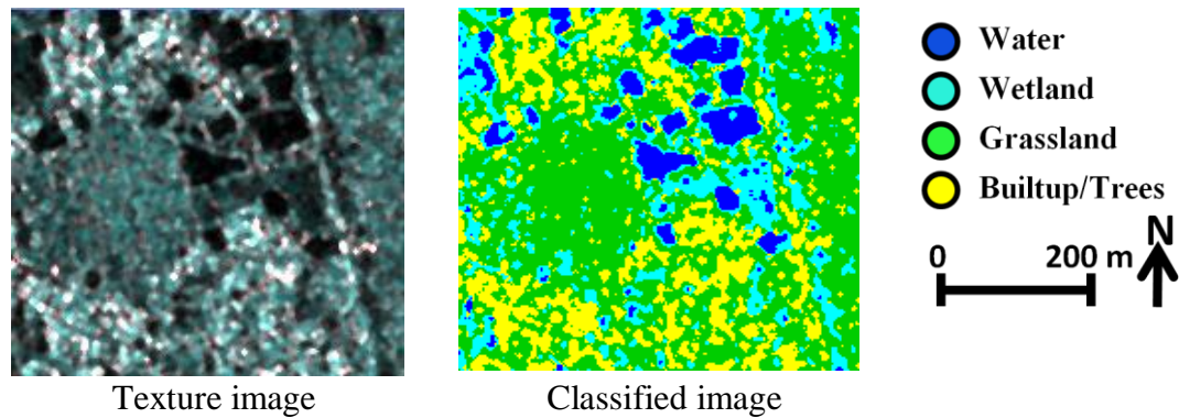
Figure 7.13: Supervised classification of occurrence data-range and mean texture image for Radarsat-2 VV compared to the texture image
