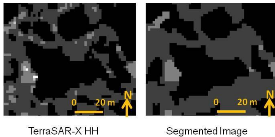
Figure 7.22: TerraSAR-X HH original image (non-texture image) before and after segmentation
