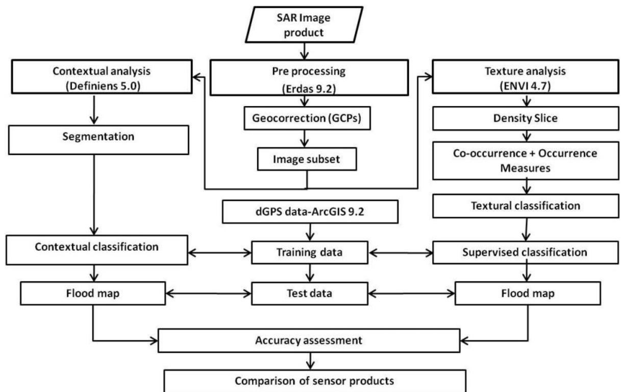
Figure 5.1: An overall workflow of the data processing methodology.
