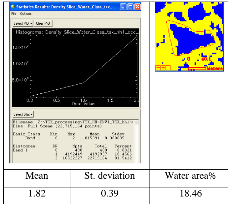
Figure 7.8: Statistical results of density slicing for water class of TerraSAR-X HH occurrence mean variable.
