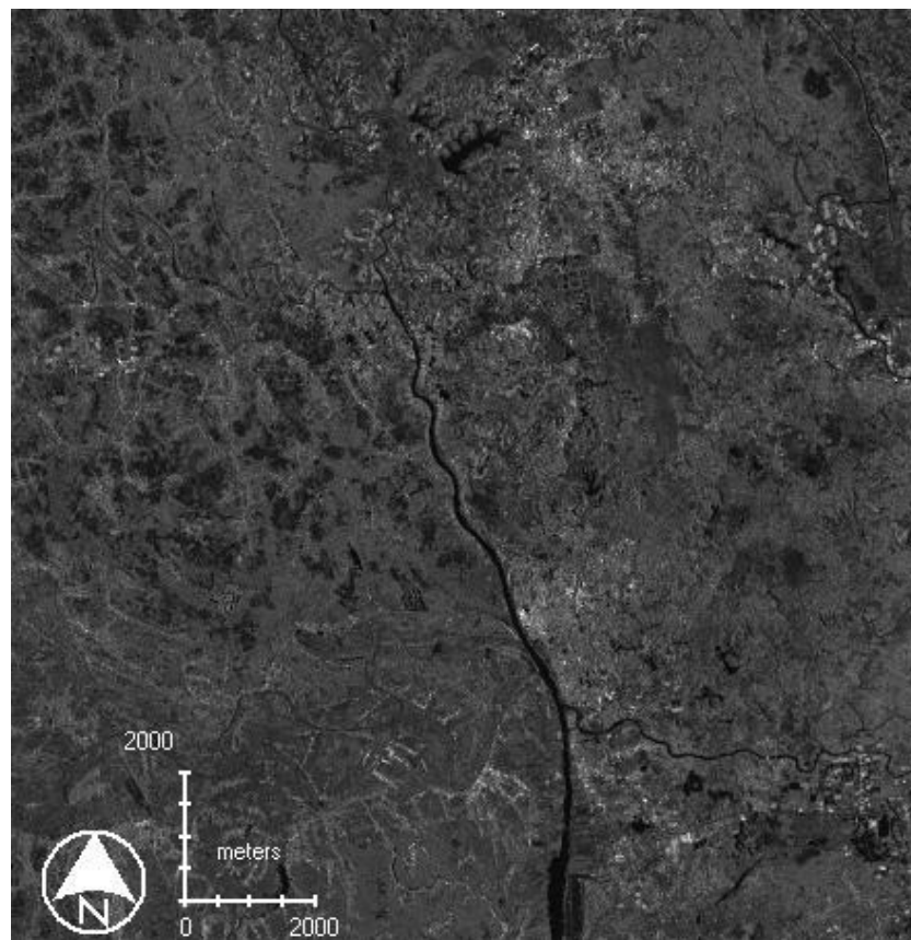
Figure 5.2: Radarsat-2 product acquired with HH polarization for the study area before Geocorrection.
