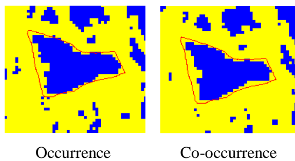
Figure 6.30: Comparison between occurrence and co-occurrence mean texture measure using density slice technique with Radarsat-2 HH.
