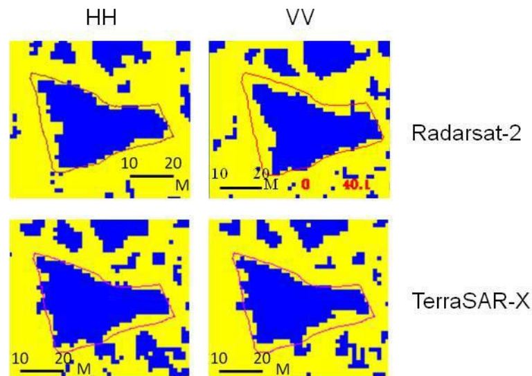
Figure 7.9: A visual comparison of SAR sensor polarizations between Radarsat-2 and TerraSAR-X.
