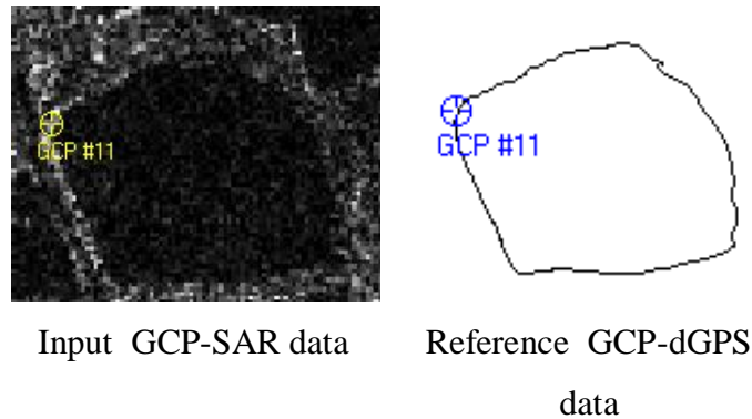
Figure 5.9: An example of a GCP extracted from a water body for both dGPS-reference and SAR-input data.
