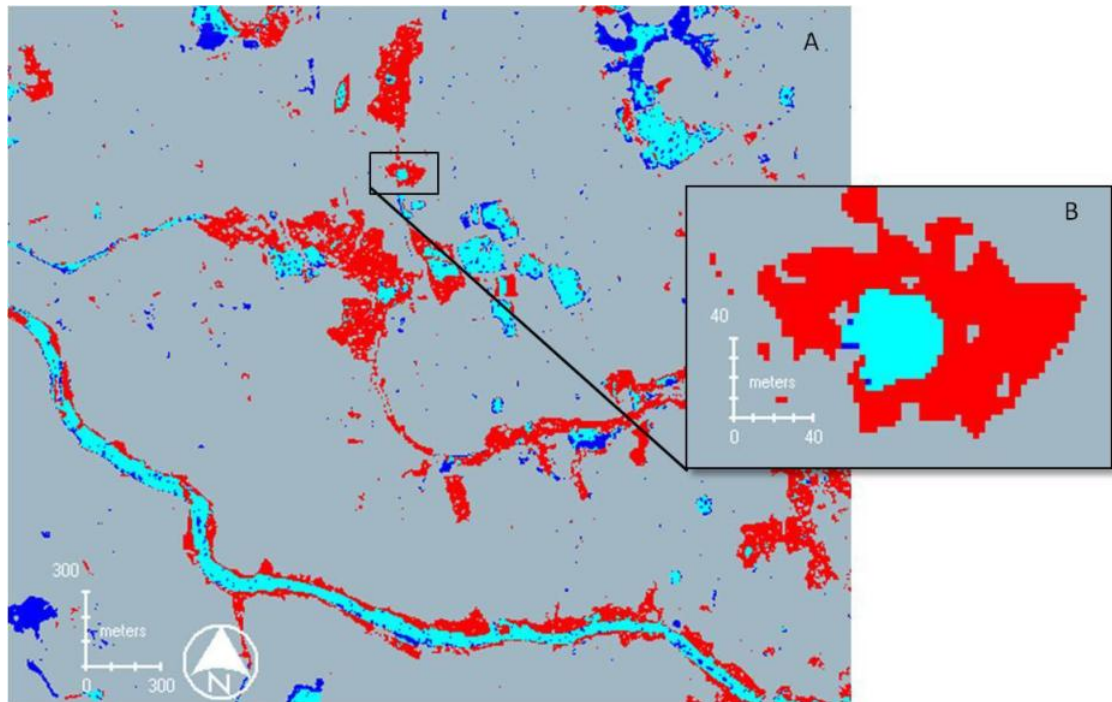
Figure 8.6: An example of discrimination between permanent water bodies and flooding extracted from TerraSAR-X HH imagery of the study area. In the zoomed in area (B) a permanent water body is shown in cyan and after flooding in red colour, showing the significance of the proposed methods. Blue (only before) and Grey (background).
