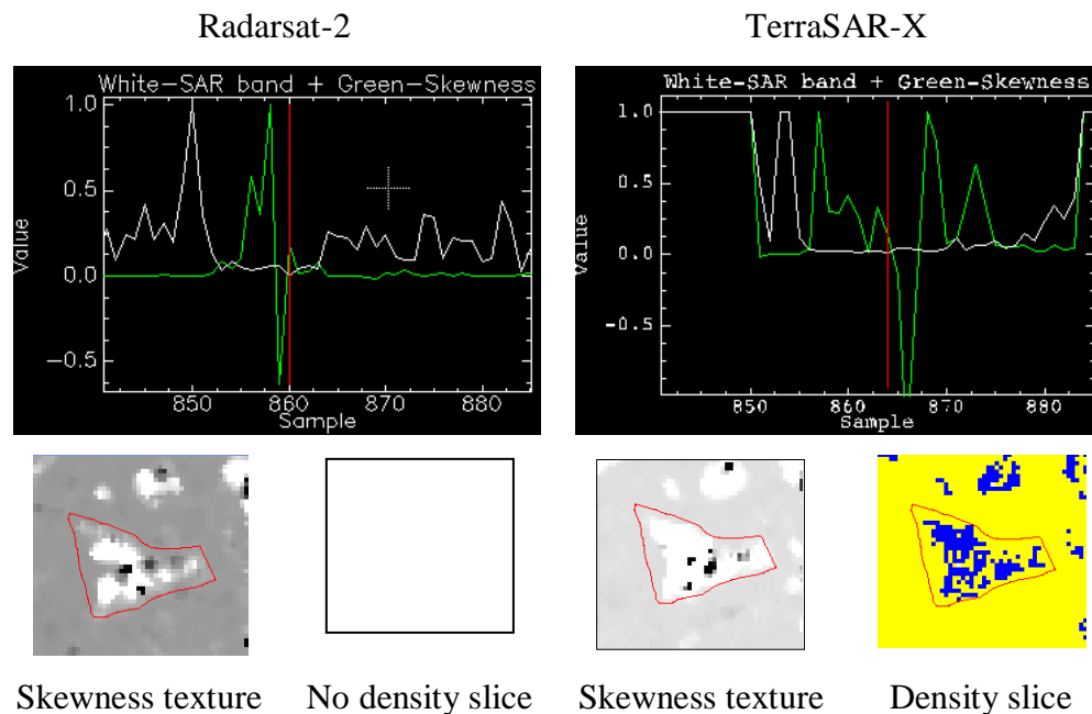
Figure 6.18: Reflectance profiles of occurrence skewness texture measure with extracted texture scenes for Radarsat-2 HH and TerraSAR-X images (note that there is no density slice range for the Radarsat-2 HH texture image since the value range is -0.00 to 0.00 ).
