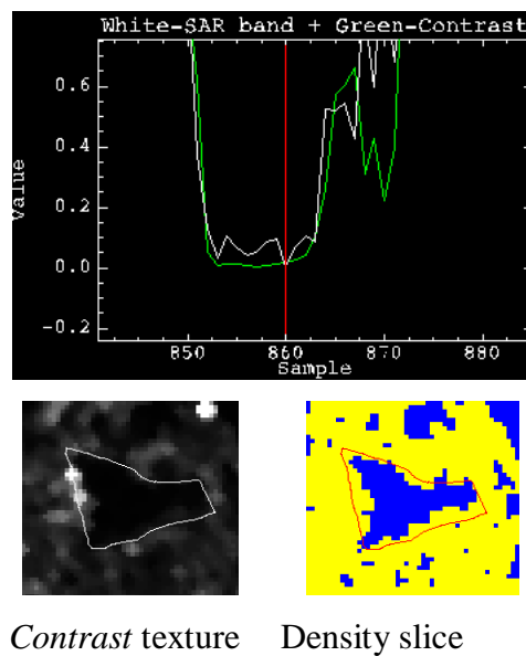
Figure 6.22: Reflectance profile of co-occurrence contrast texture measure for the Radarsat-2 HH image with extracted texture scene, and density slice in the ranges 0.0–10 (blue) and 10–1800 (yellow).
