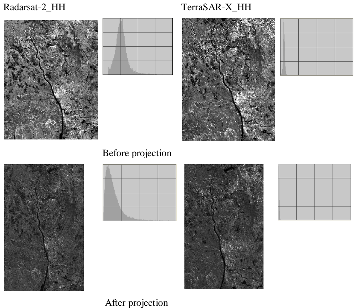
Figure 6.4: Radarsat-2 and TerraSAR-X in HH polarization with their histograms before and after projection.
