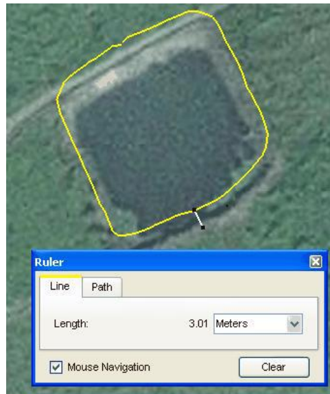
Figure 6.8: Distance of distortion of a water body extracted from Google Earth, 2010, overlaid with dGPS data. Note the distortion measured approximately 3 metres.
