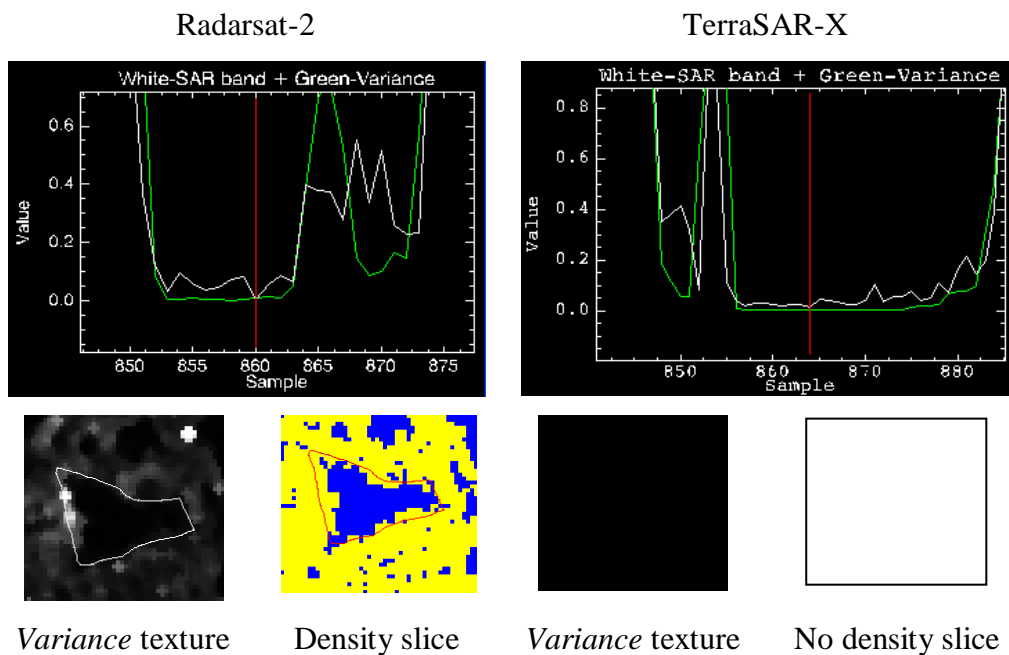
Figure 6.16: Reflectance profiles of occurrence variance texture measure with extracted texture scene for Radarsat-2 HH and TerraSAR-X images (note that there is no output texture signature for the TerraSAR-X image and accordingly no density slice).
