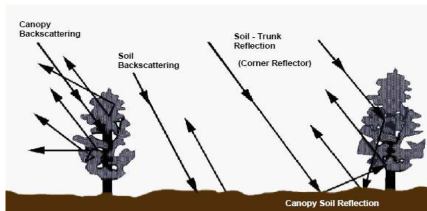
Figure 3.5: Radar energy scattering from different surfaces. Note that trunks of trees may cause the corner reflector effect (adapted from Globe SAR, 2008).
