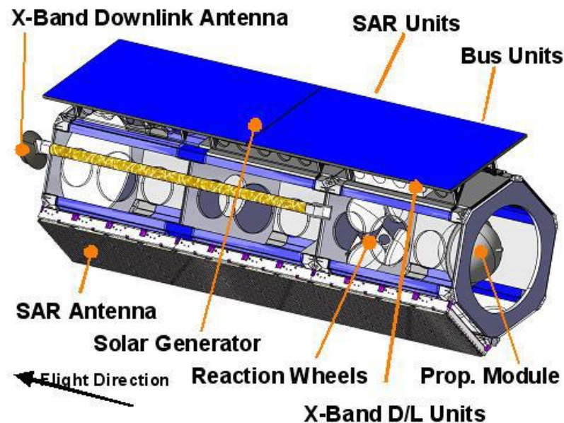
Figure 3.11: TerraSAR-X system components (DLR, 2011b).
