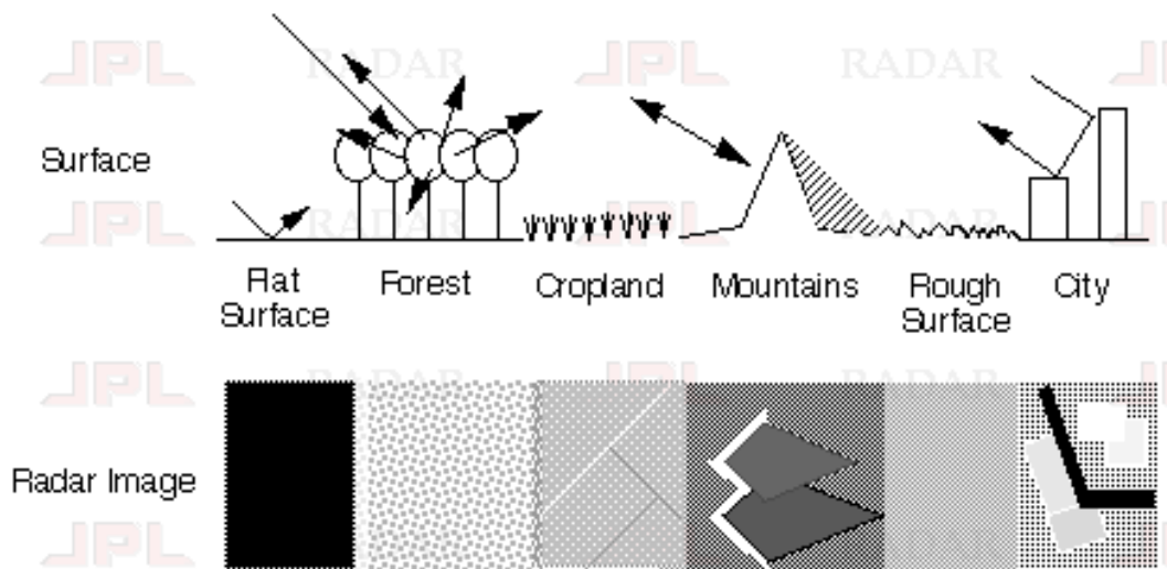
Figure 3.7: Imaging different types of surface with radar. Note how surfaces appear in a radar image (adapted from JPL-Freeman, 1996).
