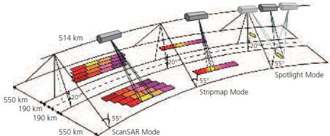
Figure 3.12: TerraSAR-X SAR modes of operation (source: DLR, 2009).
