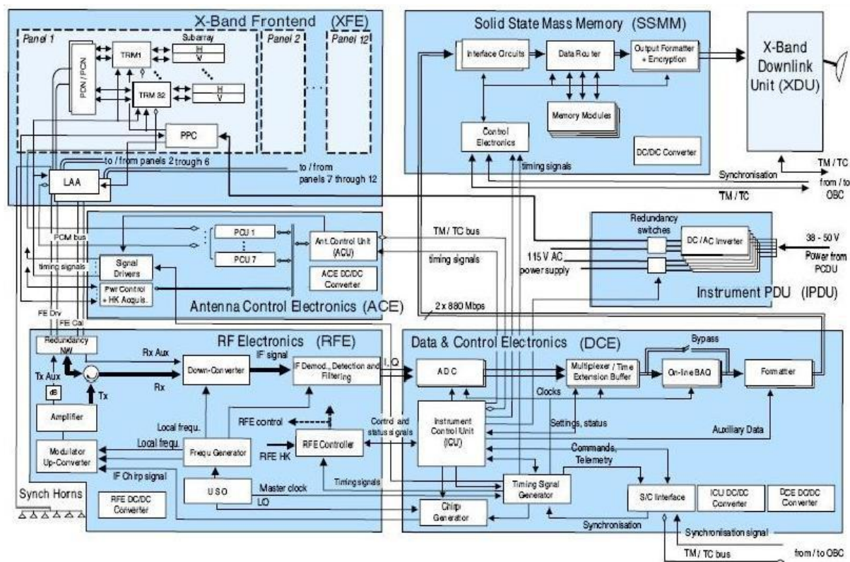
TerraSAR-X instrument functional Unit block diagram (Source: DLR, EADS)
