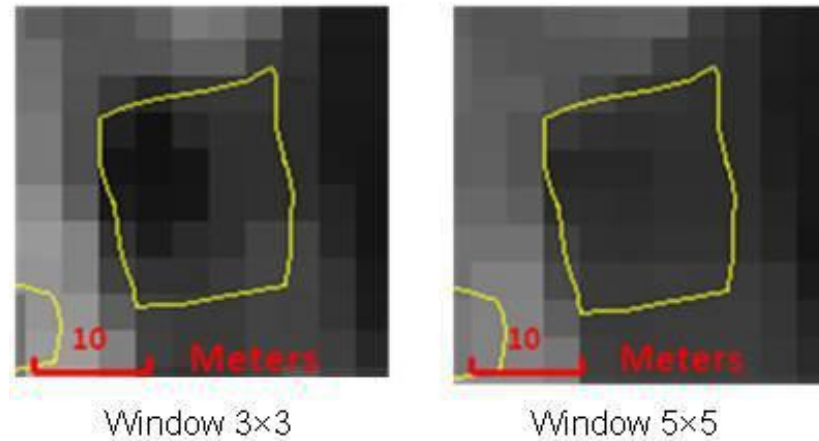
Figure 6.12: A comparison between 3×3 and 5×5 window sizes of enhanced median filter with an area of 238m 2 – note that the 5×5 window size shows less intensity.
