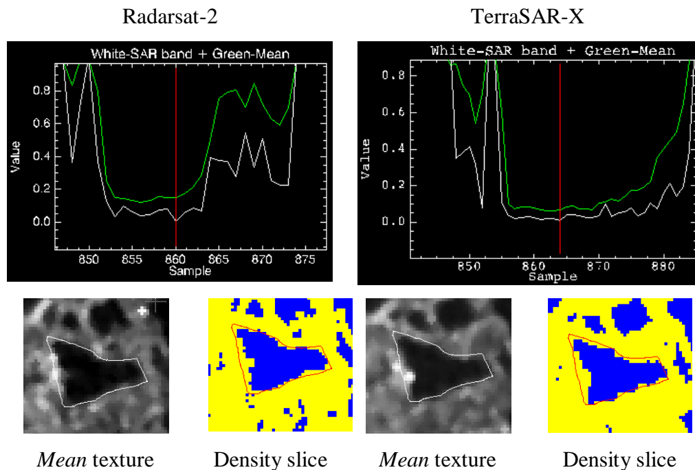
Figure 6.15: Reflectance profiles of occurrence mean texture measure for Radarsat-2 and TerraSAR-X HH images with extracted texture scenes smoothed by median 3 \times 3 window, along with density slice scenes.
