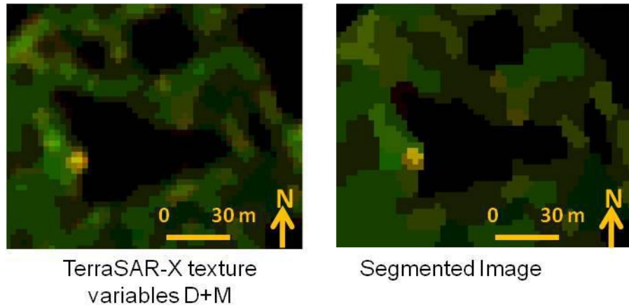
Figure 7.21: TerraSAR-X HH texture image ( data-range and mean ) before and after segmentation
