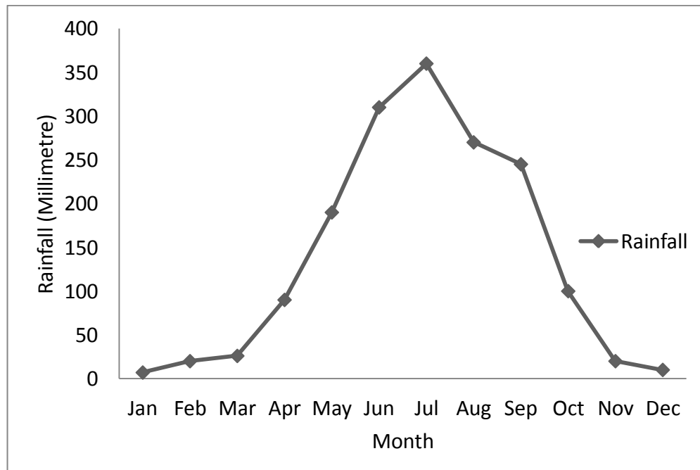
Figure 4.6: Average mean monthly rainfall in millimetre of the study area (modified from SRDI, 1997, in Huda, 2004).
