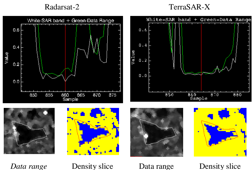
Figure 6.14: Reflectance profiles of occurrence data range texture measure with extracted texture scenes smoothed by median 3 \times 3 window, along with density sliced scenes for Radarsat-2 and TerraSAR-X HH images.
