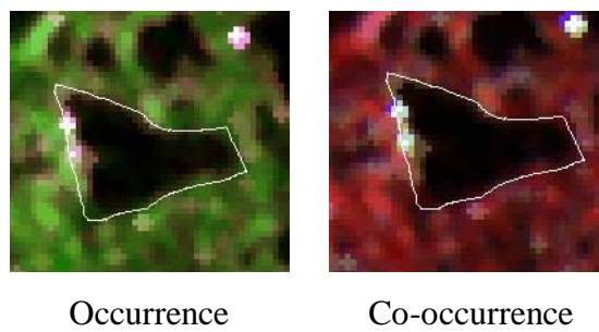
Figure 6.29: Comparison between occurrence and co-occurrence combined texture measures with Radarsat-2 HH.
