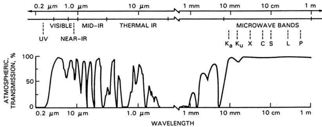
Figure 3.1: The electromagnetic spectrum showing the Visible, Near IR, Middle IR, Thermal IR, and Microwave regions and the efficiency of atmospheric transmission (Lewis and Henderson, 1998).
