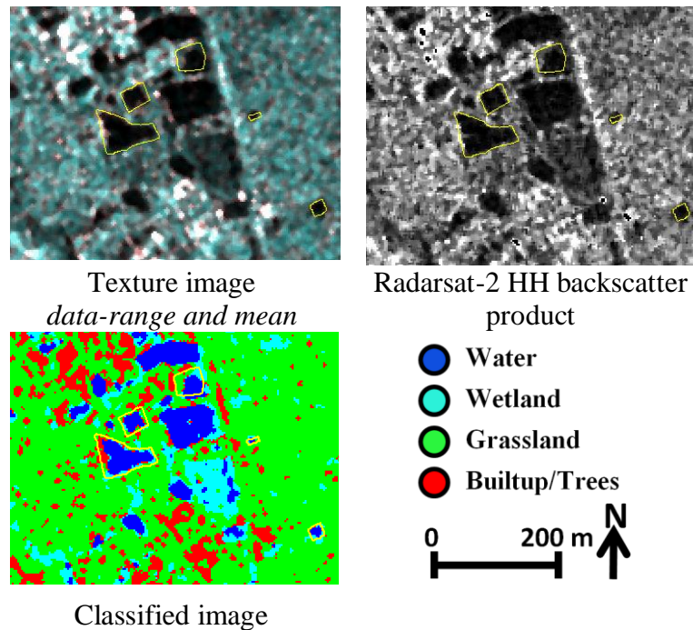
Figure 7.12: Supervised classification of occurrence data-range and mean texture image for Radarsat-2 HH overlaid with dGPS data compared to the original SAR product and the texture image; maps shown here and subsequent maps cover a small portion of the study area.
