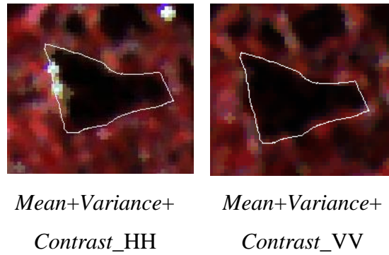
Figure 6.28: Texture analysis for products of Radarsat-2 HH and VV polarizations with a combination of co-occurrence measures.
