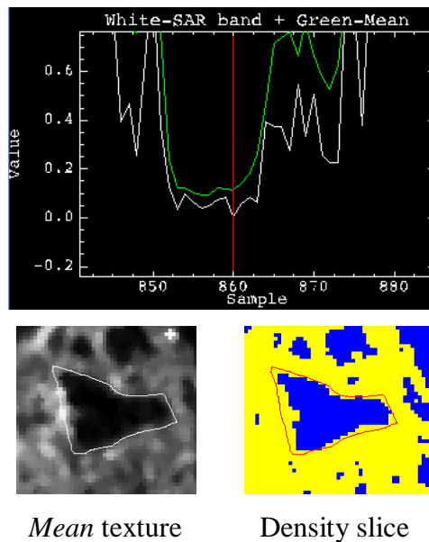
Figure 6.19: Reflectance profile of co-occurrence mean texture measure for the Radarsat-2 HH image with extracted texture scene, and density slice in the ranges 0.0–4 (blue) and 4.0–60 (yellow).
