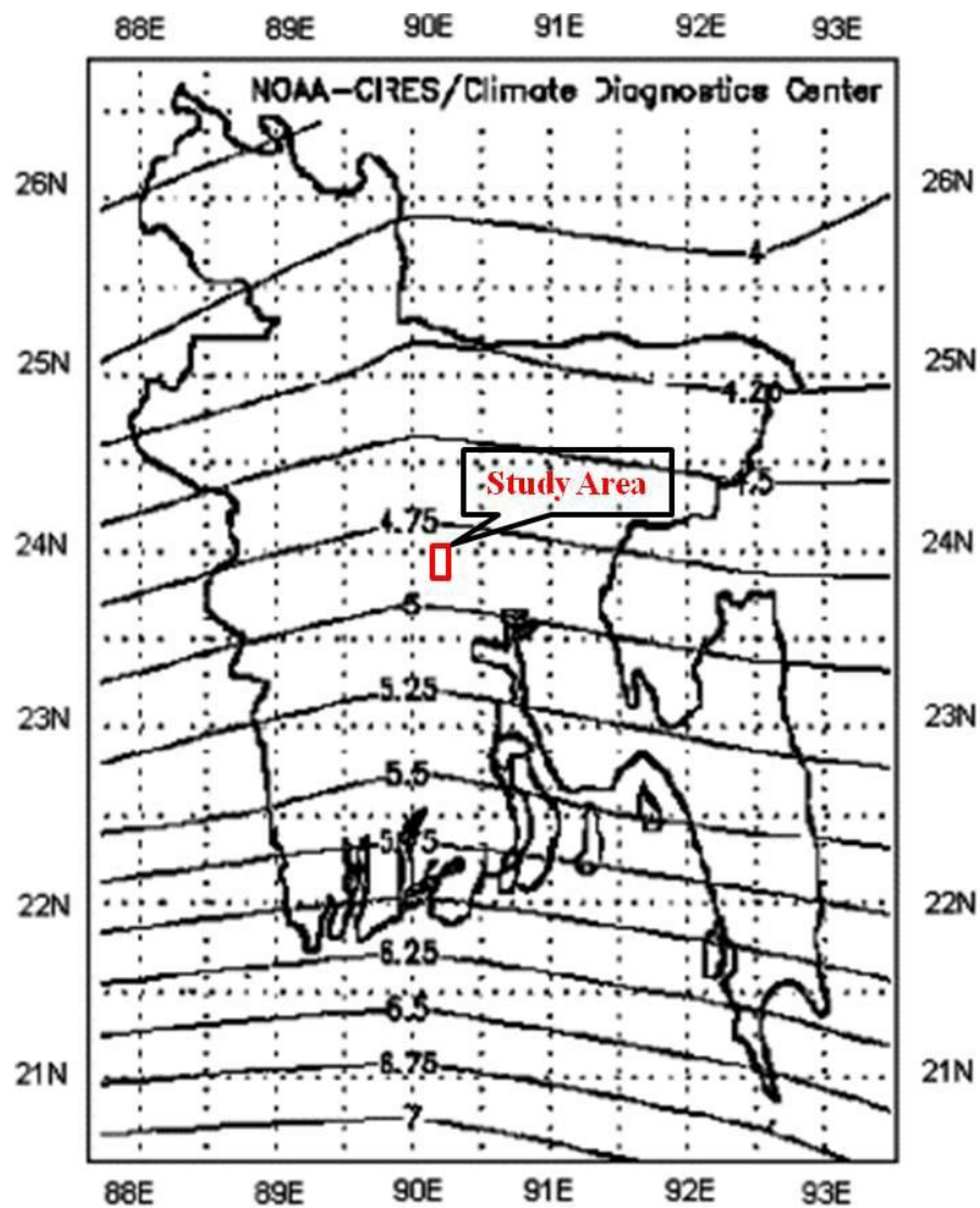
Figure 4.7: Average wind speed (m/s) in Bangladesh at surface level from January to December (adapted from Khan et al., 2004).
