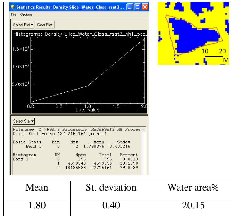
Figure 7.5: Statistical results of density slicing for water class with occurrence mean variable - Radarsat-2 HH.
