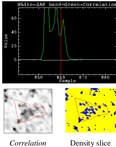
Figure 6.26: Reflectance profile of co-occurrence correlation texture measure for the Radarsat-2 HH image with extracted texture scene, and density slice in the ranges -25 to -7 (blue) and -7 to 4 (yellow).
