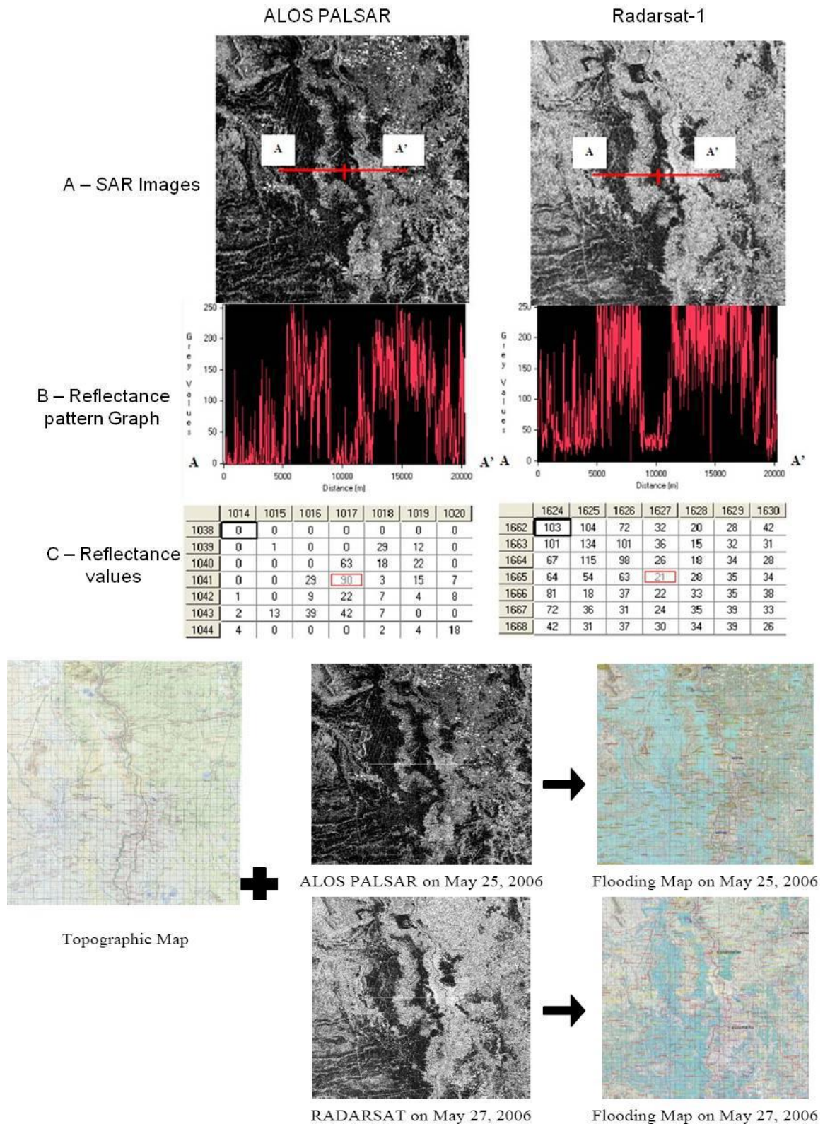
Figure 3.8: Reflectance significance comparison and flooding map using ALOS PALSAR and Radarsat-1 merged with a topographic map (A- SAR images, B-reflectance pattern graph, and C-reflectance values) (adapted from Komwong and Simking, 2006).
