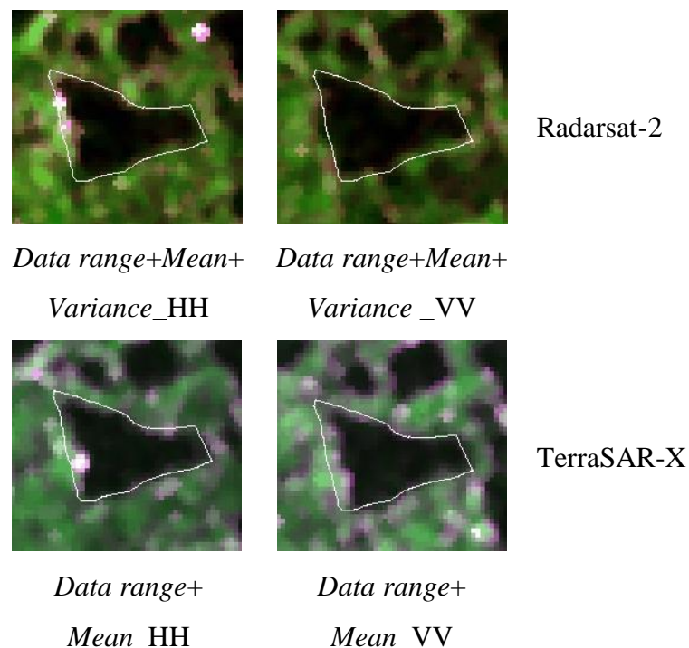
Figure 6.27: Texture analysis for products of both sensors with HH and VV polarizations with a combination of occurrence measures.
