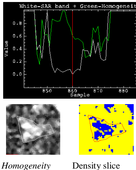
Figure 6.21: Reflectance profile of co-occurrence homogeneity texture measure for the Radarsat-2 HH image with extracted texture scene, and density slice in the ranges 0.0–0.4 (yellow) and 0.4–0.8 (blue).
