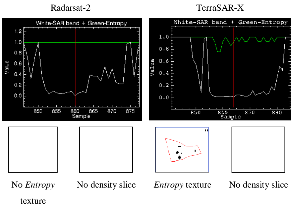
Figure 6.17: Reflectance profiles of occurrence entropy texture measure for Radarsat-2 HH and TerraSAR-X HH images (note that there is no output texture signature other than a solid white colour, and as a result there is no density slice).
