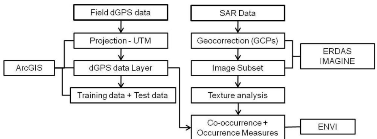
Figure 6.1: Methodology flow chart of data preparation.
