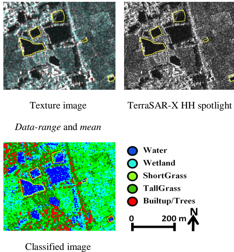
Figure 7.17: Supervised classification of occurrence data-range and mean texture image for TerraSAR-X HH spotlight overlaid with dGPS reference data in yellow compared to the original SAR product and the texture image
