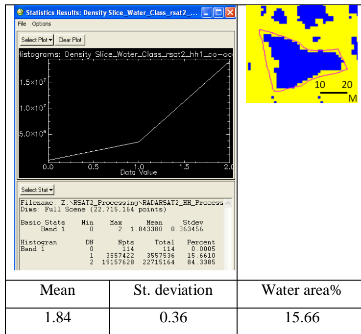
Figure 7.4: Statistical results of density slicing for water class with co-occurrence mean variable - Radarsat-2 HH.
