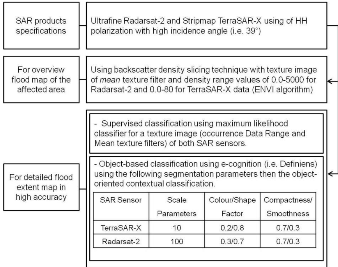
Figure 8.7: Outline of the water area mapping proposed methods for operational flood disaster applications for flat topography areas.
