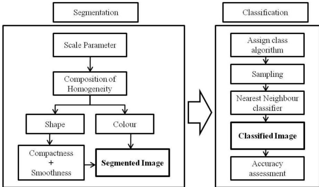
Figure 5.13: Methodology flow chart of the contextual classification used for segmentation and object-oriented classification.
