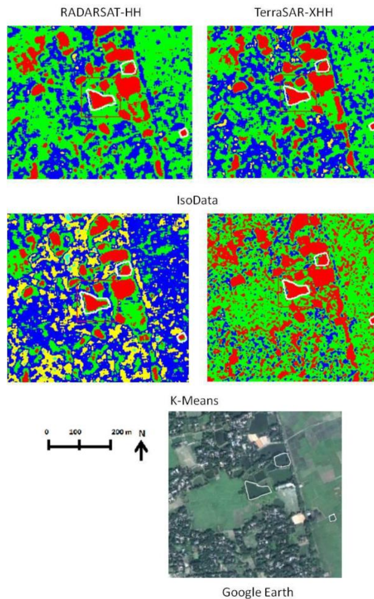
Figure 7.10: Unsupervised classification ISODATA and K-Means comparison between RADARSAT-2 and TerraSAR-X images (red indicates water); maps shown here cover a small portion of the study area.
