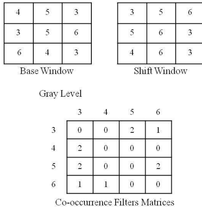
Figure 5.10: Co-occurrence matrix (Haralick et al., 1973).
