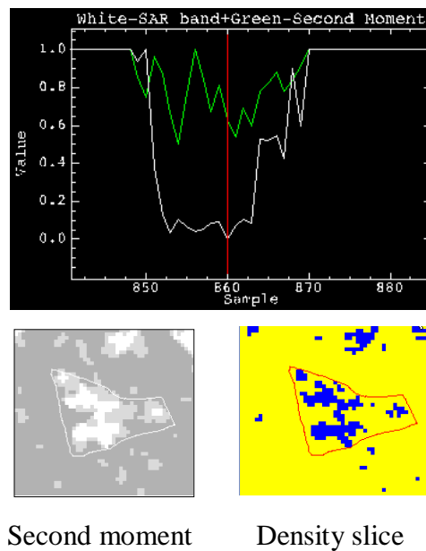
Figure 6.25: Reflectance profile of co-occurrence second-moment texture measure filter for the Radarsat-2 HH image with extracted texture scene, and density slice in the ranges 0.0– 0.14 (yellow) and 0.14–0.4 (blue).
