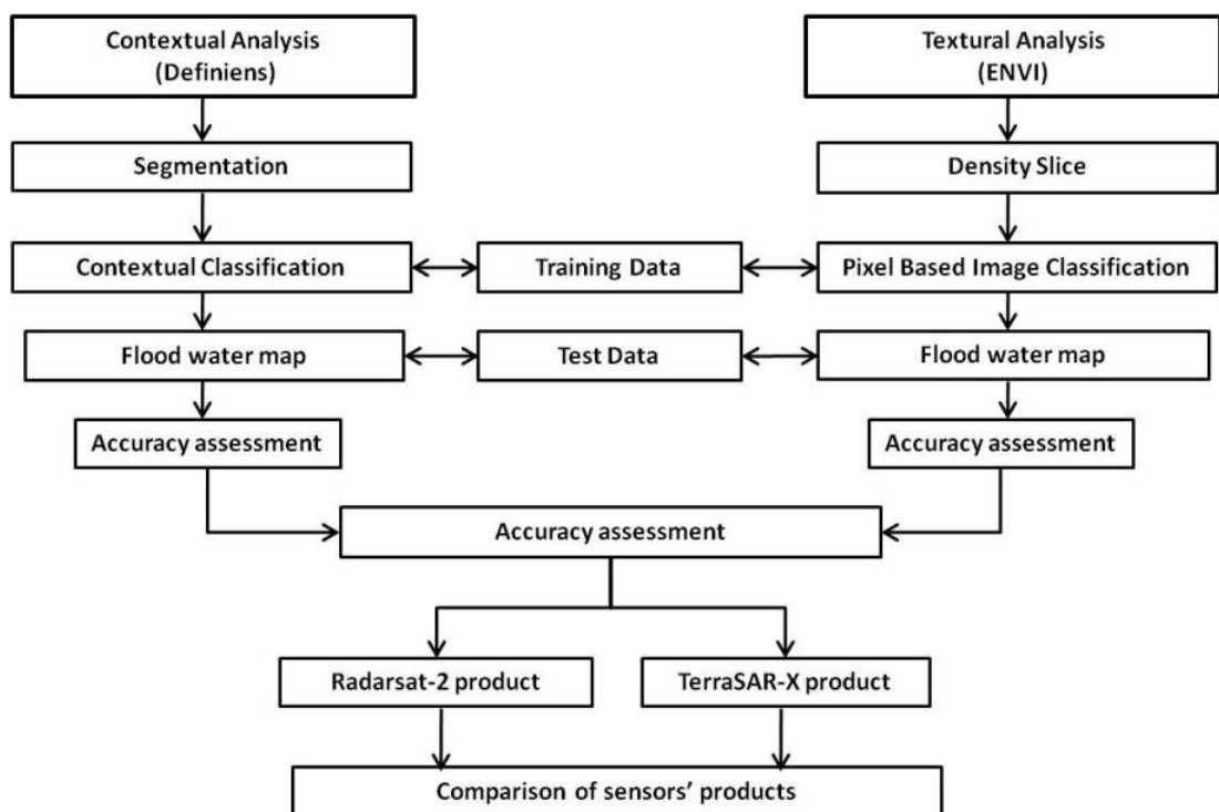
Figure 7.1: Methodology flow chart of water body mapping and accuracy assessment.
