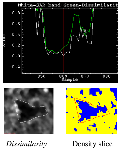
Figure 6.23: Reflectance profile of co-occurrence dissimilarity texture measure filter for the Radarsat-2 HH image with extracted texture scene, and density slice in the ranges 0.0–2.5 (blue) and 2.5–39 (yellow).
