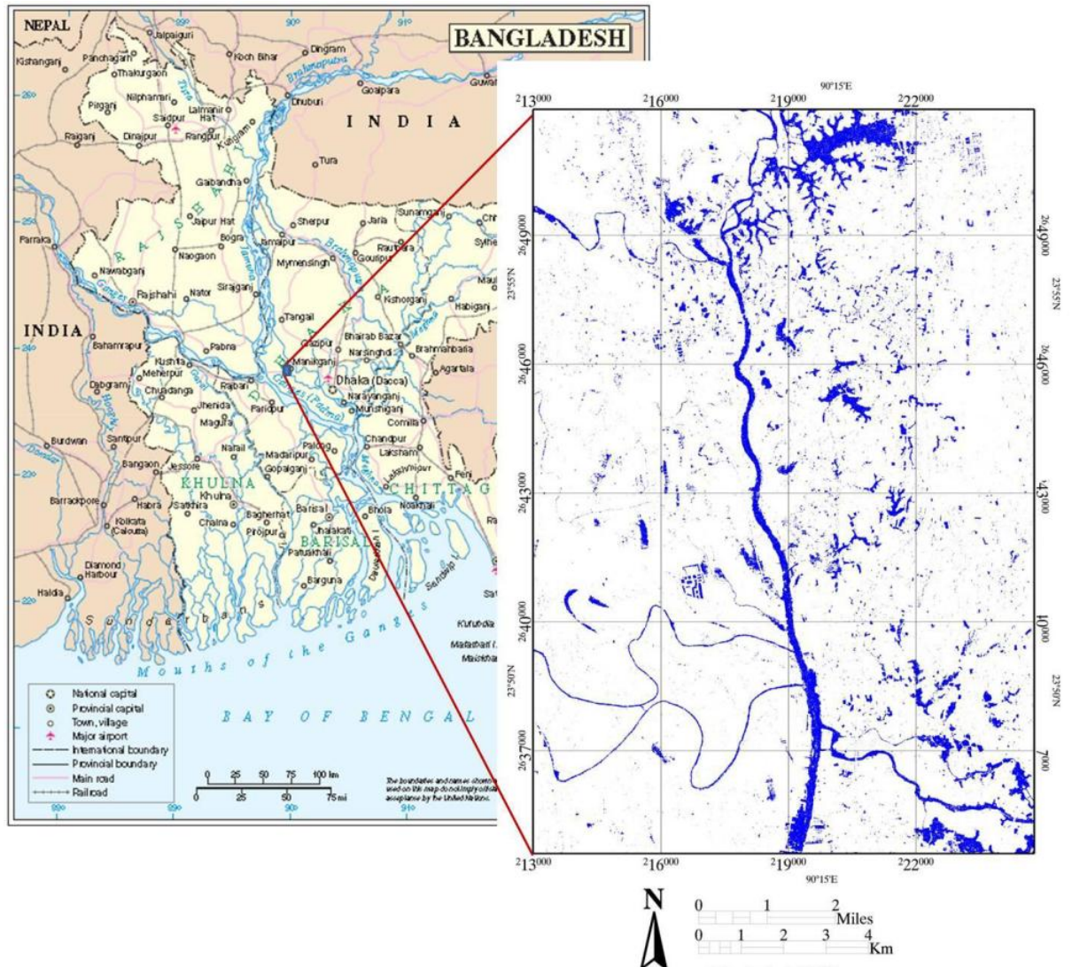
Figure 5.6: Study area extracted from Radarsat-2 HH image showing water bodies extracted from density slice analysis (Bangladesh map adapted from UNHCR, 2004).
