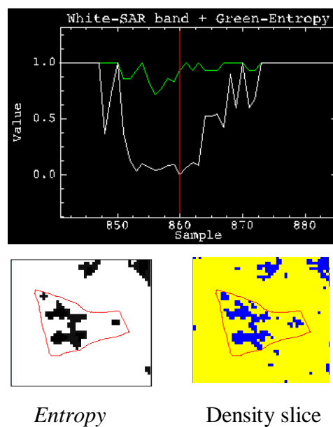
Figure 6.24: Reflectance profile of co-occurrence entropy texture measure for the Radarsat-2 HH image with extracted texture scene, and density slice in the ranges 0.0–2 (blue) and 2–2.2 (yellow).
