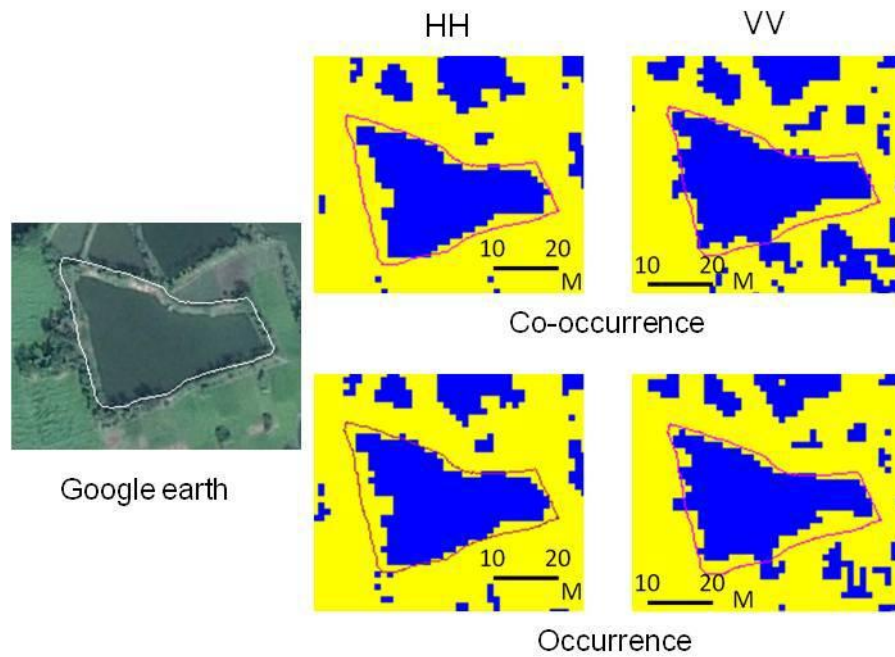
Figure 7.3: Example of density sliced results of co-occurrence and occurrence mean variable - Radarsat-2 HH and VV.
