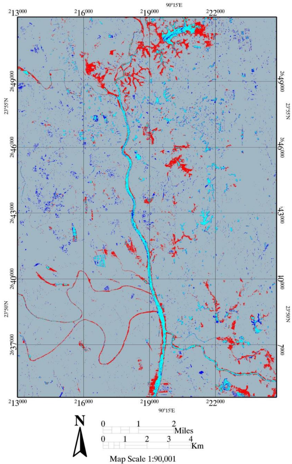
Figure 8.8: Changes detection using TerraSAR-X HH showing flooding in red. Colour code: Blue- WBs before; Red- WBs after; Cyan-no change; Grey- background.
