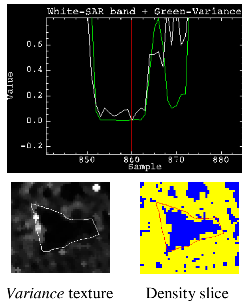
Figure 6.20: Reflectance profile of co-occurrence variance texture measure for the Radarsat-2 HH image with extracted texture scene, and density slice in the ranges 0.0–5 (blue) and 5–800 (yellow).
