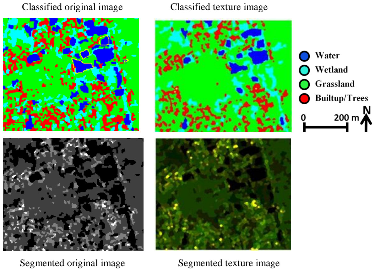
Figure 7.25: Comparison of object-oriented classification between original image and texture image ( occurrence data-range and mean ) from TerraSAR-X HH, along with the segmented images
