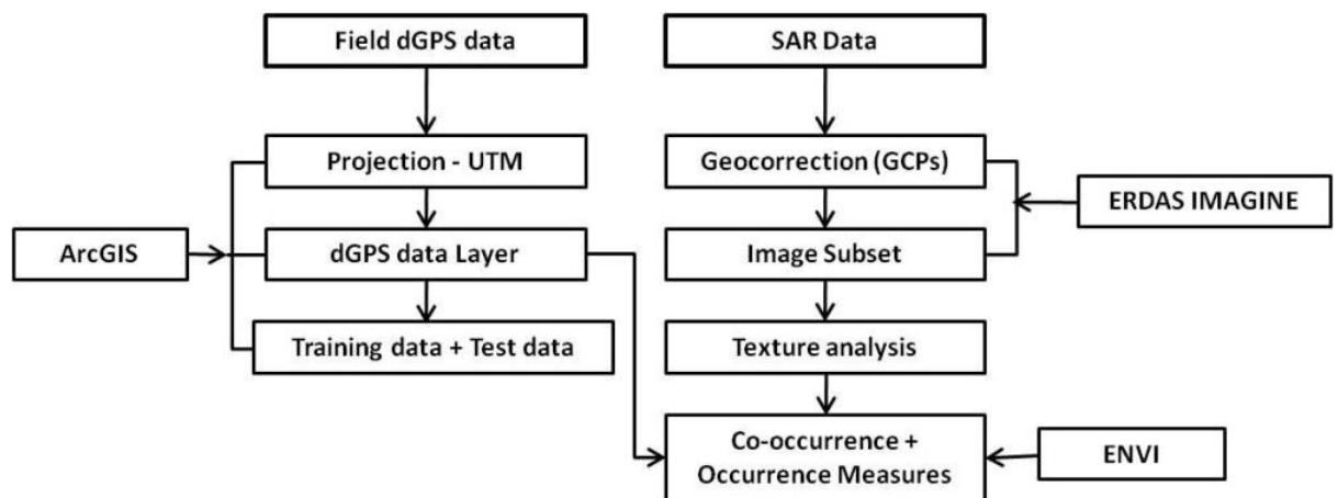
Figure 5.8: Methodology workflow of data preparation.
