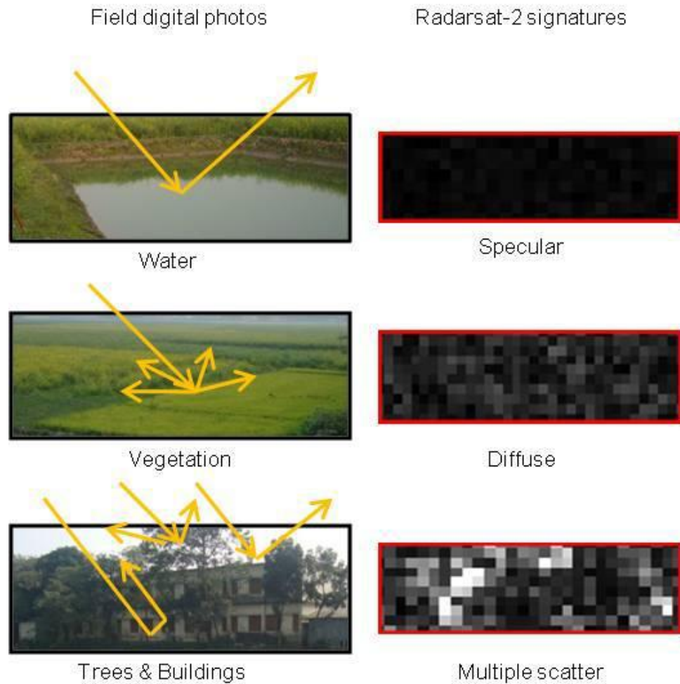
Figure 6.10: Imaging SAR sensor-HH polarization for various types of land cover compared to the field digital photos.
