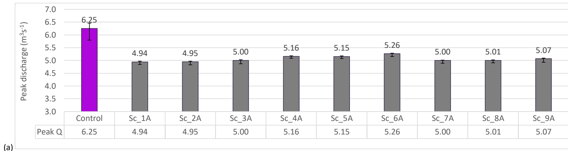
Figure 8.2 Graph of results of the nine combined flow restriction and attenuation scenarios amalgamated with the 25m deciduous woodland buffer.
