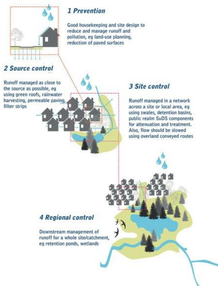
Figure 2.5 SuDS treatment train (Lead Local Flood Authorities of the South East of England, 2013).
