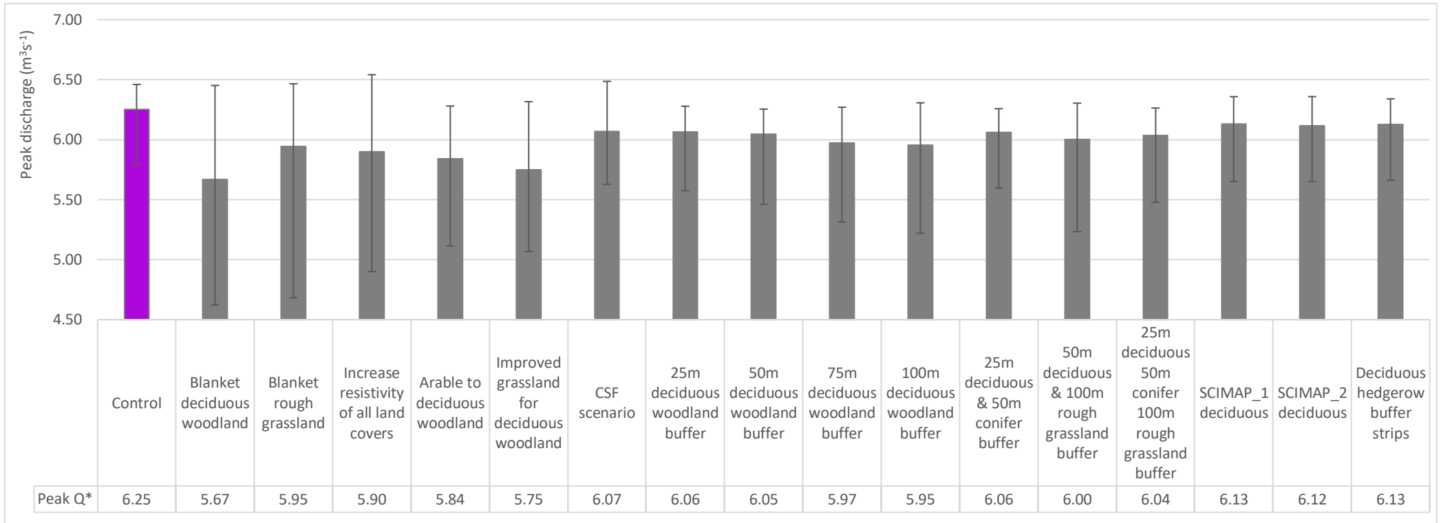
Figure 5.22 Graph showing results of all simulations that resulted in a measurable reduction in peak discharge (*Q measured in m³s⁻¹).
