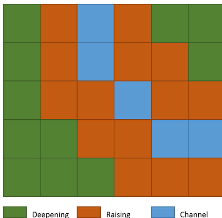
Figure 4.13 Restrictions on inserting attenuation across the catchment using the CRUM3 hydrological model.
