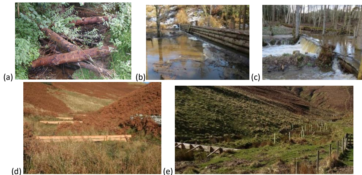
Figure 2.9 Images showing (a) flow disturbance at Hepscott in Northumberland (Royal Haskoning DHV, 2014); (b and c) timber bunds at Pickering Beck (Marrington, 2012); (d) timber barriers at Alwinton (Fraser et al., 2017); (e) timber barriers and willow planting at Alwinton (Fraser et al., 2017).
