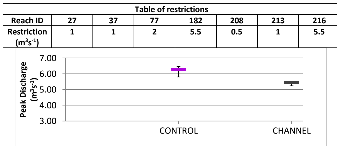
Figure 7.6 Graph showing results of channel gradient-driven flow restrictions according to table of restrictions above.
