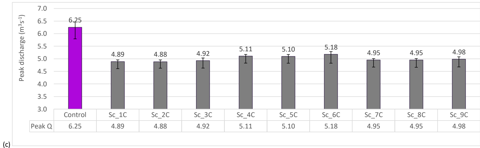
Figure 8.4 Graph showing results of the nine combined flow restriction and attenuation scenarios amalgamated with the change of arable land to deciduous woodland.
