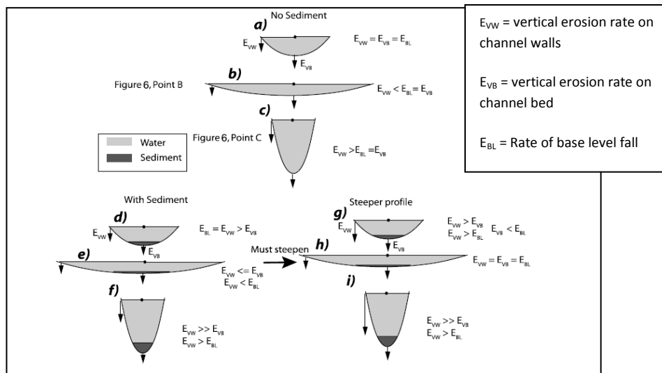
Figure 1.3. Source: Yanites and Tucker (2010). The presence of sediment can drastically alter the geomorphological response of bedrock channels to an imposed erosion rate.
