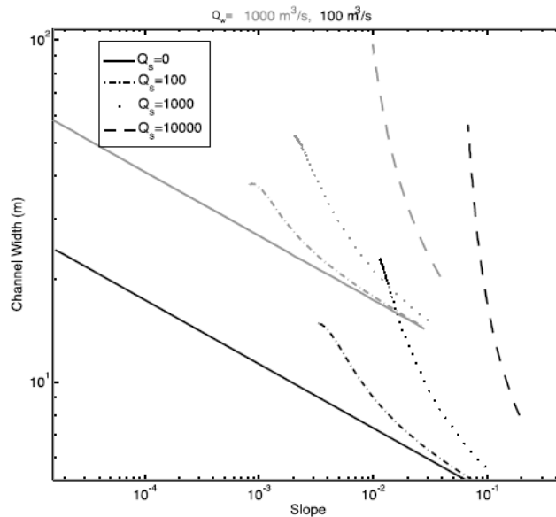
Figure 1.4. Relationship between channel width, slope and sediment supply ( Q_s ) shown for two different discharge values (source: Yanites and Tucker, 2010). As sediment supply increases, the relationship between slope and channel width steepens away from a linear scaling relationship as seen in sediment free channels and discussed by Finnegan et al. (2005).
