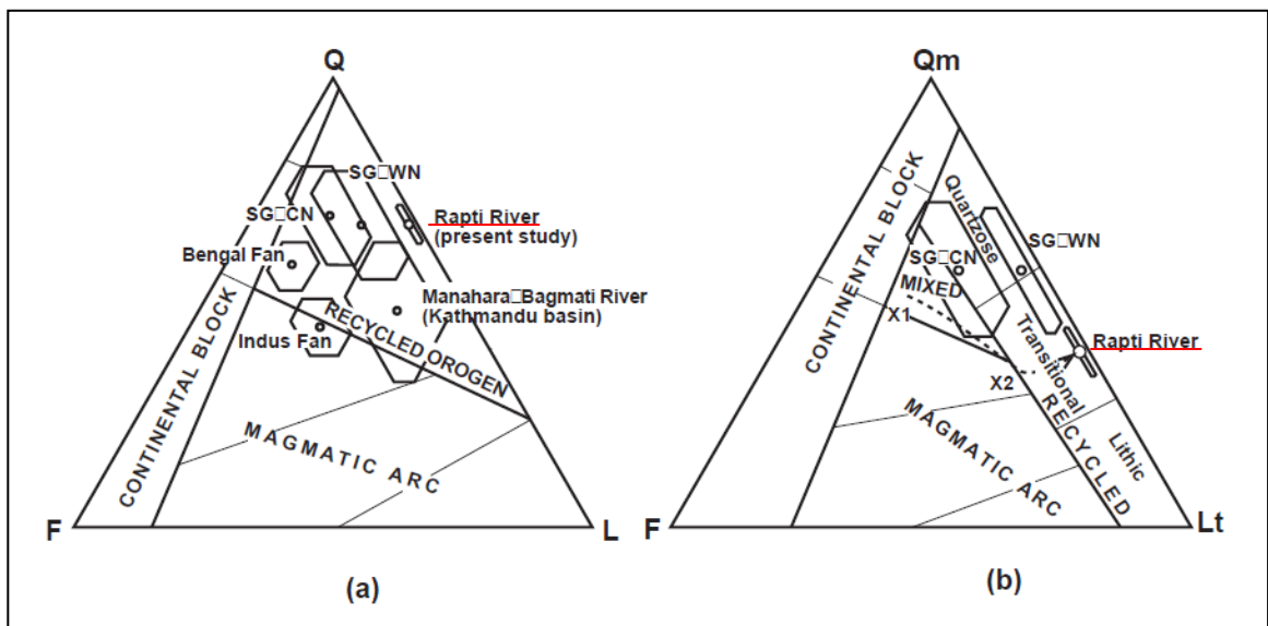
Figure 1.6. Recycled orogen provenance field plots displayed in an (a): Quartz ( Q ), Feldspar ( F ) and Lithic fragment ( L ) triangle diagram and (b): Monocrystalline quartz ( Q_m ), Feldspar and Lithic fragment + polycrystalline quartz ( L_t ) triangle diagram (source: Tamrakar et al., 2008). As can be seen in both triangle diagrams, the Rapti River sands are classified as from a recycled orogen provenance field with a high quarto-lithic composition. One explanation given to explain this high quartz content (and increase in quartz roundness further downstream) is the incorporation of recycled quartz derived from Siwalik and Dun deposits.
