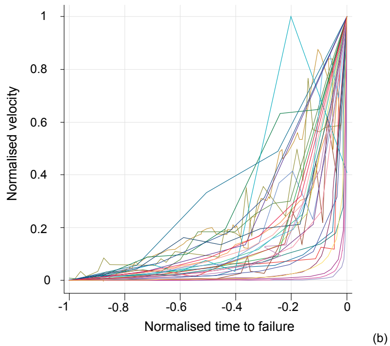
Figure 4.27: (a) Velocity-time data from the tertiary stage of creep. [Inset] Velocity-time data for failures whose maximum velocity is less than 5,000 mm/day; also excluding landslide ID 23. (b) Normalised velocity- normalised time data from the tertiary stage of creep
