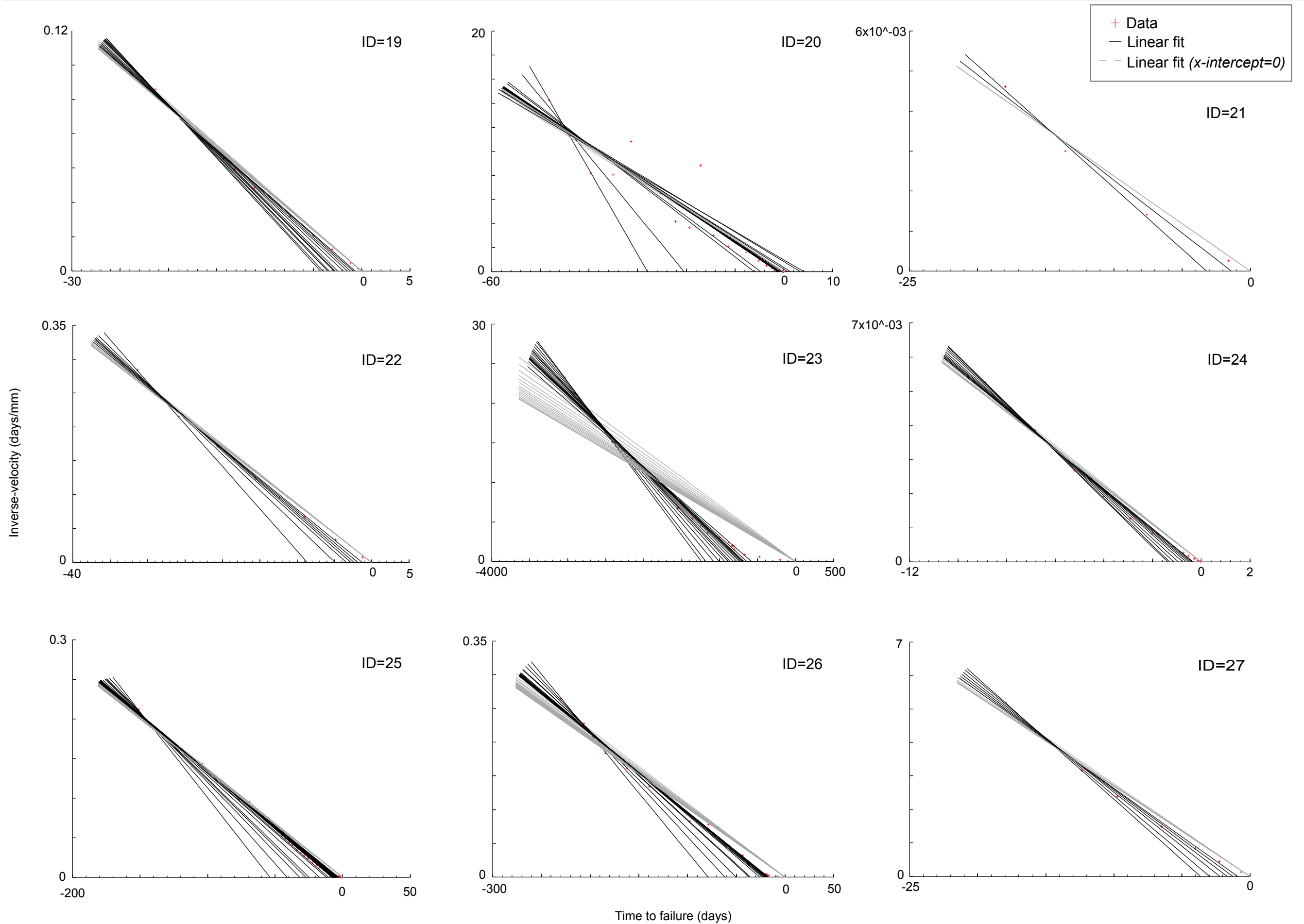
Figure 5.54:(c) Results from the iterative normal linear regression (grey corresponding to 'fixed' x-intercept) procedure carried out on inverse-velocity-time data. Landslide examples are presented on individual axes.
