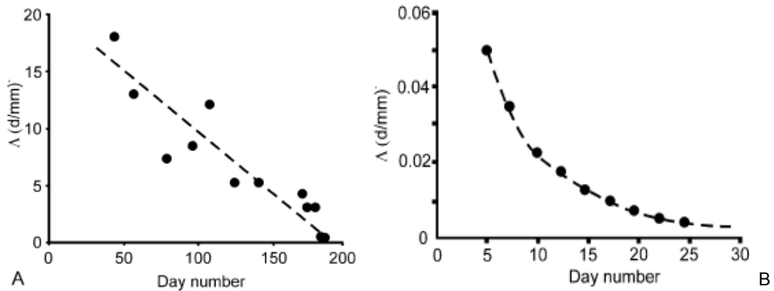
Figure 3.5: (A) Inverse-velocity-time trend for hillslopes undergoing brittle shear failure (Data from Inclinator 8, Selborne landslide, reproduced from figure 2A, Petley et al. (2002); p.720). (B) Inverse-velocity-time trend for hillslopes undergoing ductile deformation in the shear zone (Data from Abbotsford landslide, New Zealand, reproduced from figure 3B, Petley et al. (2002; p.721)).
