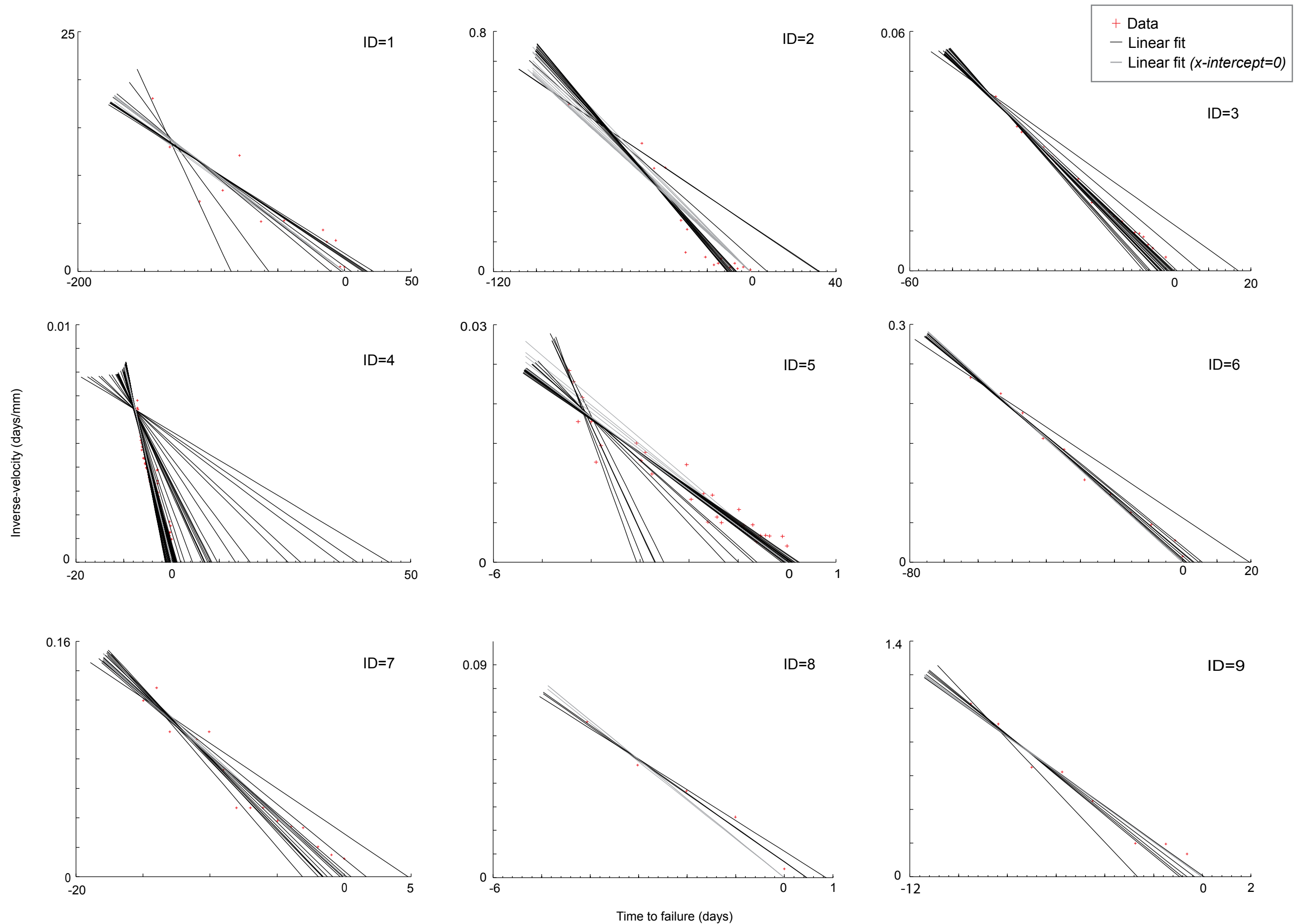
Figure 5.54:(a) Results from the iterative normal linear regression (grey corresponding to 'fixed' x-intercept) procedure carried out on inverse-velocity-time data. Landslide examples are presented on individual axes.
