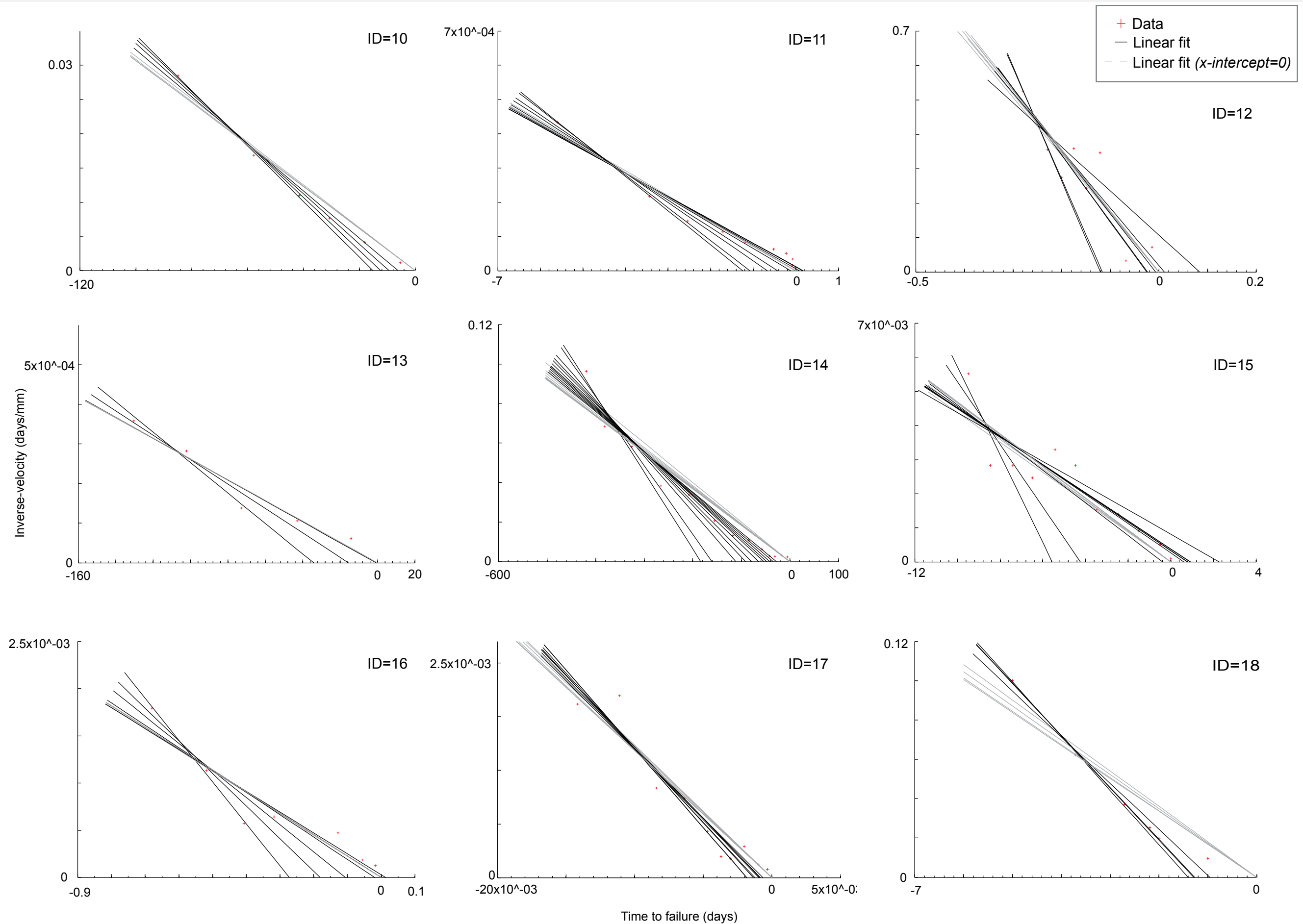
Figure 5.54:(b) Results from the iterative normal linear regression (grey corresponding to 'fixed' x-intercept) procedure carried out on inverse-velocity-time data. Landslide examples are presented on individual axes.
