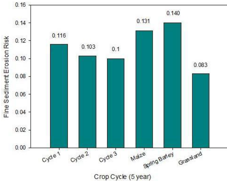
Figure 8.1: Annual average fine sediment erosion risk for various crop cycles within the River Eden catchment.
