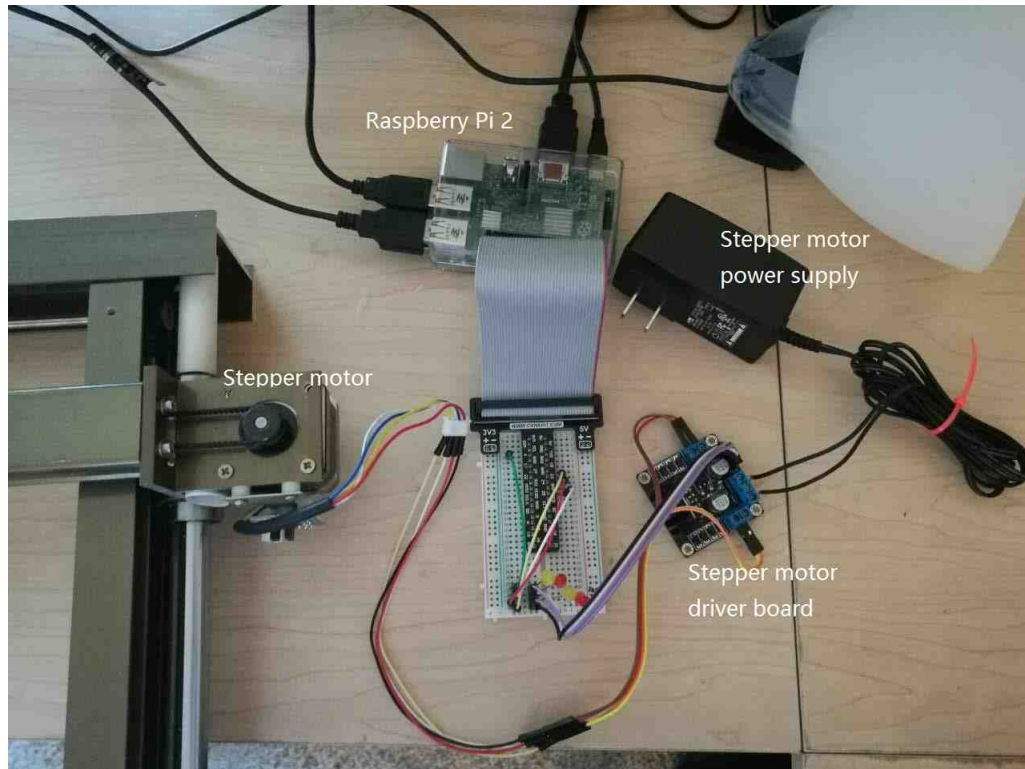
Fig. 5.2. Wire Connections
