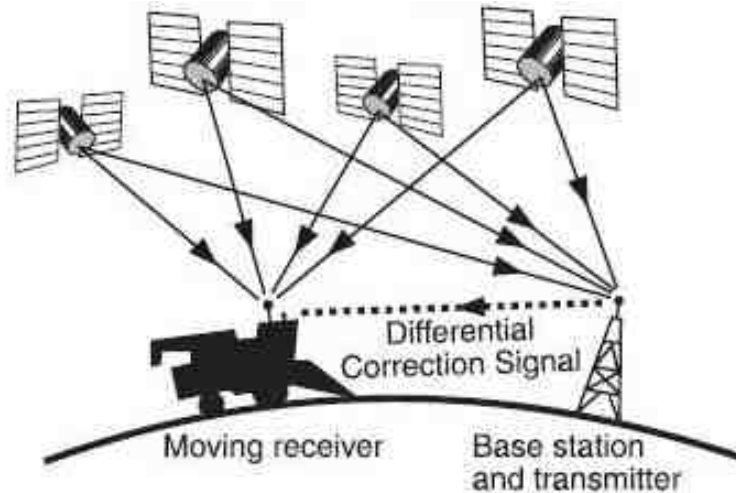
Fig. 2.1. Real-Time Differential GPS
