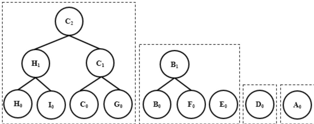
Fig. 5.4.: A receives C_2 from C , (B_1, B_0) from B , D_0 from D and generates A_0 . The received commitment forests are indicated by dashed-line box.
