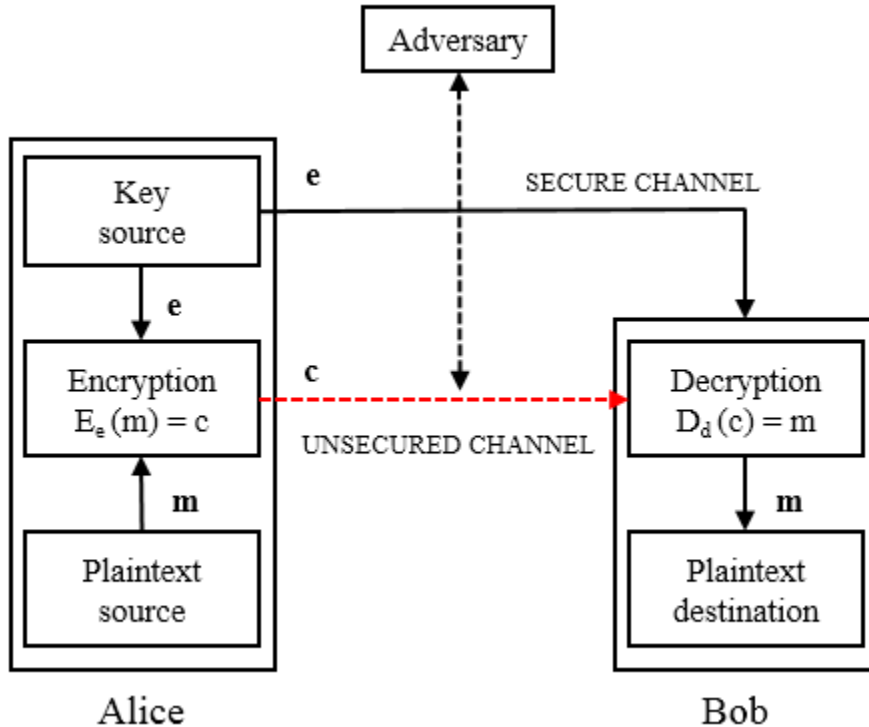
Fig. 3.1.: Two party communication using symmetric key encryption.
