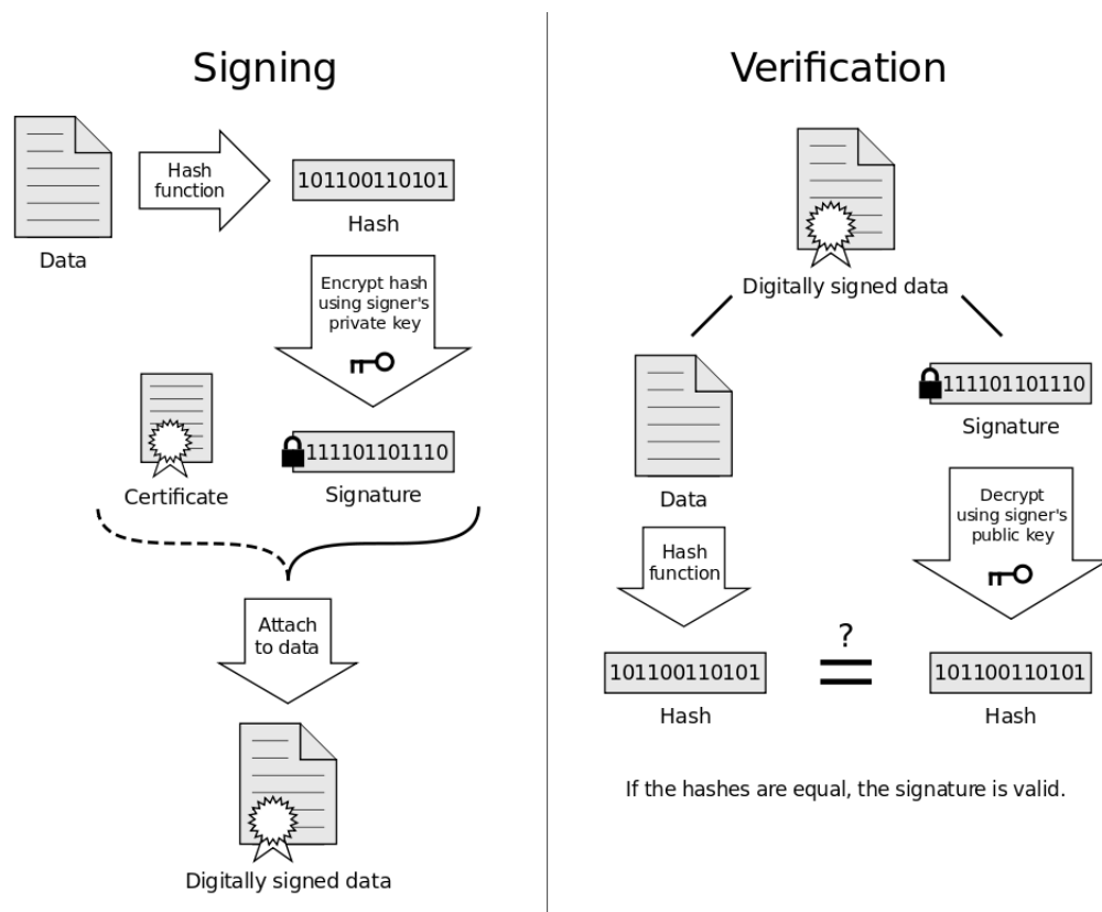
Fig. 3.3.: Signing and verification of digital Signatures [25]
