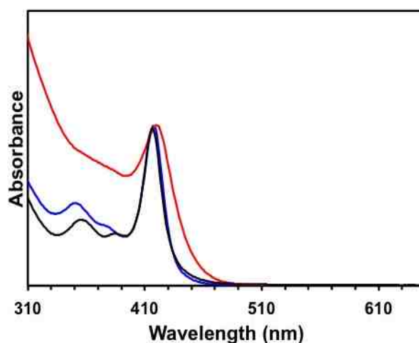
Figure 4.18 Room temperature steady-state (\text{CdSe})_{34} NC UV-visible absorption spectra of initial OLA-passivation (black curve), after \text{Et}_3\text{PAuCl} treatment forming mixed Py-/OLA-passivation (red curve), and after treatment with OLA (blue curve). The removal of Py-DTC from the surface of (\text{CdSe})_{34} NCs through \text{Et}_3\text{PAuCl} treatment produced partially OLA-passivated NCs.
