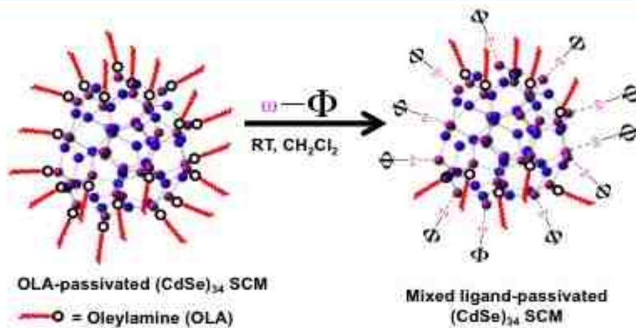
Figure 4.1 Schematic diagram depicting post-synthetic ligand exchange of OLA-passivated (CdSe) 34 NCs with a generic representation ( \omega - \Phi ) of the various ligands shown in Figure 1. The L-type ligand OLA preferentially binds with Cd sites. Purple and blue spheres represent Cd and Se atoms, respectively, of the (CdSe) 34 NC. The three-dimensional structure of the (CdSe) 34 NC does not correspond to the proposed core-cage structure reported in the literature. [5, 6] Red wavy lines are the aliphatic chain of OLA with the amine binding head group represented by black circles.
