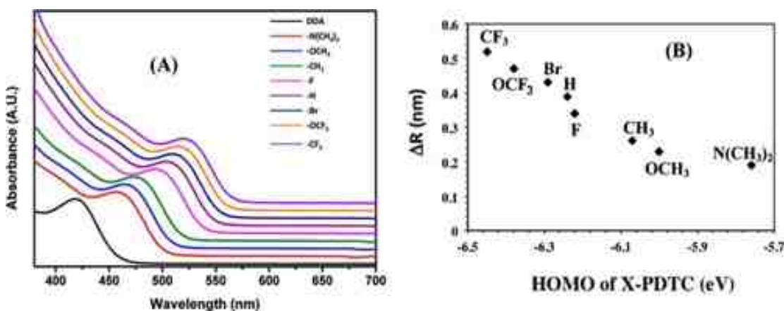
Figure 4.4. (A) Absorption spectra of various PDTC ligand-passivated 1.6 nm CdSe NCs. The spectra were taken at room temperature, and the NCs were dissolved in dichloromethane. (B) Plot of apparent increase in the excitonic radius ( \Delta R ) with respect to the HOMO energy of the PDTC ligand following (39) (see Table 4.1)
