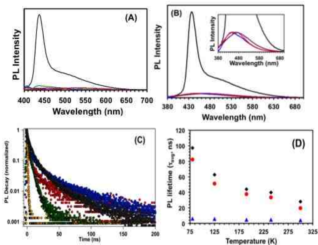
Figure 4.23 Room temperature steady-state PL spectra (in \text{CH}_2\text{Cl}_2 ) of various p-conjugated DTC type ligand-passivated (\text{CdSe})_{34} NCs: Ph-DTC (green line), Naph-DTC (blue line), Anth-DTC (red line), and Py-DTC (purple line). (B) Room temperature steady-state PL spectra of only OLA-passivated (black line), and mixed Ph-SH/OLA- (blue line), Ph-SeH/OLA- (red line), and Ph-TeH/OLA-passivated (purple line) (\text{CdSe})_{34} NCs in \text{CH}_2\text{Cl}_2 . The PL spectra were collected at 350 nm excitation energy. The inset shows an expanded region of the mixed Ph-EH/OLA-passivated (\text{CdSe})_{34} NCs. PL spectrum of original OLA-passivated NCs is shown by a black line in both panel (A) and (B). (C) Typical time-resolved PL traces measured at 300 K for different ligand-passivated (\text{CdSe})_{34} NCs: mixed Py-DTC/OLA- (blue dots), mixed Naph-DTC/OLA- (red dots), and mixed Ph-SH/OLA-passivated (green dots) NCs, and the original OLA-passivated NCs (black dots). All spectra were normalized to 1.0. The instrument response function (IRF, yellow dots) of this system was measured as 0.4 ns. (D) Temperature dependence of t_{\text{avg}} for Py-DTC/OLA- (black diamonds), Naph-DTC/OLA- (red dots), and Ph-SH/OLA-passivated (blue triangles) NCs.
