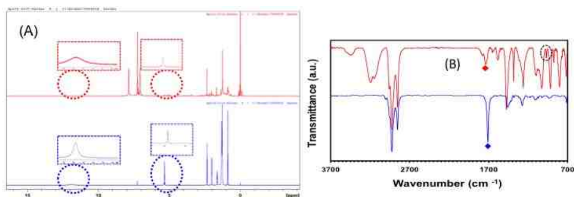
Figure 2.12 1 H NMR (A) and FTIR (B) characterization of pure oleic acid (blue) and \text{CH}_3\text{NH}_3\text{PbBr}_3 QWs (red).
