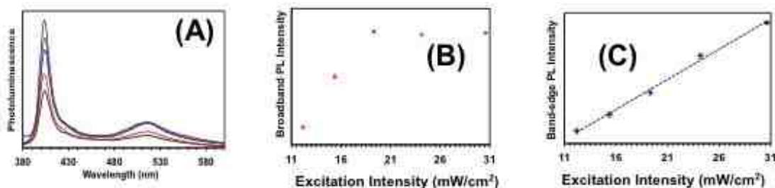
Figure 5.7 (A) PL spectra of \text{CH}_3\text{NH}_3\text{PbBr}_{3.8} NCs at different excitation power density ( \text{mW}/\text{cm}^2 ): black (11.2), red (15.4), blue (19.3), green (24.2), and purple (30.6). Dependence of broadband (B) and band-edge (C, R^2 =
