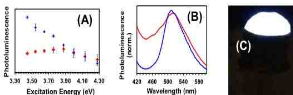
Figure 5.11 (A) Excitation wavelength dependent broadband PL intensity of \text{CH}_3\text{NH}_3\text{PbBr}_{3.8} (red) and \text{CH}_3\text{NH}_3\text{PbCl}_{1.3}\text{Br}_{2.5} (blue) NCs. (B) Comparison of broadband PL peak of \text{CH}_3\text{NH}_3\text{PbBr}_{3.8} (red) and \text{CH}_3\text{NH}_3\text{PbCl}_{1.3}\text{Br}_{2.5} (blue) NCs at 350 nm excitation. (C) A 5 mm commercial UV LED (360 nm) coated with \text{CH}_3\text{NH}_3\text{PbCl}_{1.3}\text{Br}_{2.5} NCs in polyurethane
