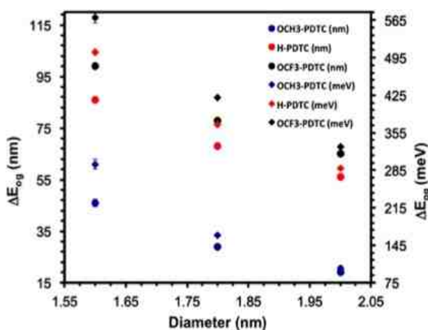
Figure 4.6. Comparison of change in the optical band gap and excitonic radius of various sized CdSe NCs passivated with CF_3O- , H- , and CH_3O- PDTC ligands.
