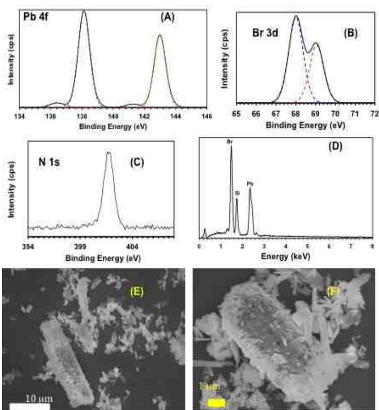
Figure 2.16 The XPS spectra (A-C) confirm the formation of \text{CH}_3\text{NH}_3\text{PbBr}_3 bulk material as determined from the appearance of shoulders in the Pb 4f spectrum. The Br 3d peak at 69.1 eV is lower in intensity than the peak at 68.0 eV, and together with the appearance of one nitrogen peak at 401.8 eV confirms the formation of \text{CH}_3\text{NH}_3\text{PbBr}_3 bulk material. The sample was also analyzed by EDX (D) and the atomic ratio of Pb-to-Br was found to be 1:2.9, whereas the ideal ratio of bulk \text{CH}_3\text{NH}_3\text{PbBr}_3 material should be 1:3. The SEM characterization (E-F) of the bulk \text{CH}_3\text{NH}_3\text{PbBr}_3 material showed the appearance of flake-type structure, which is aggregated.
