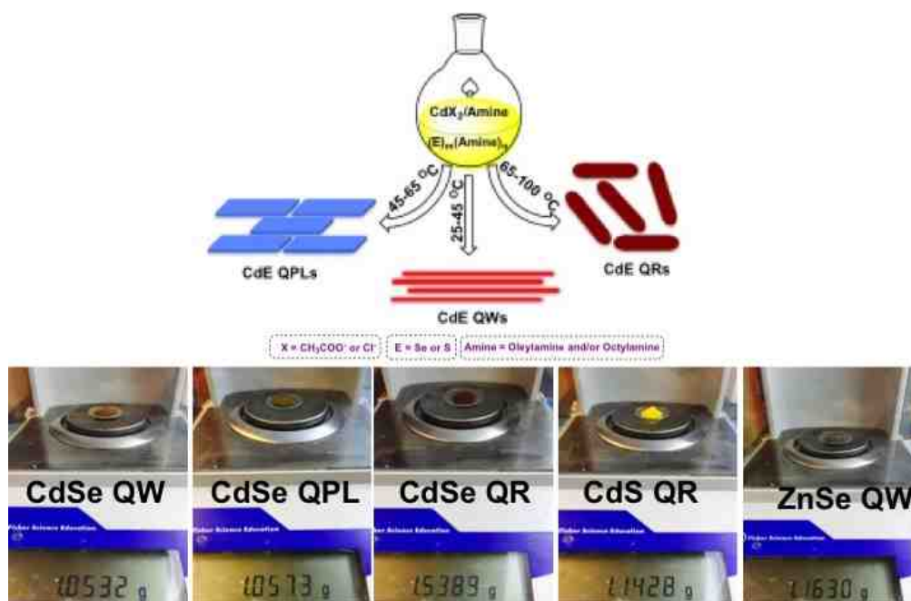
Figure 3.1. Depicts the synthetic route to produce metal chalcogenide QW, QPL, and QRs by varying surface ligand and temperatures and the gram scale yields of the for mentioned materials.
