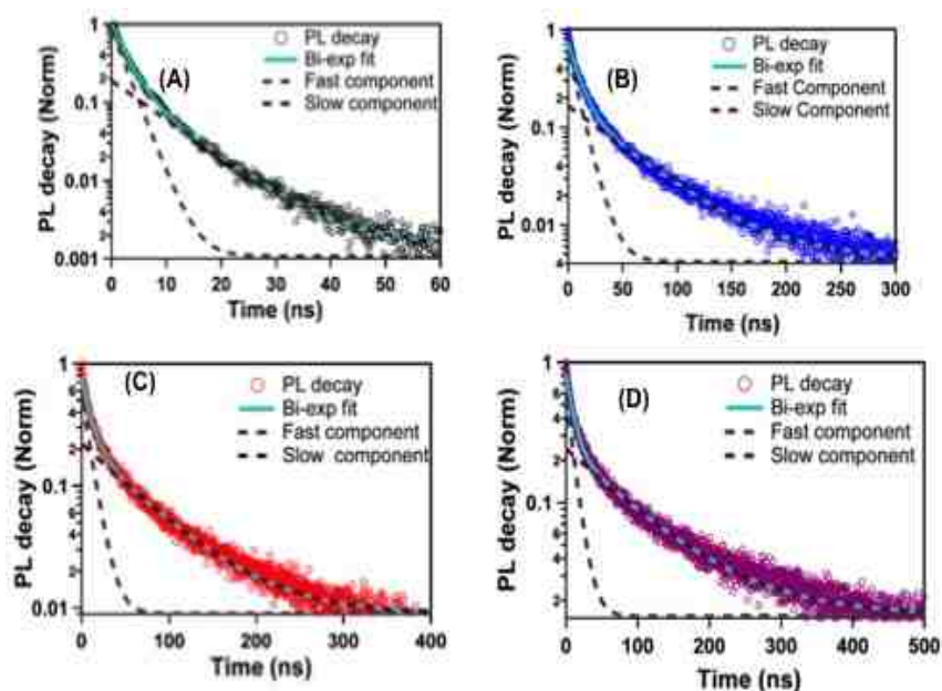
Figure 2.9 Normalized, biexponential fit of TCSPC spectra of reaction mixture at 30 (A), 60 (B), 120 (C), and 240 (D) sec. The time constant of the slow component ( t_{\text{slow}} ) is 9, 50, 63, and 89 ns at the four incubation time points.
