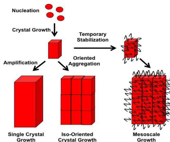
Figure 1.4. The three various mechanisms of shape control; classic crystal growth, oriented attachment, and mesoscale assembly. Based on figure in Colfen et al.[7]
