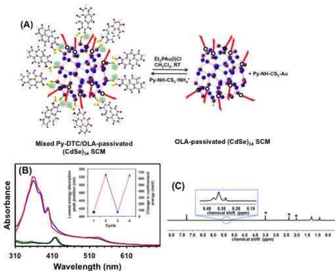
Figure 4.14 (A) Schematic diagram represents reversible ligand exchange of a mixed ligand-passivated NC with \text{Et}_3\text{PAuCl} . The negatively charged -\text{NH}-\text{CS}_2^- head group electrostatically interacts with surface Cd site similar to a dative type bond. Purple and blue spheres represent Cd and Se atoms, respectively, of (\text{CdSe})_{34} NC. Yellow and green spheres are S and N of -\text{NH}-\text{CS}_2 . Pink/light blue dots represent ammonium ion. (B) Steady-state absorption spectra of purified OLA-passivated (\text{CdSe})_{34} NCs after synthesis (black line), after Py-DTC treatment (mixed Py-DTC-/OLA- (\text{CdSe})_{34} NCs) (green line), after \text{Et}_3\text{PAuCl} treatment (partially OLA-passivated NCs) (red line), and after Py-DTC re-treatment (mixed Py-DTC-/OLA- (\text{CdSe})_{34} NCs) (blue line). The inset shows reversibility of the lowest energy absorption peak position of OLA-passivated (\text{CdSe})_{34} NCs (black dot), after repeatedly attaching Py-DTC (red triangles) and removing Py-DTC by \text{Et}_3\text{PAuCl} treatment (blue diamond). The details of the ligand treatment and removal are provided in the Materials and Method section. (C) ^1\text{H} NMR spectrum of \text{Et}_3\text{PAuCl} -treated and purified OLA-passivated (\text{CdSe})_{34} NCs. The expanded vinyl ( -\text{CH}=\text{CH}- ) resonance of OLA is shown in the dotted blue box. The asterisks represent signal from residual solvent. The spectrum was collected in \text{CDCl}_3 at a 15 s relaxation delay time.
