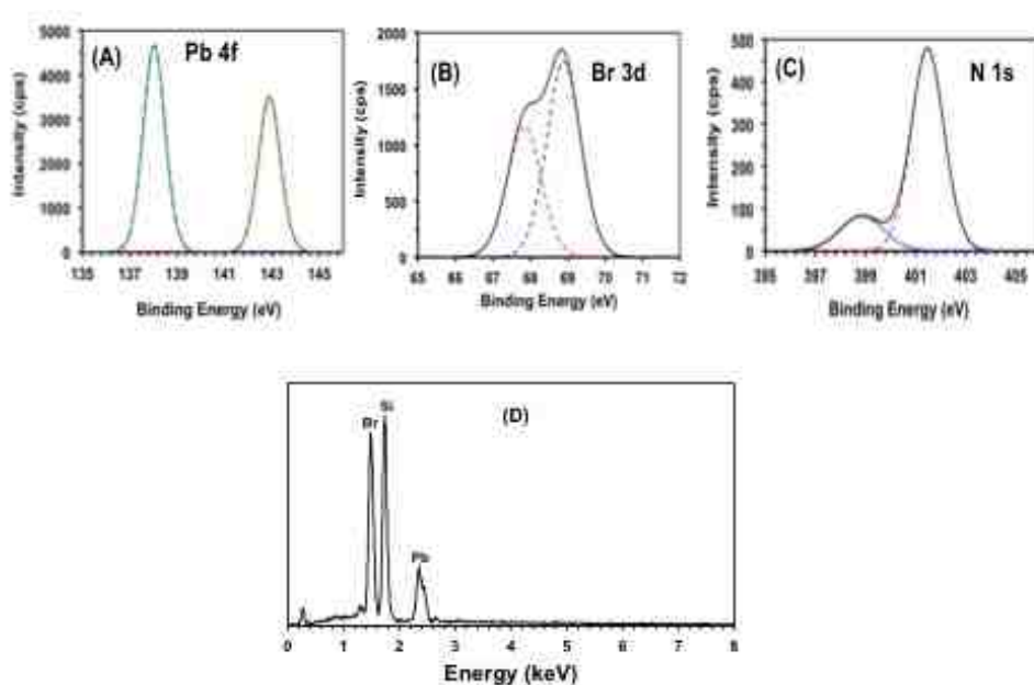
Figure 2.11 X-ray photoelectron spectroscopic (XPS) analysis of \text{CH}_3\text{NH}_3\text{PbBr}_3 QWs. The Pb 4f (A), Br 3d (B), and N 1s (C) spectral profile of the \text{CH}_3\text{NH}_3\text{PbBr}_3 QWs. The solid lines are the experimental data and dotted lines are the fits. (D) A representative energy dispersive X-ray (EDS) spectroscopy analysis of \text{CH}_3\text{NH}_3\text{PbBr}_3 QWs.
