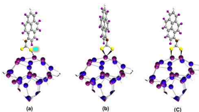
Figure 4.15 Proposed mode of binding of Py-DTC ligand to surface Cd sites of a (\text{CdSe})_{34} NC. Purple and blue spheres represent Cd and Se atoms, respectively. Dative ion-pair (A), chelating (B), and bidentate bridging (C) interactions. The pink/light blue dot represents ammonium ion and the sulfur from -\text{NH}-\text{CS}_2 is shown as yellow spheres.
