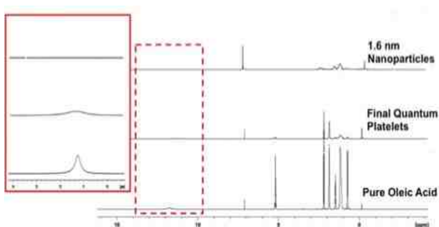
Figure 2.26 ^1\text{H} NMR analysis was performed on both the 1.6 nm diameter nanocrystals obtained at 5 s (top) and the final quantum platelets (middle). Pure oleic acid (bottom) was used as a reference for the peak positions
