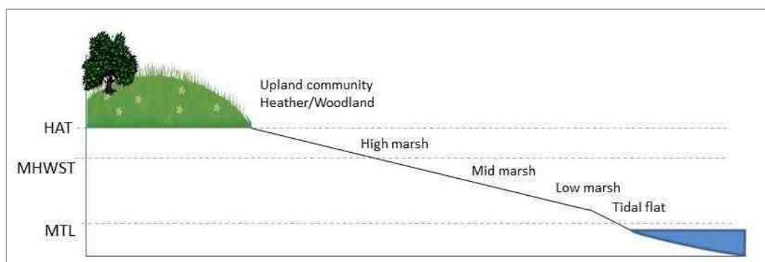
Figure 2.1: Schematic diagram of a salt-marsh environment showing zonation and reference water levels. (HAT – Highest Astronomical Tide, MHWST – Mean High Water Spring Tides, MTL – Mean Tide Level)
