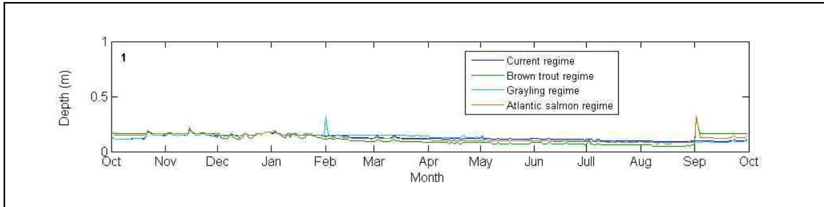
Figure 6.24 Depths produced during the water year 2002-2003 when the current, brown trout, grayling and Atlantic salmon regimes were applied to HEC-RAS, site 1
