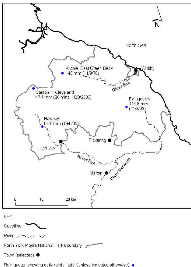
Figure 4.5. Recorded extreme rainfall events in the North York Moors area. Diagram contains Ordnance Survey Strategi® data: © Crown Copyright/database right 2011. An Ordnance Survey/EDINA supplied service. Rainfall data sources: Met Office MIDAS database and Cinderey (2003) for Carlton-in-Cleveland rainfall.
