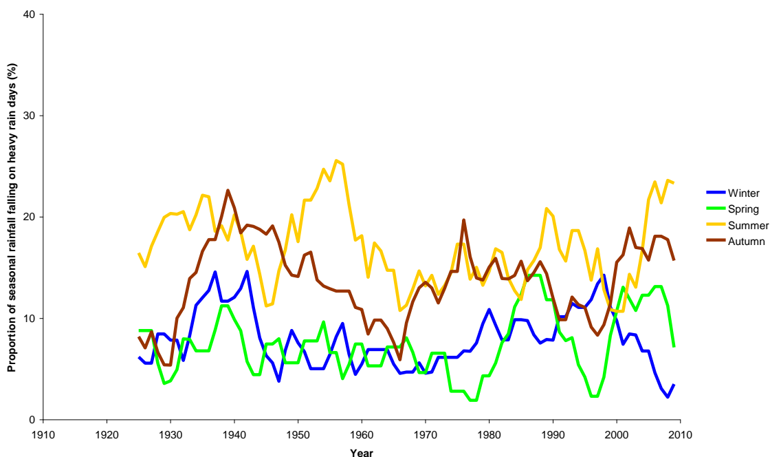
Figure 4.7: Changes in the proportion of seasonal rainfall falling on heavy rain days for winter, spring, summer and autumn, upper Ryedale, 1916-2009. Heavy rain days defined using the DR1 threshold. Lines show ten year running means. Rainfall series formed from data contained in the Met Office MIDAS database.
