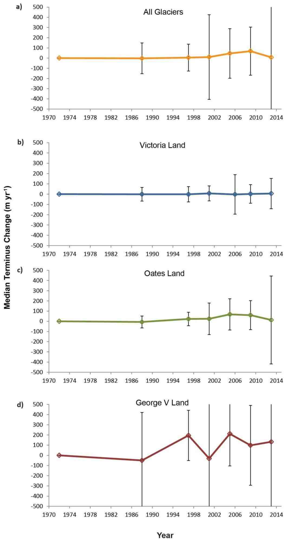
Figure 5.2: Median terminus change (m yr -1 ) per epoch for a) the whole study area, b) Victoria Land, c) Oates Land and d) George V Land. 1 standard deviation error bars are shown as black lines. Note that some error bars extend beyond the graph.
