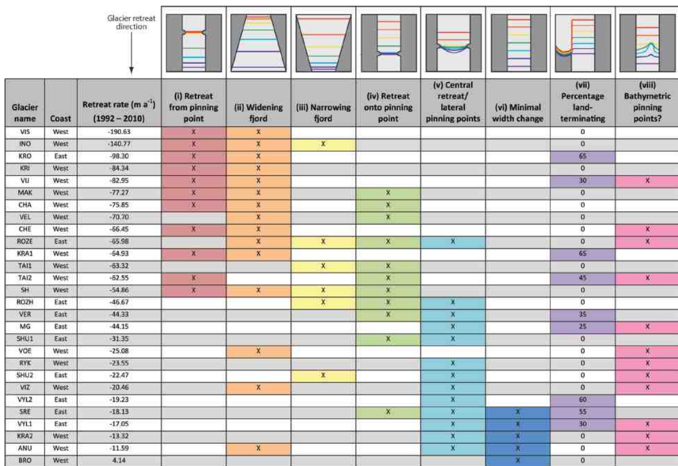
Figure 2.6: Fjord width change categorisation proposed by (Carr et al., 2014) relative to the 1992-2010 glacier retreat rate (from highest to lowest) of retreating glaciers in Novaya Zemlya in the Russian Arctic. Each column represents an idealised retreat of glacier terminus position in relation to variations in fjord width. Each row shows the retreat rate of an actual glacier (from highest retreat rate to lowest) and an ‘x’ marks the types of width variation observed during the glacier’s retreat. Column vii includes the percentage of the glacier that that is land-terminating.
