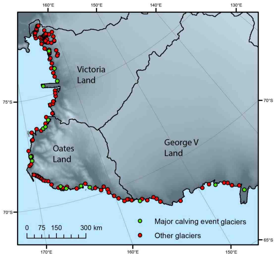
Figure 5.18: The location of the marine-terminating glaciers that experienced major calving events during the study time period.
