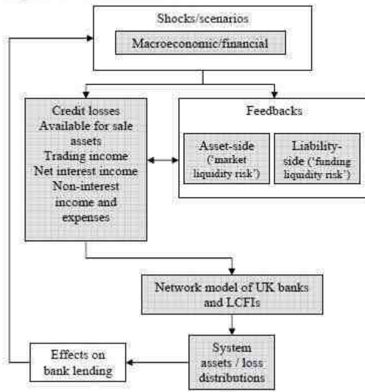
Figure 1: RAMSI framework
