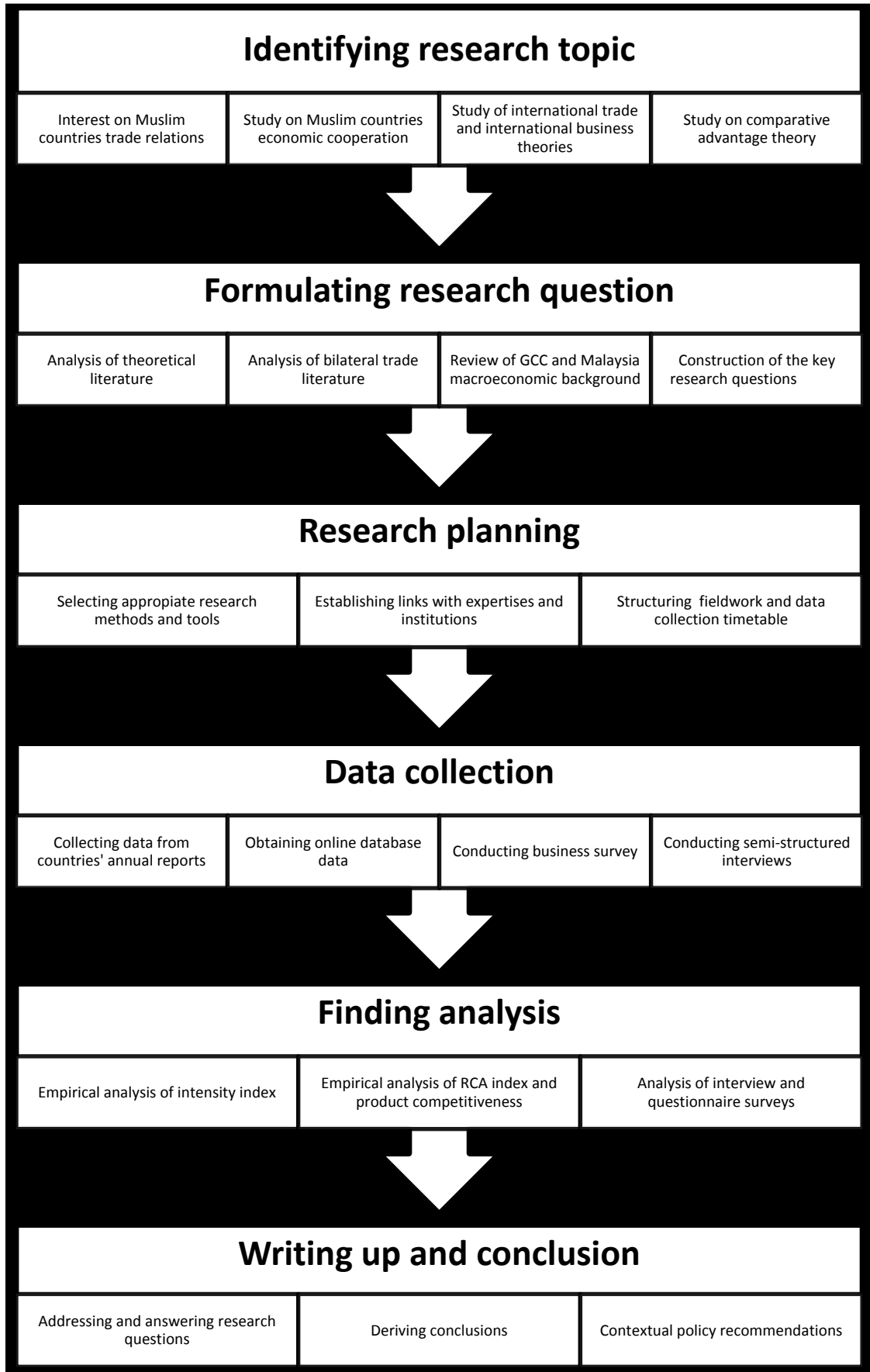
Figure 5-1: Research process
