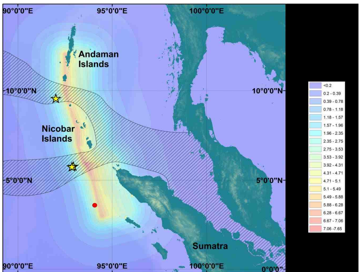
Figure 3.7 ShakeMap generated by the USGS for the Boxing Day 2004 Earthquake. Sumatra, the Nicobar and Andaman Islands, and Thailand are shown with submarine cable breaks denoted by yellow stars. Red dot represents earthquake epicentre. Hatch shading denotes the areas covered by submarine cables.
