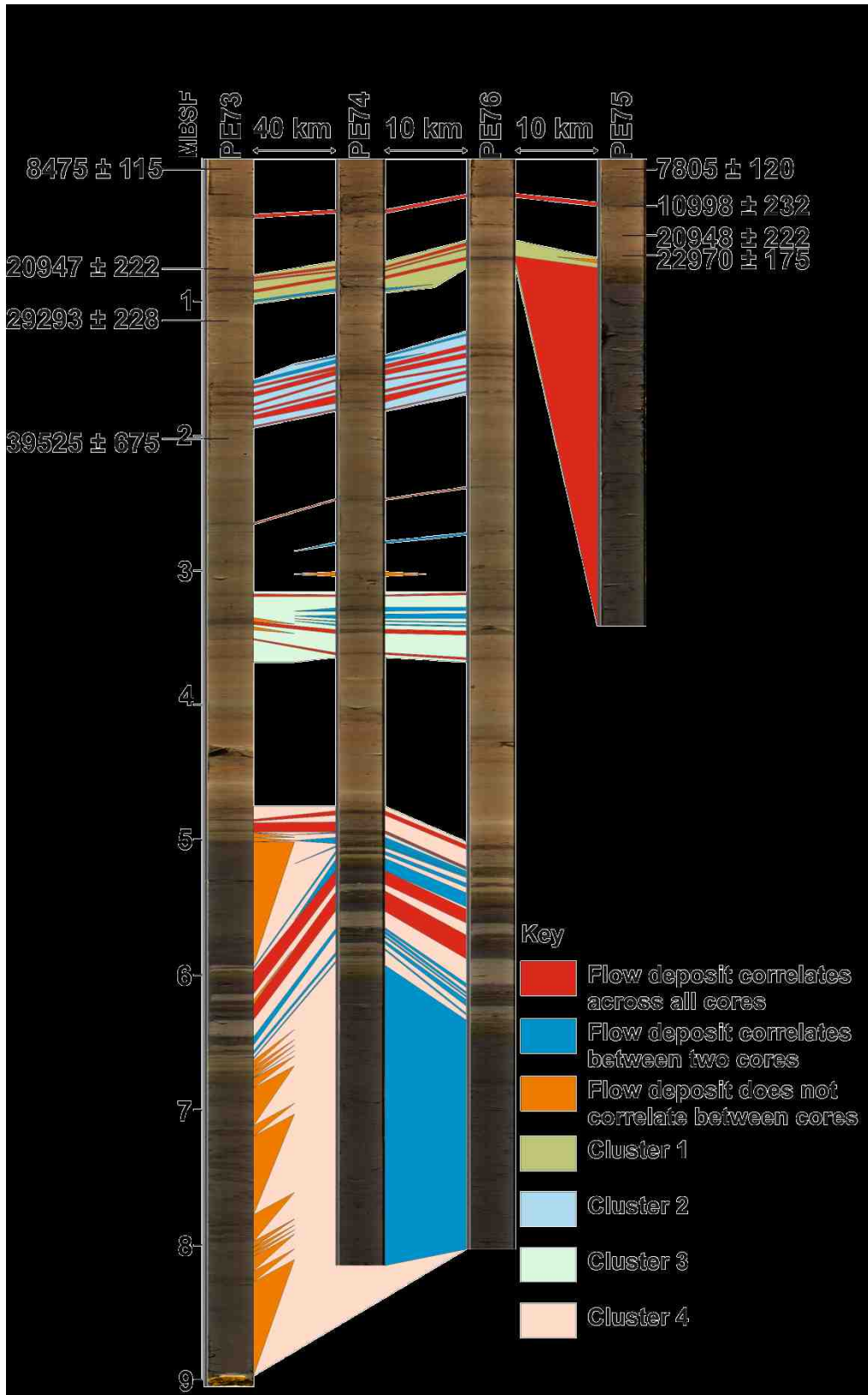
Figure 5.7 Core correlations between cores PE73, PE74, PE75 and PE76. Distances between the cores and radiocarbon dates from cores PE73 and PE75 are shown. MBSF = Meters Below Sea Floor. Four clusters of distal debris-flow muds correlate well across the three long cores. Few deposits from glacigenic debris-flows occur outside of these main clusters.
