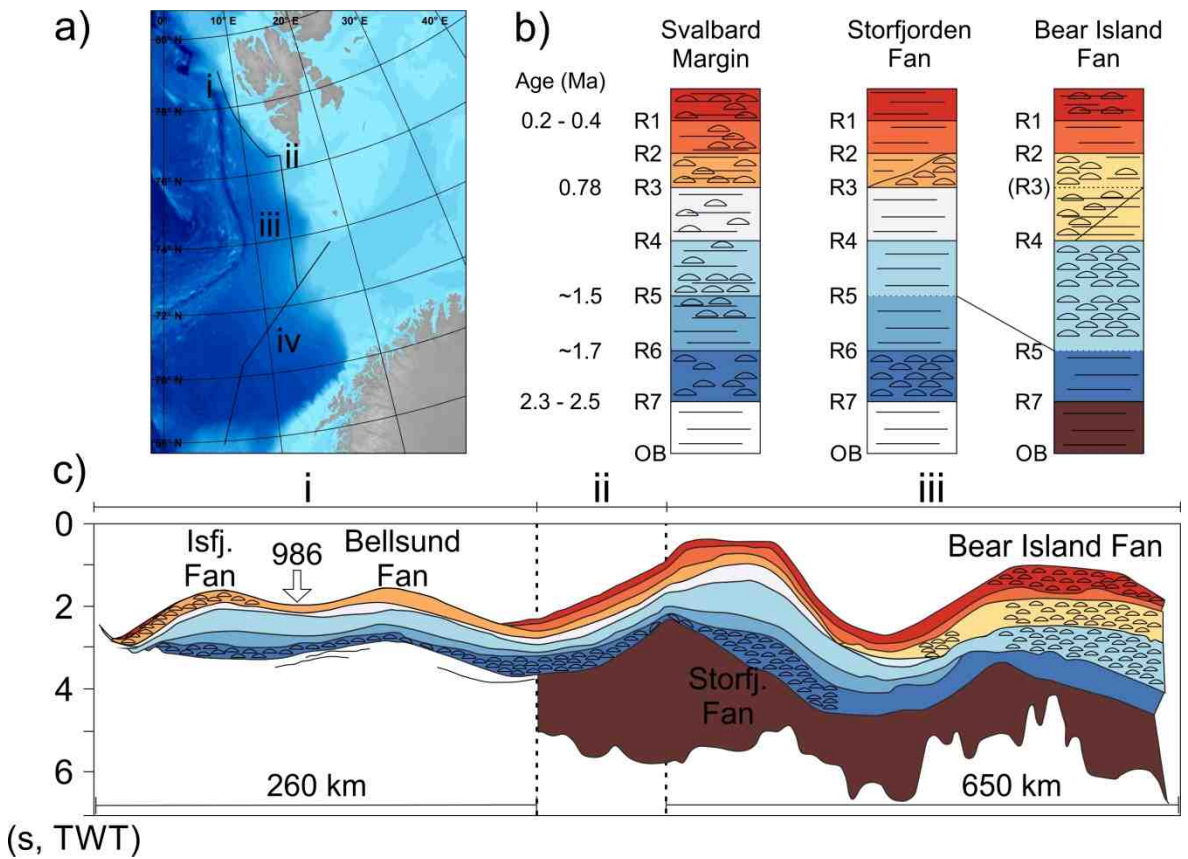
Figure 6.8 a) Location map of seismic profiles along the Svalbard/Barents Sea continental margin. b) Seismic stratigraphic framework for the Svalbard/Barents Sea Margin, with correlation of the main sequence boundaries between the Svalbard Margin (Isfjorden), Storfjorden and Bear Island Trough-Mouth Fans. Internal reflection pattern in b) and c) is indicated with changes between stratified (parallel lines) and chaotic with mass movement structures (half circle pattern). Regional reflectors based on chronology from ODP Site 986 are indicated. Modified from Faleide et al. (1996), Jansen et al. (1996) and Solheim et al. (1998).
