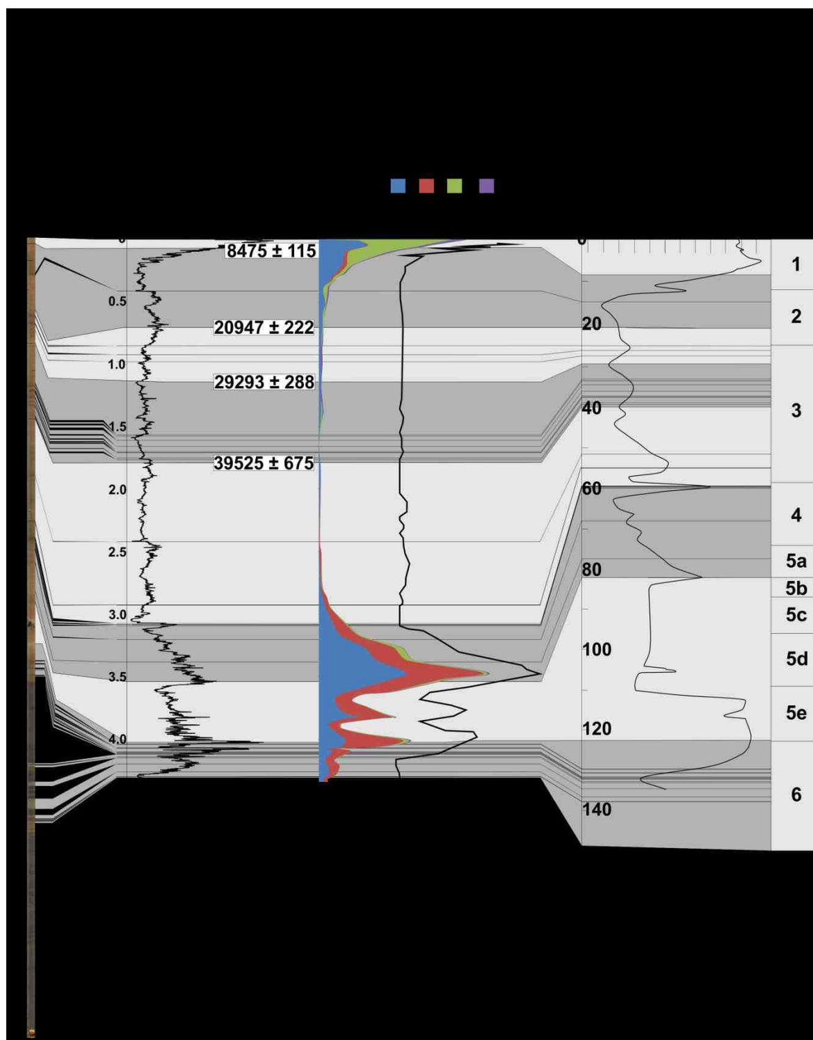
Figure 5.8 Core panel for PE73 showing hemipelagic ITRAX Ca profile. Radiocarbon dates are initially used to correlate the core record with a local benthic \delta^{18}\text{O} curve from core V27-60 offshore of the Bear Island Trough-Mouth Fan (Labeyrie and Duplessy, 1985). Beyond the range of radiocarbon dating, the ITRAX Ca profile is correlated with the \delta^{18}\text{O} curve. Coccolithophore counts from toothpick hemipelagic samples are shown to corroborate the proxy dating using the ITRAX Ca profile based on the coccolith abundance curve from Backman et al. (2009) which was obtained from core V27-60.
