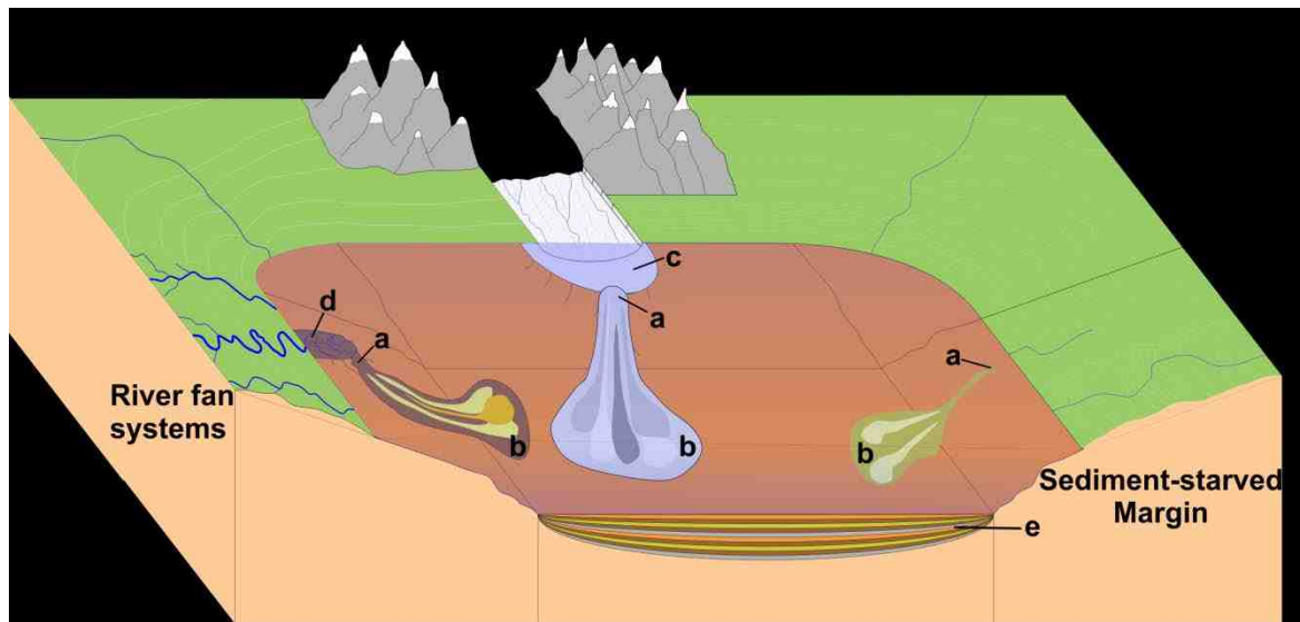
Figure 2.5 Three separate sedimentary systems feeding into one ocean basin. Each system is likely to have different characteristic landslide recurrence intervals due to different local environmental factors. River-fan systems experience the highest sediment input during deglaciation or lowstands, depending on latitude, as rivers efficiently transport terrestrial sediment (Covault and Graham, 2010; Urlaub et al., 2013). Glaciated margins are strongly influenced by climatic cycles due to the direct influence of growing and shrinking ice sheets and the position of ice streams (Lee, 2009) in terms of both local sea level and the location and timing of sediment delivery (Dowdeswell et al., 1996). Sediment starved margins are characterised by lower sediment deposition rates as they have not been affected by glaciation and are located away from major river-fan systems. Labels (a) landslide headscarp, (b) landslide deposits, (c) trough-mouth fans, (d) river-fan deltas, (e) interbedded sequence of background hemipelagic and sediment density flow deposits.
