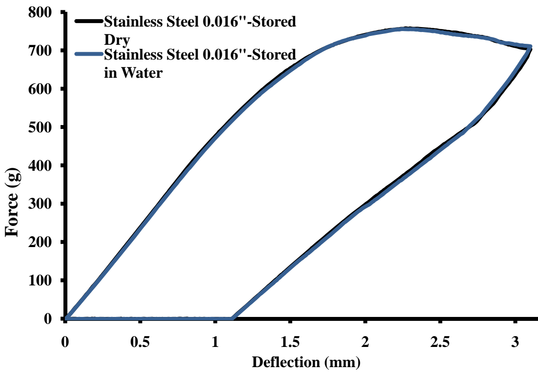
Figure 13. Graph example of force-deflection curve for stainless steel 0.016 inch.
