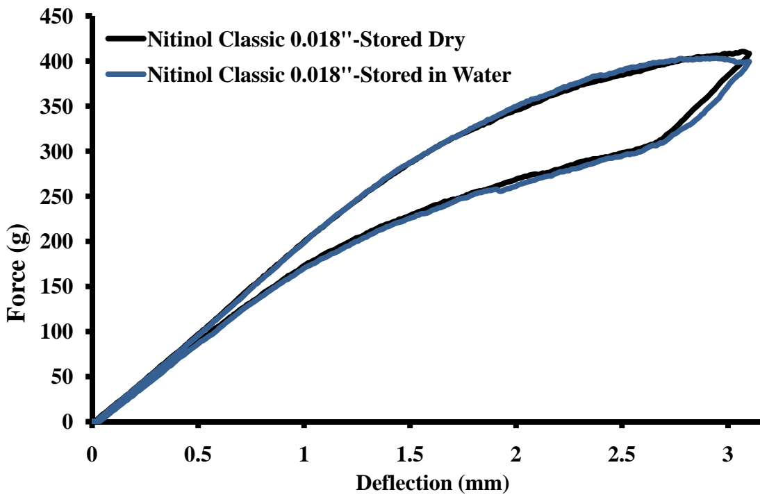
Figure 12. Graph example of force-deflection curve for Nitinol Classic 0.018 inch.
