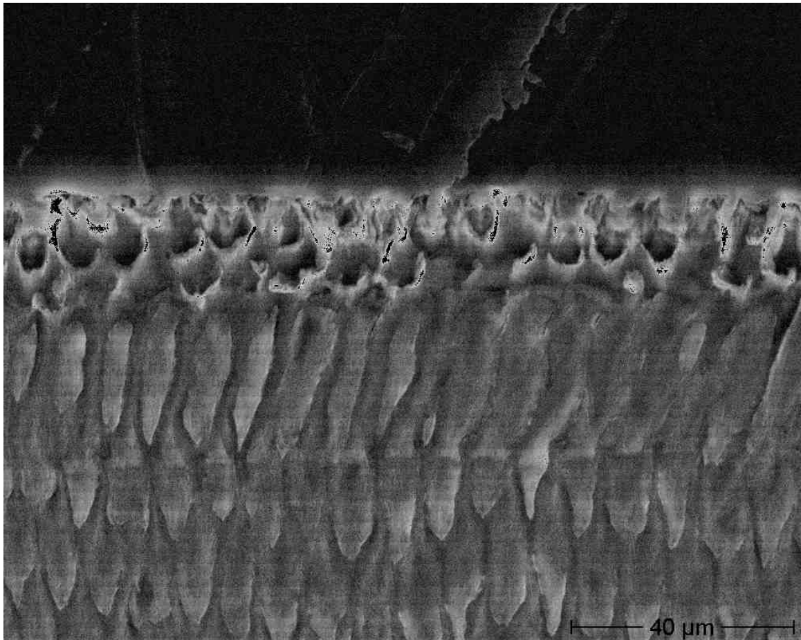
Figure 13. Cross-section after Pre-etching and SEP (Scanning Electron Microscopy)
