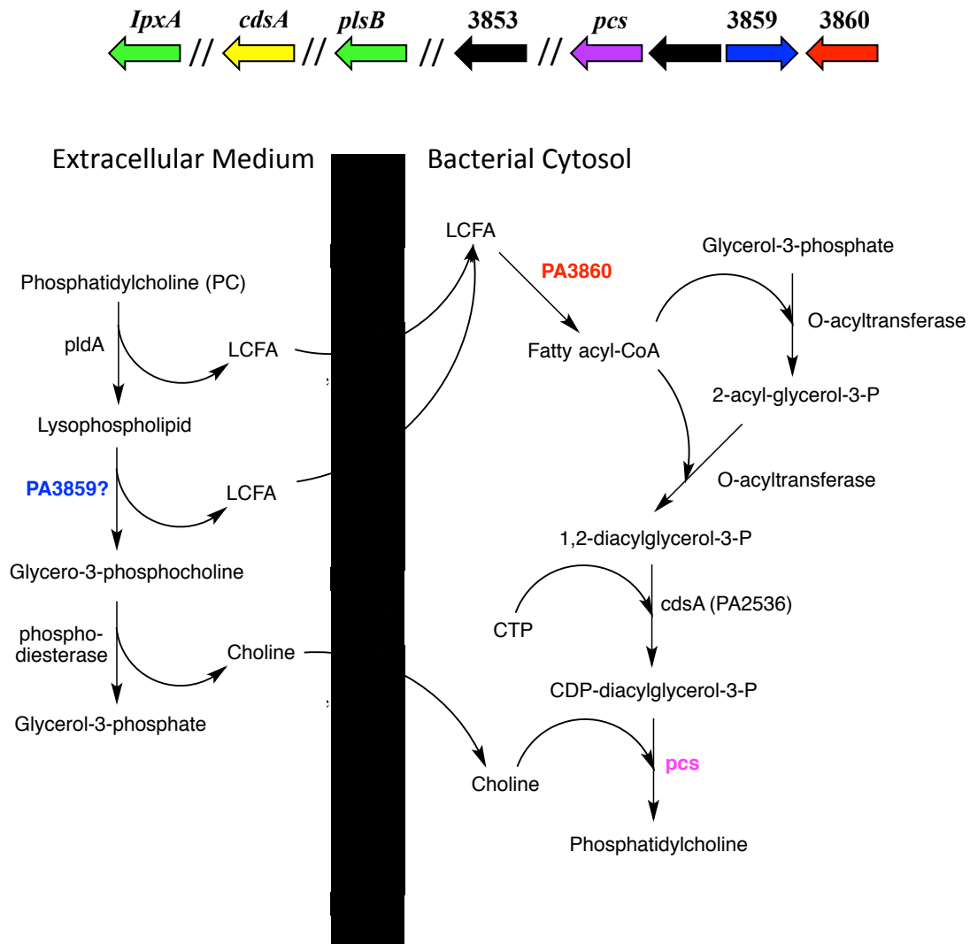
Figure 3-7. Potential PA3860 involvement in phosphatidylcholine (PC) synthesis. Gene context shows proximity of PA3860 to pcs , PA3859 (carboxylesterase), PA3853 (putative acyltransferase), and downstream genes involved in PC synthesis.
