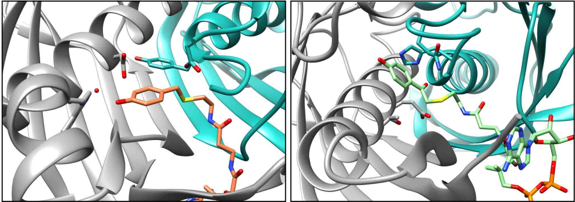
Figure 1-5. Active site scaffolds of 4-HBT-I from Pseudomonas sp. CBS-3 (PDB: 1LO8) (left) and 4-HBT-II from Arthrobacter sp. Strain SU (PDB: 3R3F) (right). Active sites are positioned at the dimer interface. Monomer units are colored separately. 4-hydroxybenzoyl-CoA substrate analog inhibitors are colored in orange and green.
