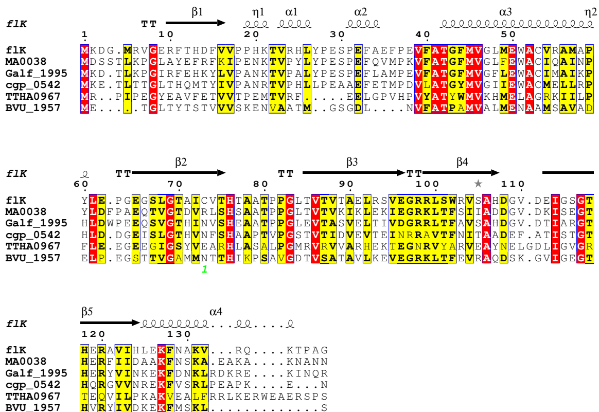
Figure 2-11. Multiple alignment of f1K and cloned f1K -orthologs. Completely conserved residues are highlighted in red and highly conserved residues are highlighted in yellow. Secondary structure was overlaid using the f1K crystal structure (PDB: 3KV8_B).
