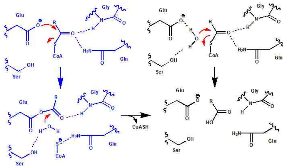
Figure 3.3: Possible catalytic mechanisms (nucleophilic catalysis [blue] or base catalysis [black]) for YdiI and YdbB.
