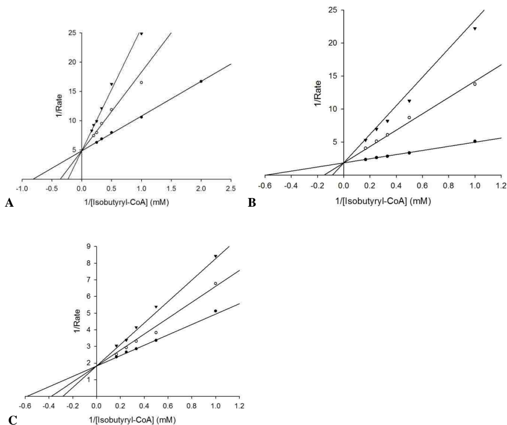
Figure 5.4: A - Competitive inhibition plots for \beta -ketopropanone- holo ACP monitored by DTNB assay using 0.16 \mu\text{M} E. coli YbgC, 0.5-6 mM isobutyryl-CoA, and 0 ( \bullet ), 10 (o), or 20 ( \blacktriangledown ) \mu\text{M} inhibitor. B - Competitive inhibition plots for \beta -ketopropanone-CoA monitored by DTNB assay using 0.22 \mu\text{M} E. coli YbgC, 1-6 mM isobutyryl-CoA, and 0 ( \bullet ), 250 (o), or 500 ( \blacktriangledown ) \mu\text{M} inhibitor. C - Competitive inhibition plots for apo -ACP
