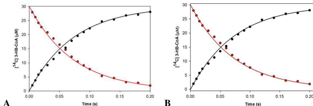
Figure 6.5: Experimental and simulated time courses for the single turnover reaction containing 50 \mu\text{M} wild type BH1999 and 30 \mu\text{M} [ ^{14}\text{C} ]3-HB-CoA in 50 mM \text{K}^+\text{HEPES} (pH 7.5, 25 ^\circ\text{C} ). The time point data [ ^{14}\text{C} ]3-HB-CoA (●) and [ ^{14}\text{C} ]3-hydroxybenzoic acid (●) were calculated from the fraction of [ ^{14}\text{C} ] 3-HB-CoA and [ ^{14}\text{C} ] 3-hydroxybenzoic acid present in the acid quenched reaction. (A) The simulated curves were generated using the kinetic model in Scheme 6.1 using the rate constants k_1 = 160
