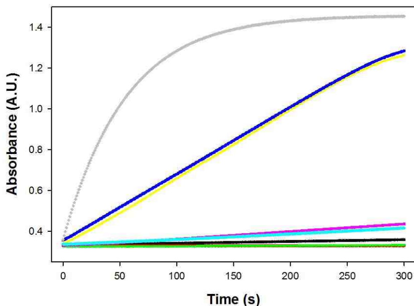
Figure 6.7. All reaction solutions contained 1 mM DTNB in 50 mM K + HEPES (pH 7.5, 25 °C). Test Reactions: (—) 70 \mu M 3-HB-CoA and 0.07 \mu M BH1999; (—, —) 70 \mu M 3-HB-CoA, 100 mM hydroxylamine, and 0.07 \mu M BH1999; Control Reactions: (—) 70 \mu M 3-HB-CoA and 0.07 \mu M BH1999 preincubated with 100 mM hydroxylamine; (—) 70 \mu M CoA and 100 mM hydroxylamine; (—) 70 \mu M 3-HB-CoA; (—) 100 mM hydroxylamine; (—) 70 \mu M 3-HB-CoA and 100 mM hydroxylamine.
