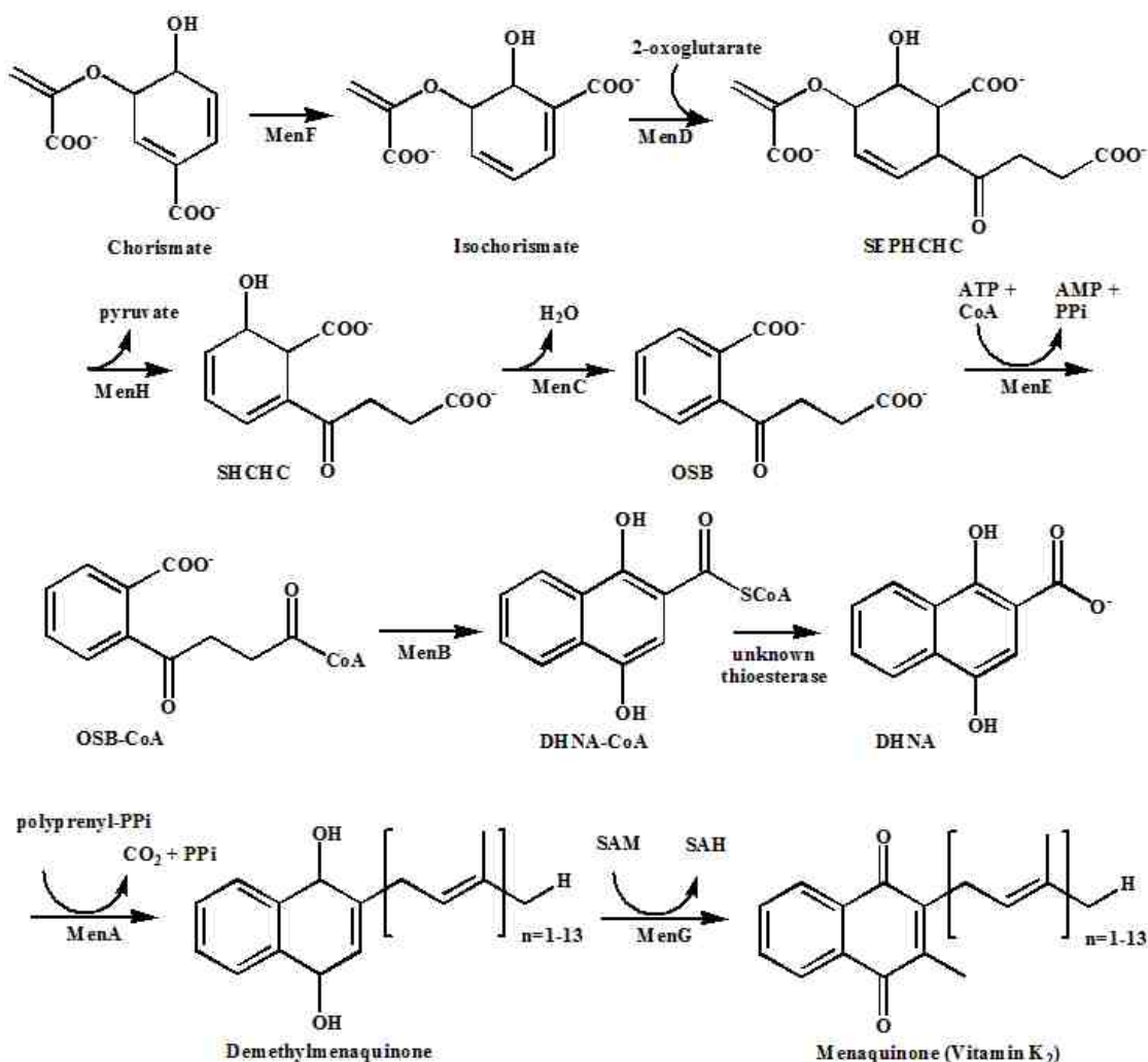
Figure 2.1. The menaquinone biosynthetic pathway in E. coli . The pathway enzymes are: isochorisimate synthase, MenF; SEPHCHC synthase, MenD; SHCHC synthase, MenH; OSB synthase, MenC; OSB-CoA ligase, MenE; DHNA synthase, MenB; DHNA prenyltransferase, MenA; demethylmenaquinone methyltransferase, MenG. The following acronyms are; 2-succinyl-5-enolpyruvyl-6-hydroxy-3-cyclohexene-1-carboxylic acid, SEPHCHC; (1 R ,6 R )-2-succinyl-6-hydroxy-2,4-cyclohexadiene-1-carboxylic acid, SHCHC; o -succinyl-benzoic acid, OSB; 1,4-dihydroxynapthoic acid, DHNA; S -adenosyl-methionine, SAM; and S -adenosyl-L-homocysteine, SAH.
