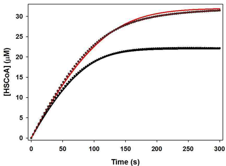
Figure 3.13: Experimental and simulated time courses for the steady-state reaction containing 0.022 \text{ } \mu\text{M} wild type YdiI and 20 (●) or 30 \text{ } \mu\text{M} (●) benzoyl-CoA in 50 \text{ mM}
