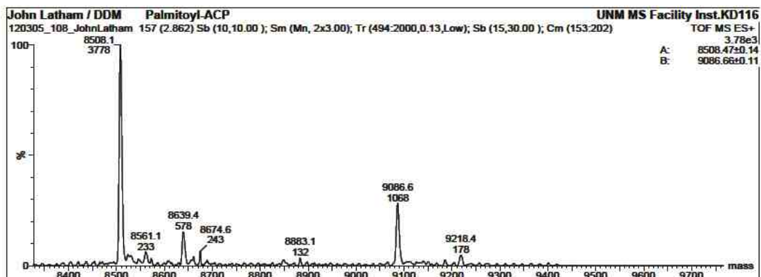
Figure 5.4: Exact molecular weight determination by TOF-ESI-MS of A - apoACP (predicted MW = 8507 Da), B - acetyl- holo ACP (predicted MW = 8890 Da), C - \beta -ketopropanone- holo ACP (predicted MW = 8902 Da), D - isobutyryl- holo ACP (predicted MW = 8917 Da), E - hexanoyl- holo ACP (predicted MW = 8945 Da), F - octanoyl- holo ACP (predicted MW = 8974 Da), G - lauroyl- holo ACP (predicted MW = 9031 Da) H - myristoyl- holo ACP (predicted MW = 9059 Da) and I - palmitoyl- holo ACP (predicted MW = 9085 Da). The product of thioester hydrolysis is holo ACP (predicted MW = 8847 Da).
