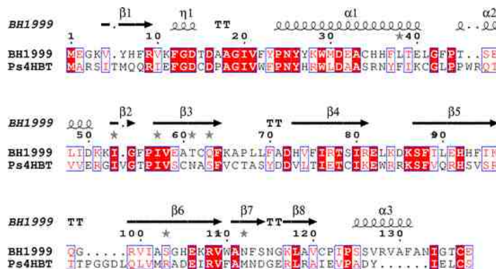
Figure 6.1: ESript generated sequence alignment of BH1999 and Pseudomonas sp. Strain CBS3 4-HBT where white font and red backgrounds represent identical residues and red font white background represents similar residues.
