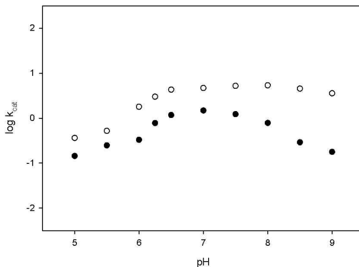
Figure 3.5 - Profile of pH dependence showing log k_{\text{cat}} vs. pH for the WT YdiI (○) and WT YdbB (●) catalyzed hydrolysis of 4-hydroxybenzoyl-CoA measured by direct assay at 300 nm and at 25°C.
