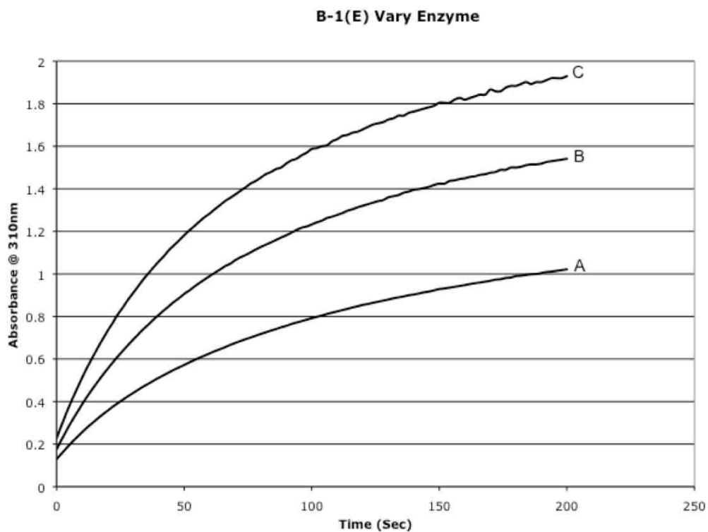
Figure 14. Plots of absorbances vs. time for LP catalyzed reactions of 1E to generate VAD using 200 \mu\text{M} 1E , 100 \mu\text{M} \text{H}_2\text{O}_2 and (A) 0.24 \mu\text{M} LP, (B) 0.36 \mu\text{M} LP, (C) 0.48 \mu\text{M} LP.
