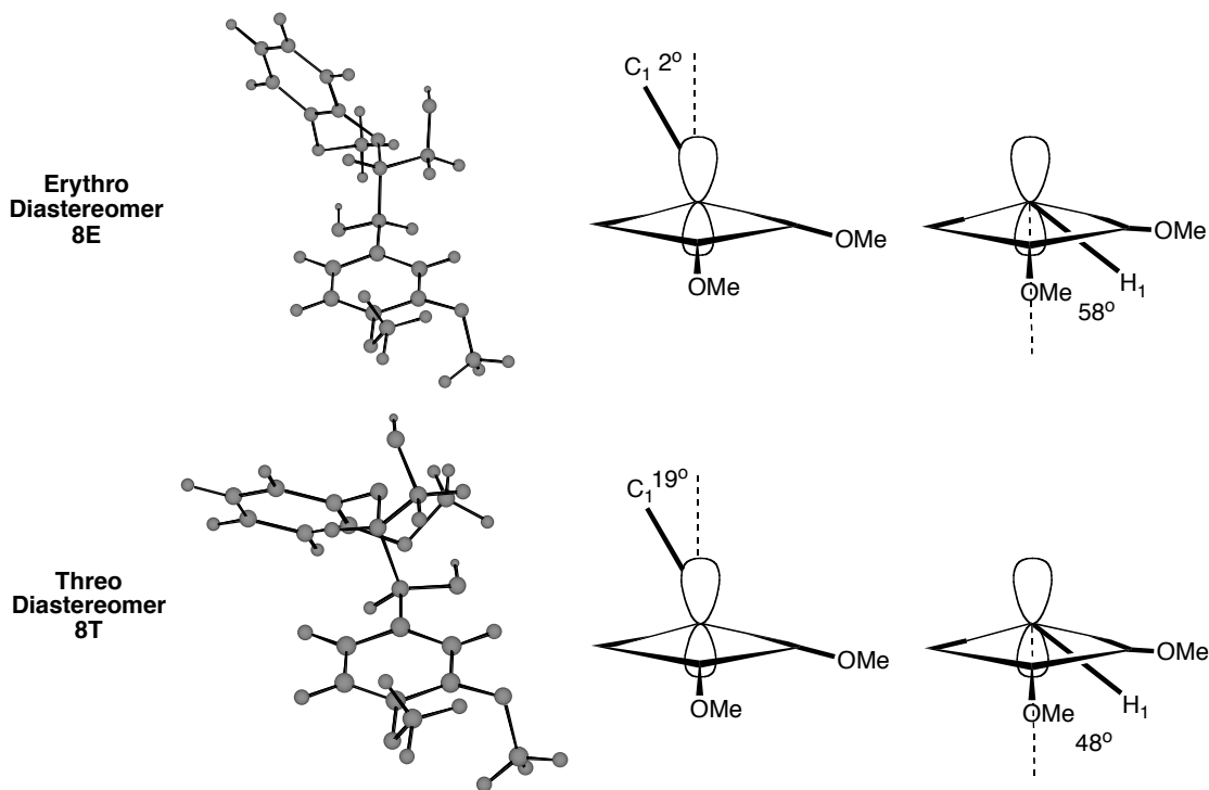
Figure 12. Summary of AMI Calculated Lowest Energy Conformers of 2E and 2T .
