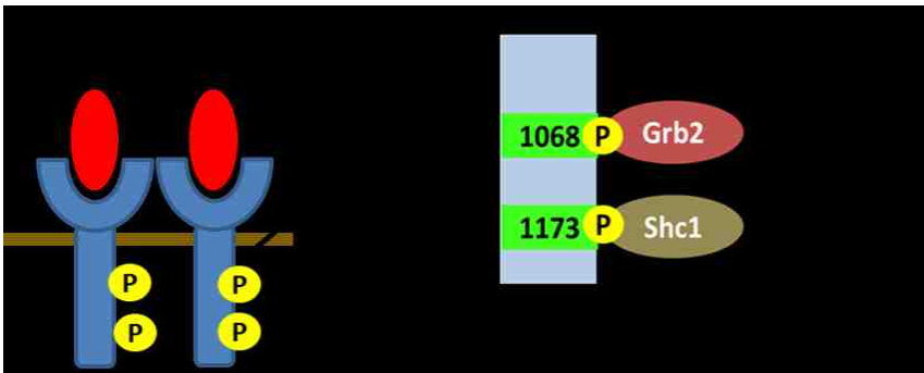
Figure 3.1. Graphical description of model. EGF-bound receptors can dimerize and phosphorylated each other. This model includes the phosphorylation of Y1068 and Y1173, and the recruitment of Grb2 and Shc1 to those respective sites.
