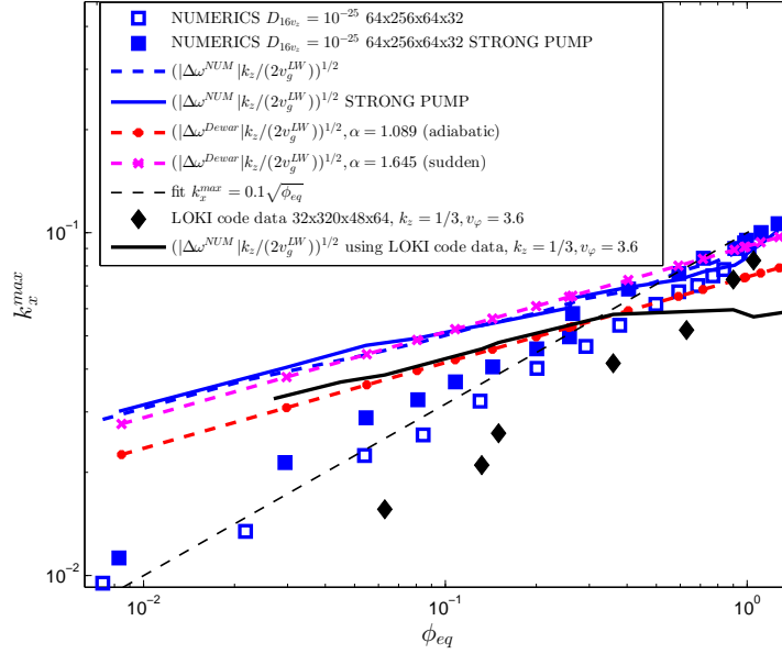
Figure 6.11: The wavenumber k_x^{max} at which the growth rate reaches the maximum as a function of \phi_{eq} for k_z = 0.35 , v_\phi = 3.488 .
