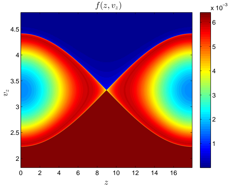
Figure 3.2: The phase space density distribution function f_{BGK}(z, v_z) of BGK mode with k_z = 0.35, \phi_0 = 0.3, v_\phi = 3.321836 .
