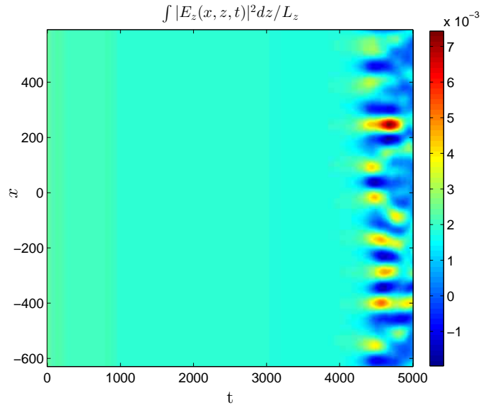
Figure 4.4: The density plot vs. x and t for \langle |E_z|^2 \rangle_z \equiv L_z^{-1} \int_0^{L_z} |E_z|^2 dz ( |E_z|^2 averaged over z ) shows a development of LW filamentation with time from the initial BGK mode.
