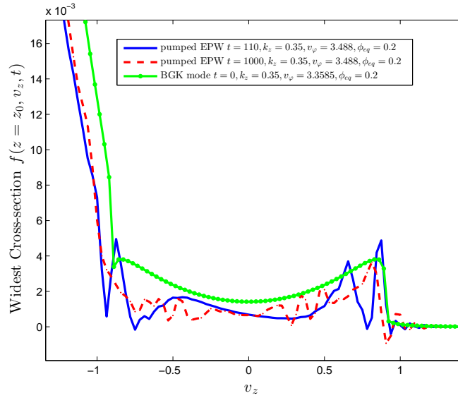
Figure 5.3: The widest cross-sections of f(z = z_0, v_z, t) of the trapping regions at t = 110 and t = 1000 of the weakly pumped EPW obtained with parameters k_z = 0.35 , v_\phi = 3.488 , \phi_{pump} = 0.01 , T_{off} = 110 and resulting \phi_{eq} = 0.2 in comparison with the widest cross-sections of the trapping region of BGK mode constructed analytically as in Chapter 3 with parameters k_z = 0.35 , \phi_{eq} = 0.2 and v_\phi = 3.3585 (according to the BGK dispersion relation (3.15)). z_0 is chosen such that the resulting cross-sections have the maximum width.
