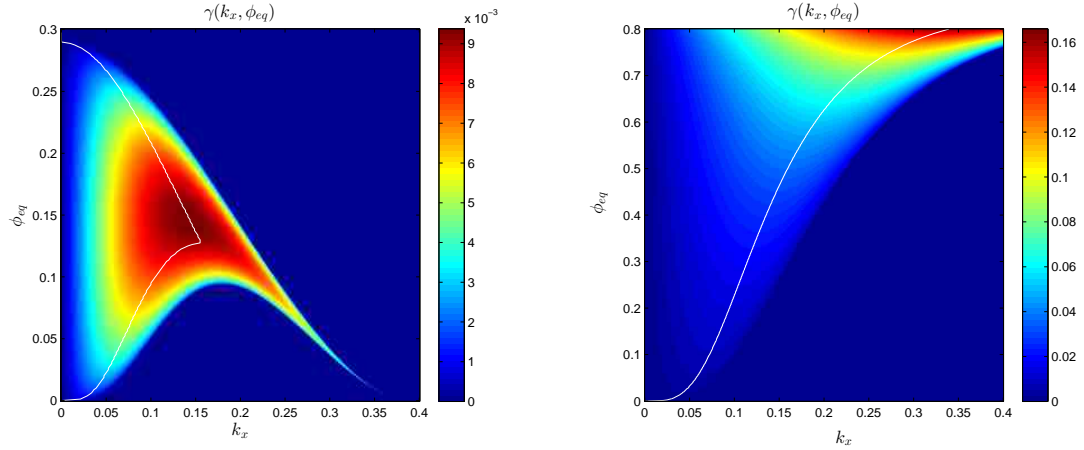
(a) Growth rates using D as in Eq. (3.25) (b) Growth rates using linear approximation for D as in Eq. (3.26)
