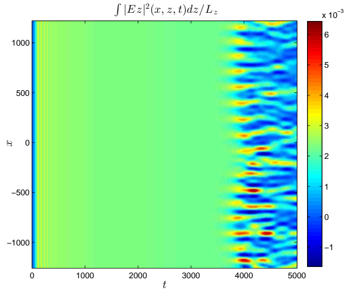
Figure 6.2: The density plot vs. x and t for \langle |E_z|^2 \rangle_z \equiv \int_0^{L_z} |E_z|^2 dz / L_z ( |E_z|^2 averaged over z ) shows a development of LW filamentation with time from the pumped EPW with k_z = 0.35 , \phi_{eq} \approx 0.2 .
