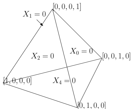
Figure 3.4: A picture of \mathbb{P}^3 with its standard decomposition.
