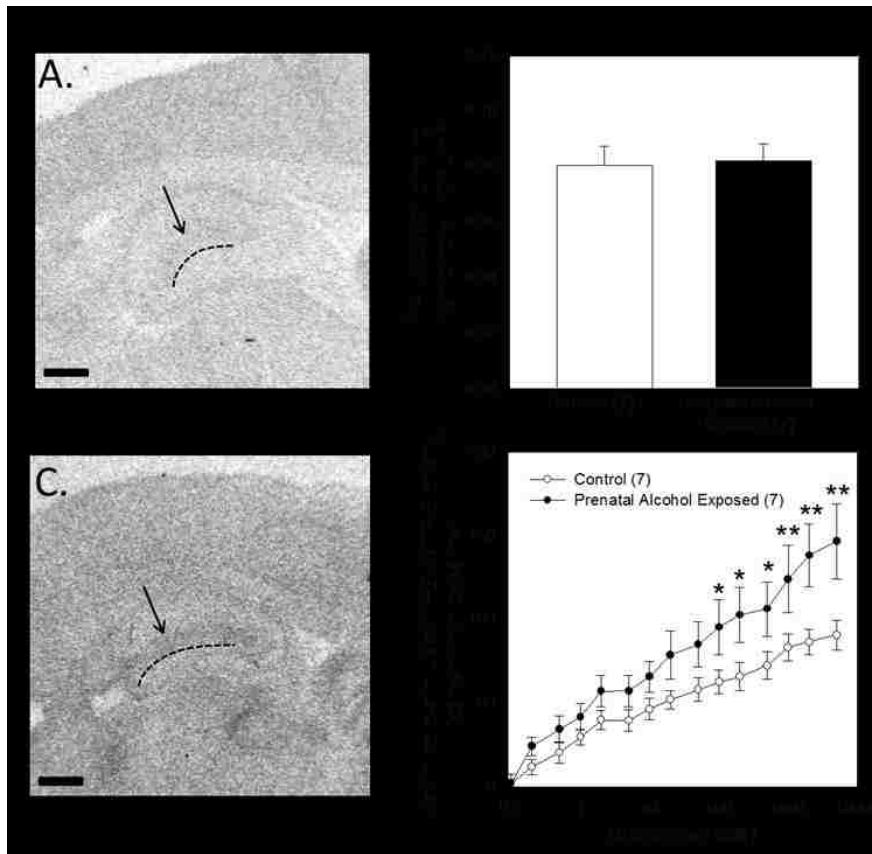
Figure 5.1 Impact of prenatal ethanol exposure on histamine H 3 receptor density and H 3 receptor effector coupling in the dorsal dentate gyrus of the rat brain.
