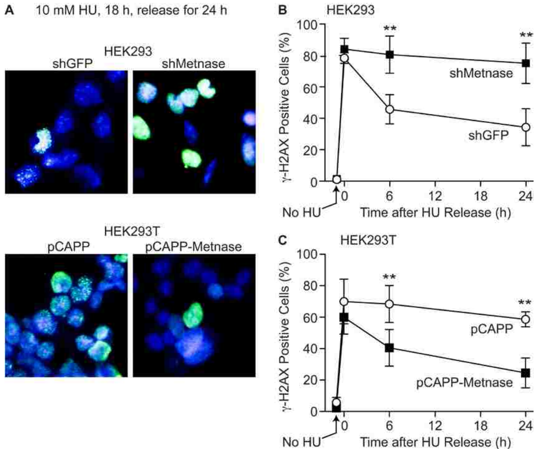
Figure 4-10. Metnase promotes resolution of replication stress-induced \gamma -H2AX.
