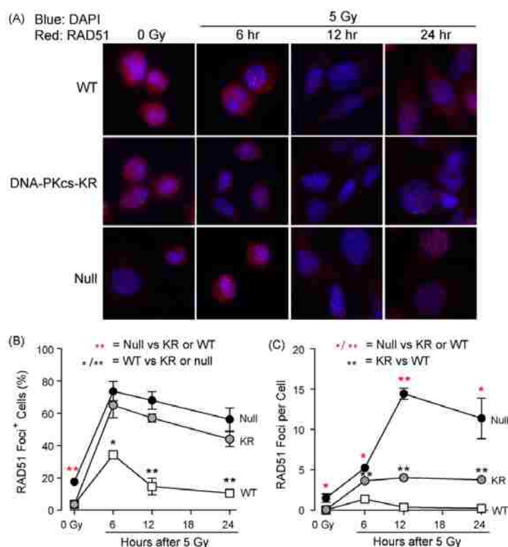
Fig. 3. IR-induced RAD51 foci resolve slowly in DNA-PKcs defective cells. (A) Representative immunofluorescent images of wild-type (A48), DNA-PKcs null (VD13) and DNA-PKcs-KR (VD13-KR4) cells mock-treated or treated with 5 Gy IR. RAD51 was detected with anti-RAD51 antibodies (red) 6, 12, or 24 h after IR. Nuclei were stained blue (DAPI). Magnification = 40 \times . (B and C) Percentage of cells with 1 or more RAD51 foci, and number of RAD51 foci per cell. Values are averages \pm SEM for three sets of images, with an average of 105 cells scored per data point. (*) indicates P < 0.05 ; (**) indicates P < 0.01 .
