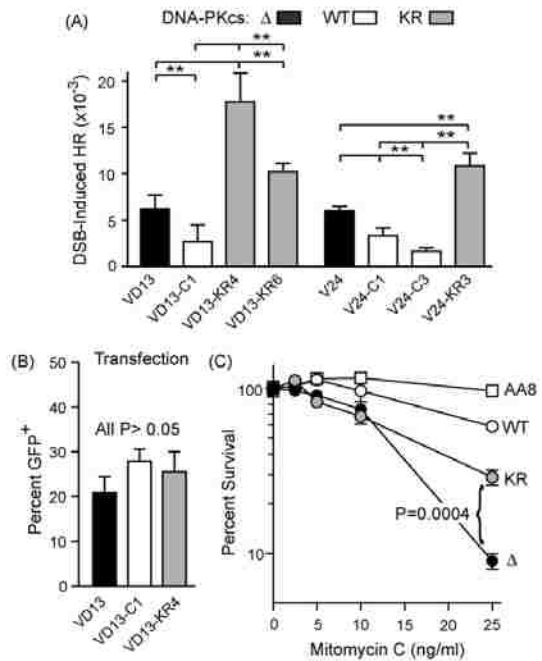
Fig. 2. DNA-PKcs-KR enhances HR. (A) DSB-induced HR frequencies are shown for cells expressing wild-type DNA-PKcs, DNA-PKcs-KR, or null ( \Delta ). Values are averages ( \pm SD) for 3–5 determinations. Double asterisks indicate significant differences at P \leq 0.01 ( t -tests). (B) GFP transfection efficiencies measured by flow cytometry. (C) Percent survival as a function of MMC concentration in wild-type (AAB and VD13-C1), DNA-PKcs-KR (VD13-KR4), and null (VD13) cells. Values are averages ( \pm SD) for 3 determinations.
