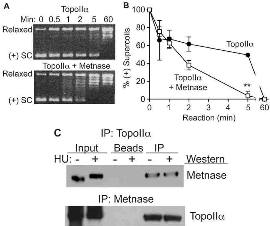
Figure 4-12. Metnase interacts with Topoll \alpha and stimulates relaxation of positive supercoils.
