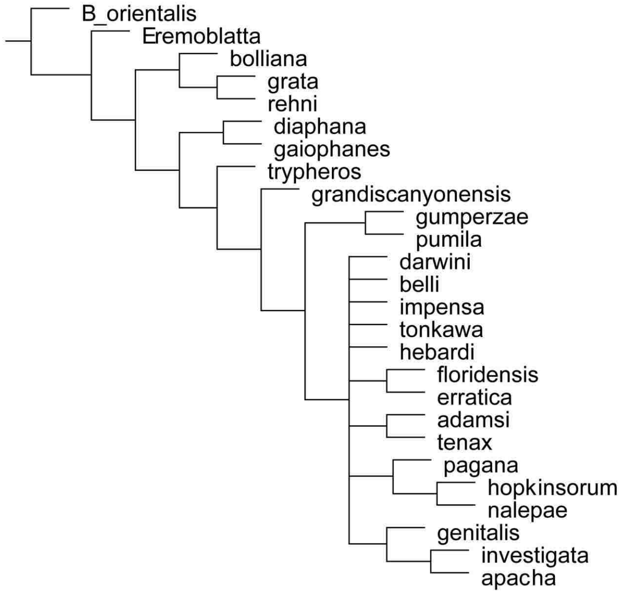
Figure S4. 12S Parsimony Tree.
