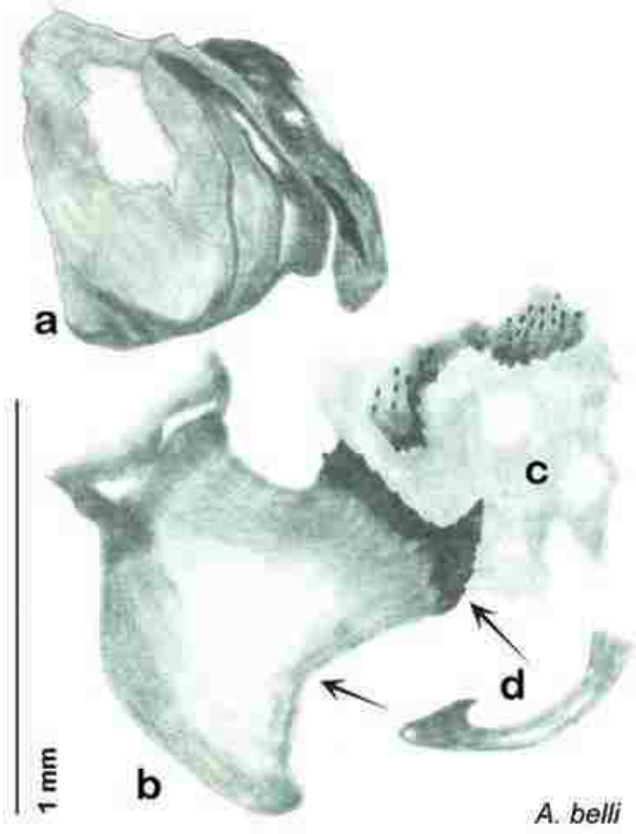
Figure 31. A. belli , genitalia: a right dorsal phallomere b right ventral phallomere c small central sclerite d genital hook. Arrow(s) indicate diagnostic characters (see text).
