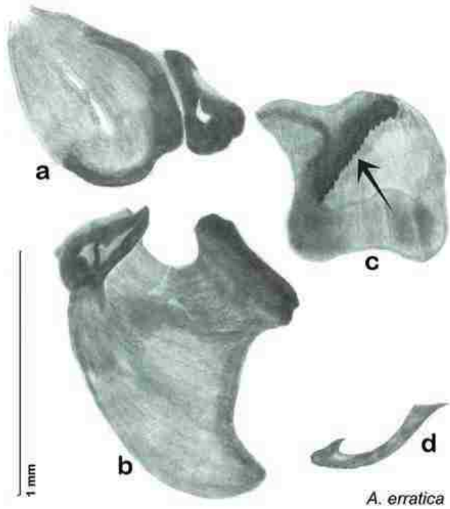
Figure 49. A. erratica , genitalia: a right dorsal phallomere b right ventral phallomere c small central sclerite d genital hook. Arrow(s) indicate diagnostic characters (see text).
