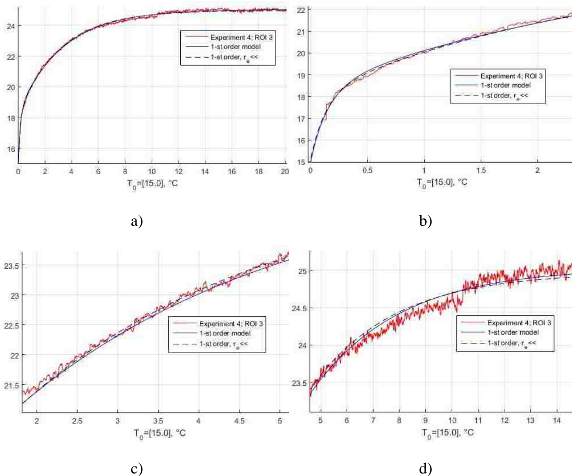
Figure 5.1. Nonlinear fit of the experimental data for TR-1 e and TR-1 r e << in the whole time range a) for 0...2 min b), 2...5 min c), and 5...15 min d).
