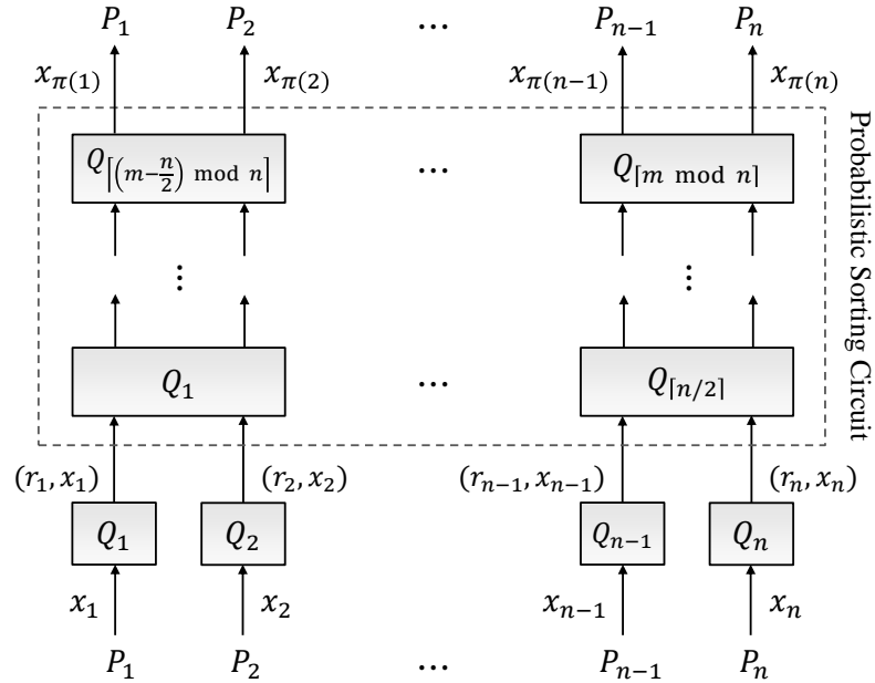
Figure 3.3: MPS circuit
