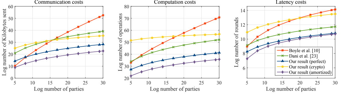
Figure 3.4: Communication cost (left), computation cost (middle), and the number of communication rounds (right)
