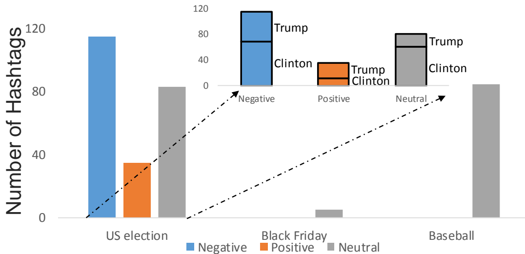
Figure 3.6: Histogram for labeled keyword sentiment for all the datasets.
