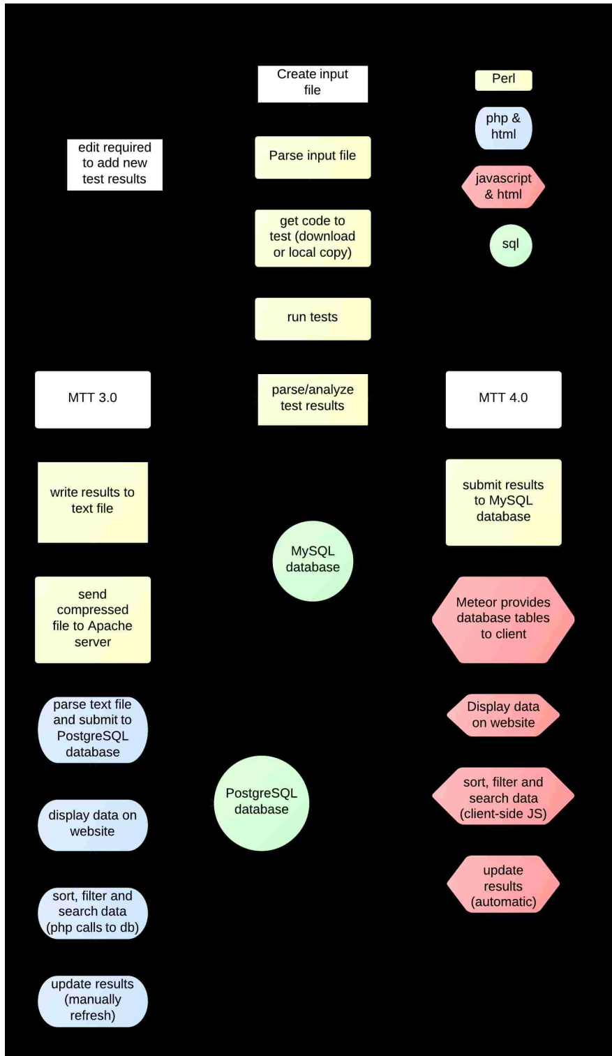
Figure 4.2: Flow chart comparing MTT 3.0 and MTT 4.0
