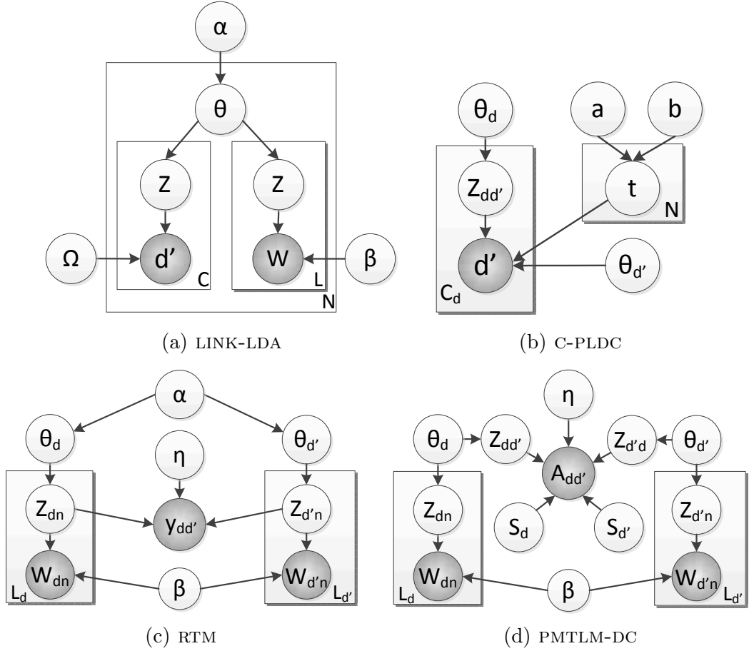
Figure 4.1: Graphical models for link generation.
