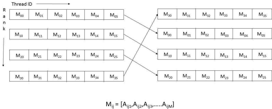
Figure 5.4: Input and Output Matrice for MPI_Put(). The M are arrays of values of the specified MPI datatype.
