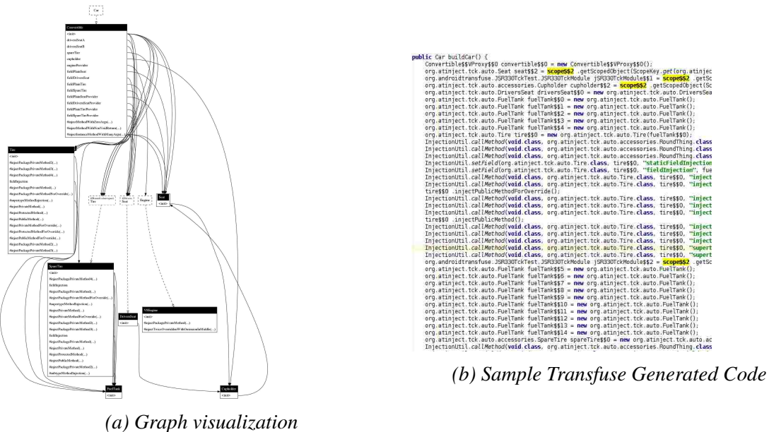
Figure 4.3: Example JSR330 injection graph. This graph contains 8 classes and 66 injection points. Transfuse builds this graph through 382 lines of injection graph code.
