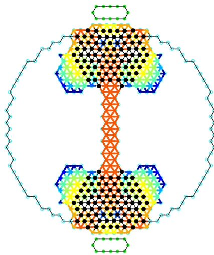
(a) Deformed shape for simulation time of 32 fundamental periods
