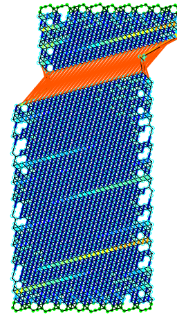
(b) Deformed shape at time step 126100 for lattice rotation of 15^\circ
