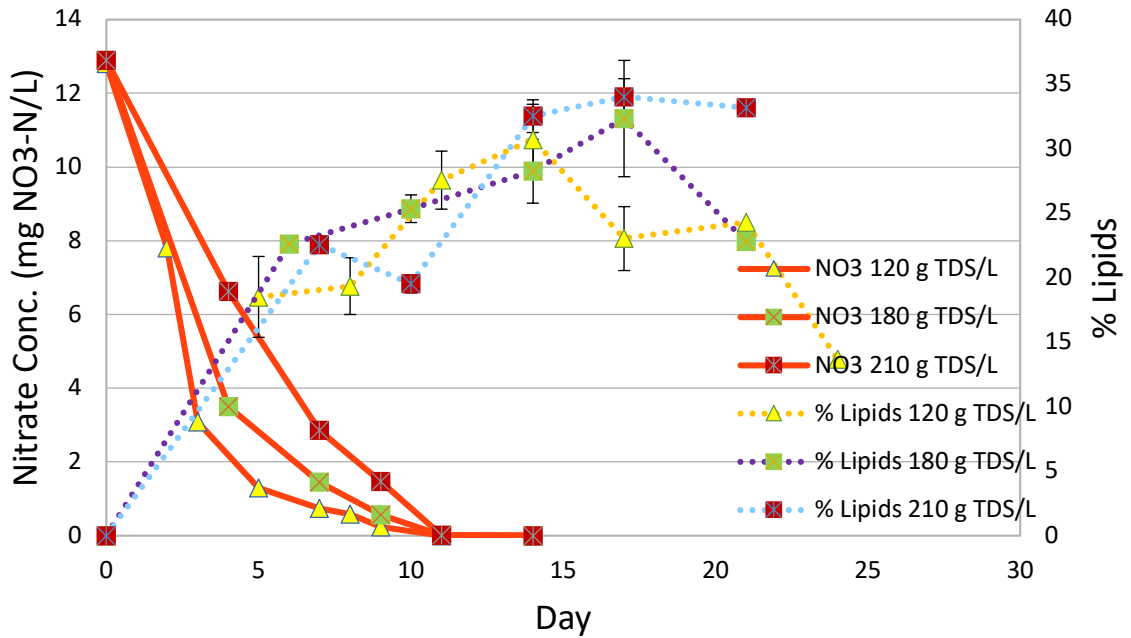
Figure 3.4. 24: D. tertiolecta PW (Exp. D1) nitrate concentration and lipid content for 120, 180, and 210 g TDS/L conditions.
