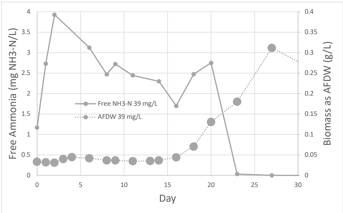
Figure 3.5. 7: Estimated free ammonia and measured biomass densities for D. tertiolecta in 120 g TDS/L PW media at an initial concentration of 39 mg NH 4 -N/L.
