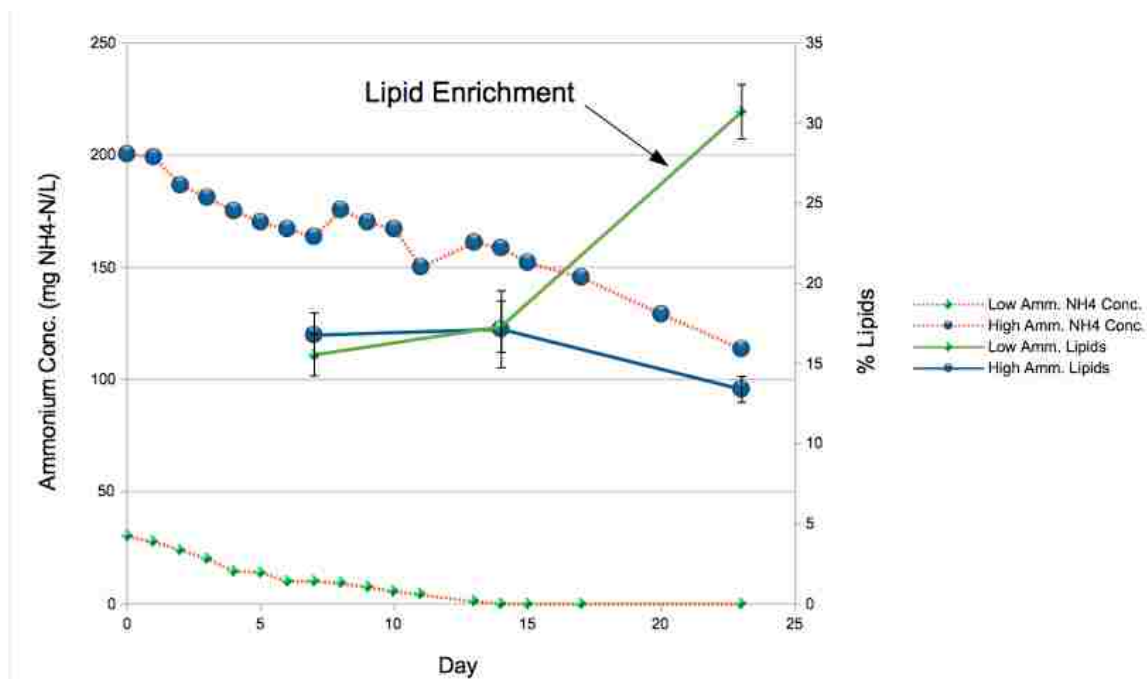
Figure 3.3. 35: Polyculture lipid content and ammonium measurements for tubular reactor with initial Ammonium of 30 and 200 mg NH4-N/L.
