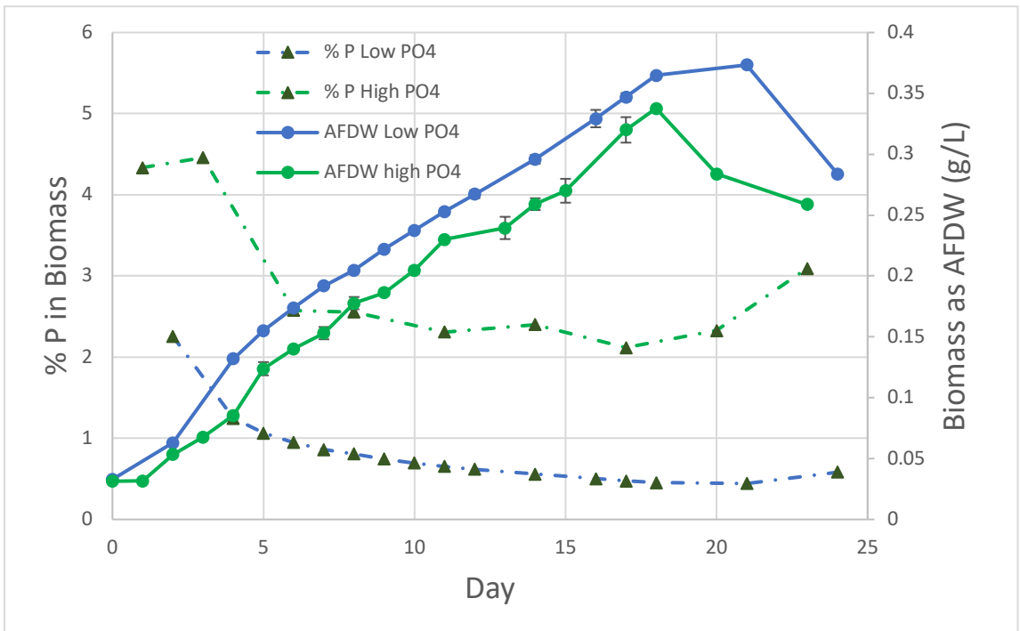
Figure 3.4. 44: D. tertiolecta biomass measurements and % phosphorus in a 120 g TDS/L PW and 13 mg NH 4 -N/L media at low (1.7 mg PO 4 -P/L) and high (8 mg PO 4 -P/L) initial concentrations.
