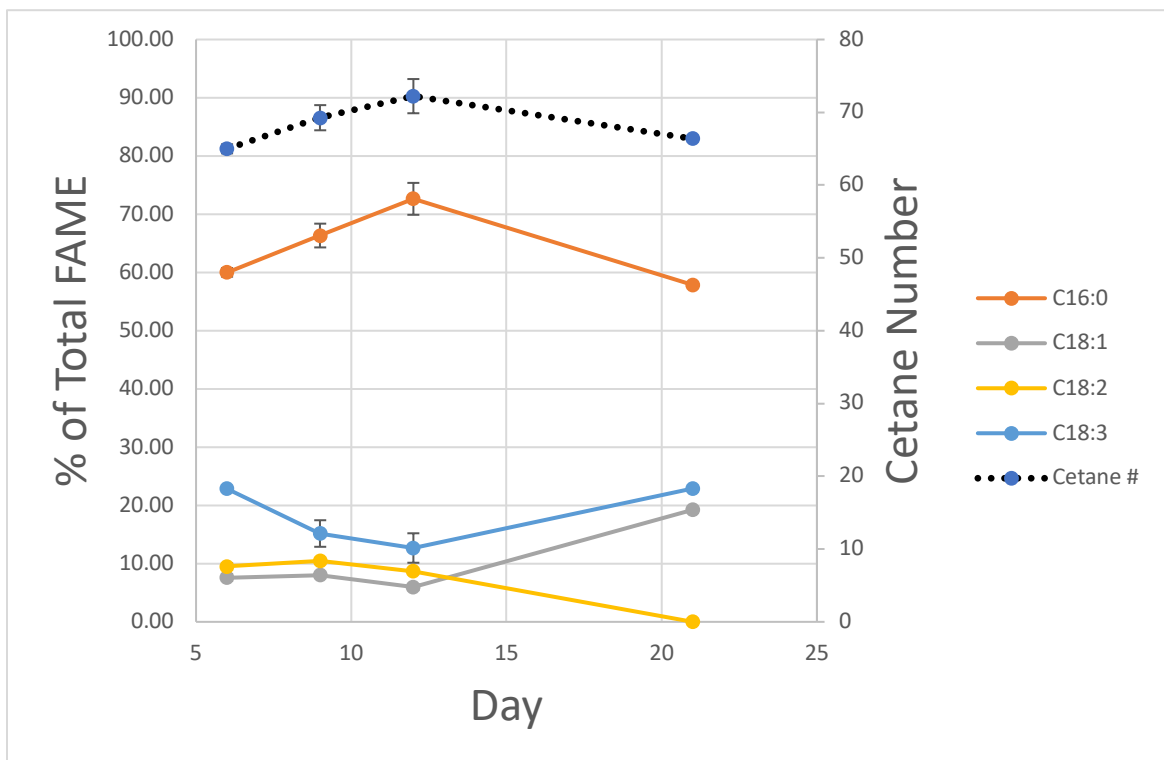
Figure 3.4. 29: D. tertiolecta PW flask experiment % FAME and cetane number for the 60 g TDS/L condition using nitrate.
