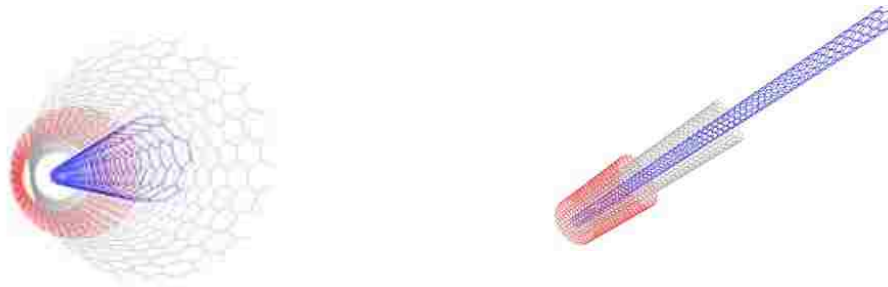
Figure 13.MWCNTs
