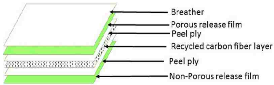
Figure 18.Composite layers
