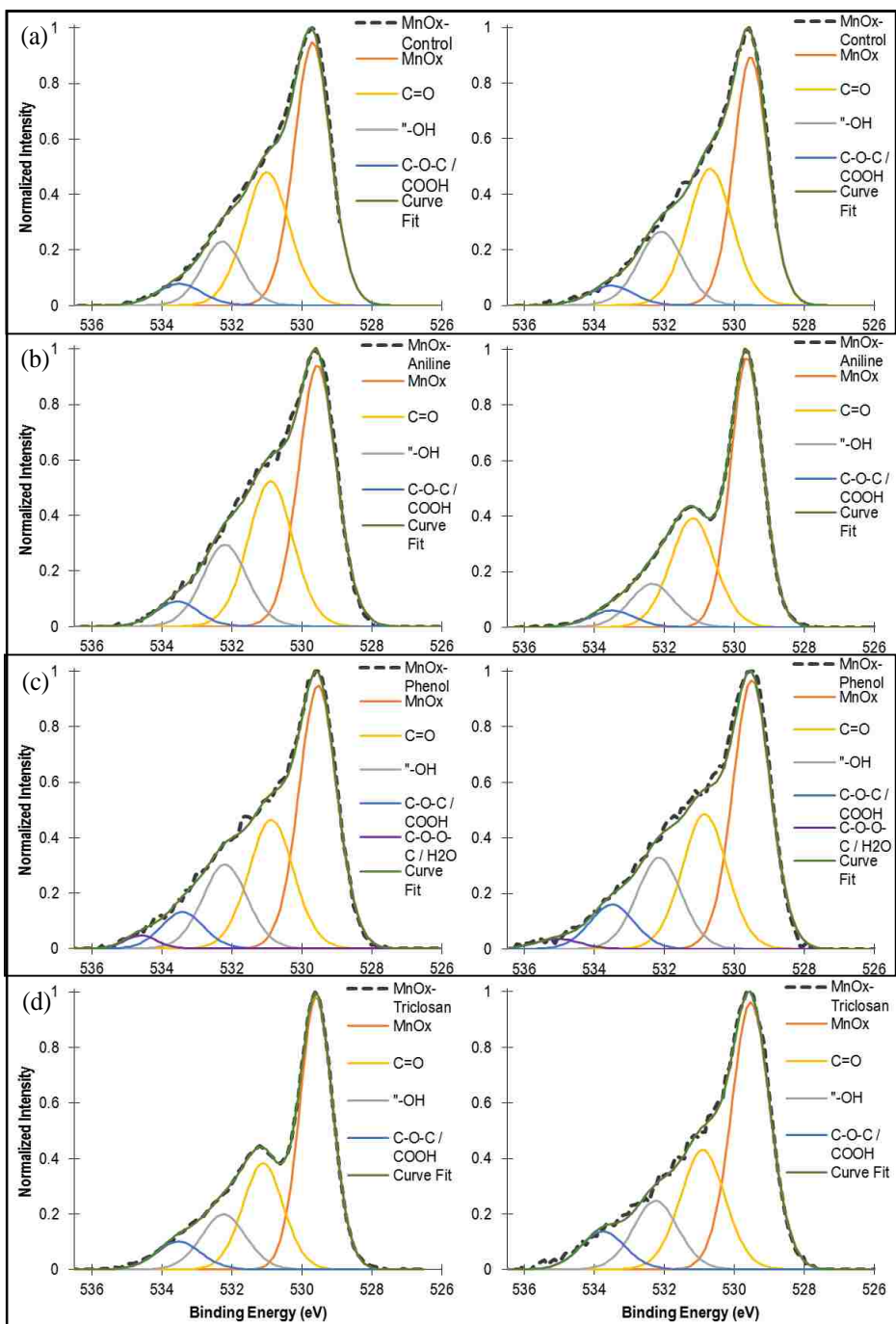
Figure S4. Fitting of O 1s XPS high resolution spectra for replicate samples of (a) \text{MnO}_x Control (b) \text{MnO}_x Aniline (c) \text{MnO}_x Phenol (d) \text{MnO}_x Triclosan. The unknown sample data is shown as black dashed line; the solid green line is the overall contribution due to fitting of different types of oxygen bonds.
