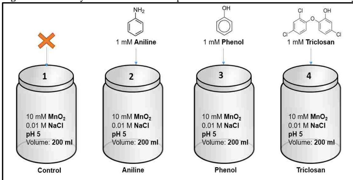
Figure S1. Summary of the batch reaction experiment conditions and reactors for this study
