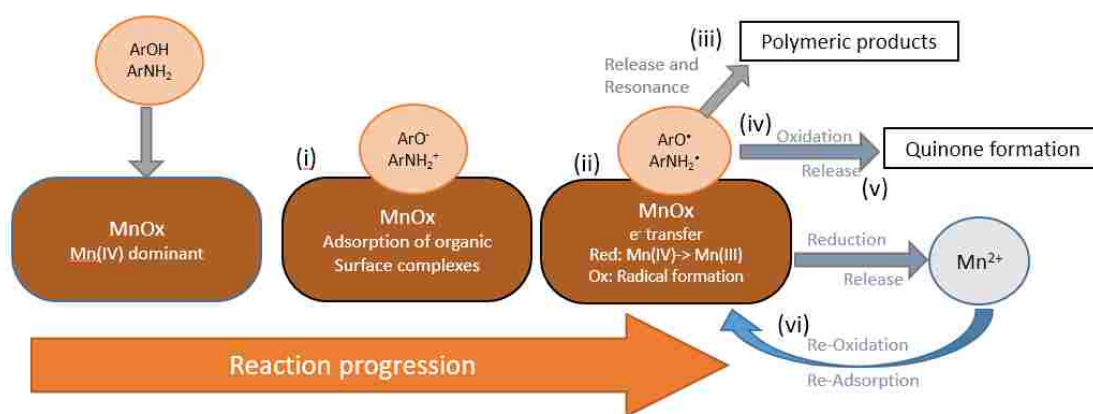
Figure 1 Proposed reaction mechanism for reaction of Phenols ( \text{ArOH} ) and Aniline ( \text{ArNH} ) with \text{MnO}_x
