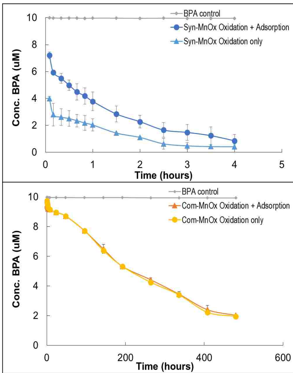
Figure S7. BPA removed by oxidation and adsorption vs. BPA removed by oxidation alone. Reaction conditions: 100 \mu\text{M} \text{MnO}_x , 10 \mu\text{M} BPA, 10 mM NaCl, pH 5.0
