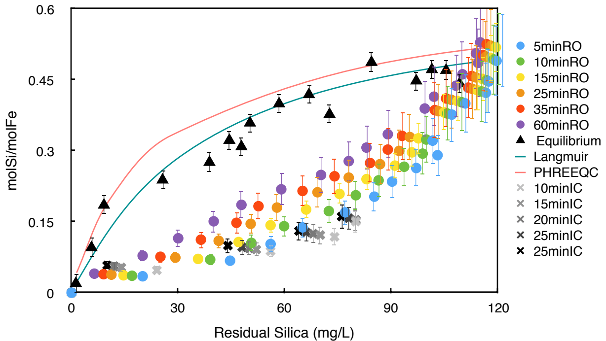
Figure 37. Results of data analysis for SBR and equilibrium adsorption experiments, along with langmuir and PHREEQC adsorption Isotherm models
