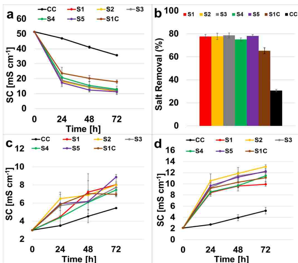
Figure 12. Desalination chamber solution conductivity (a), desalination chamber salt removal (b), anode chamber solution conductivity (c), cathode chamber solution conductivity (d).
