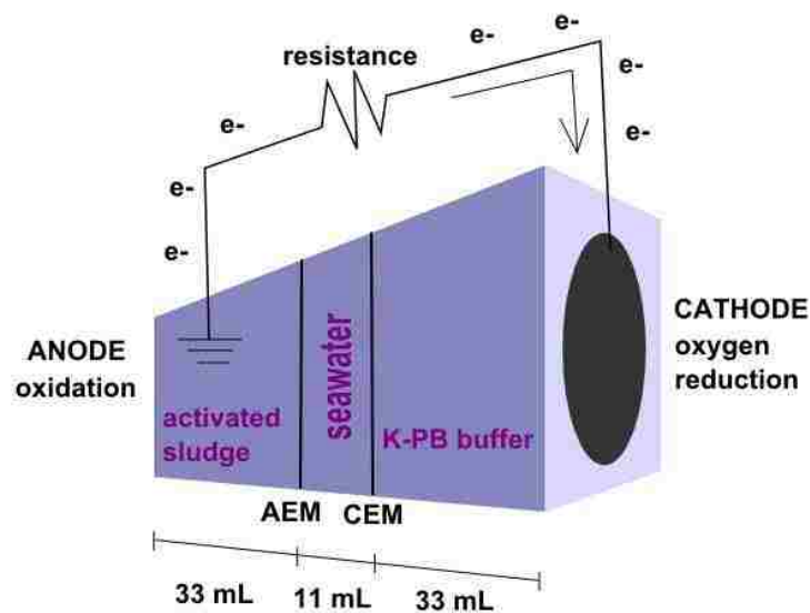
Figure 2. Schematic of microbial desalination cell set up used for this study.
