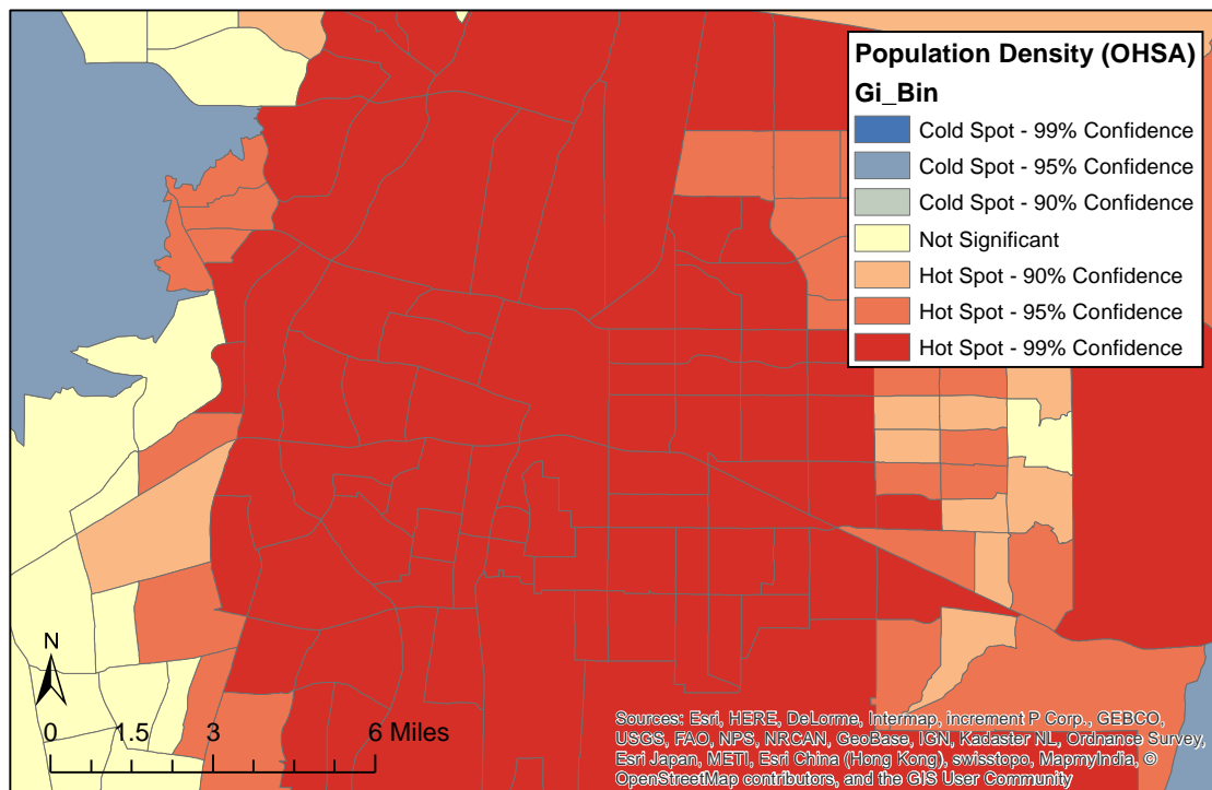
Figure 26. OHSA for population density within each census tract
