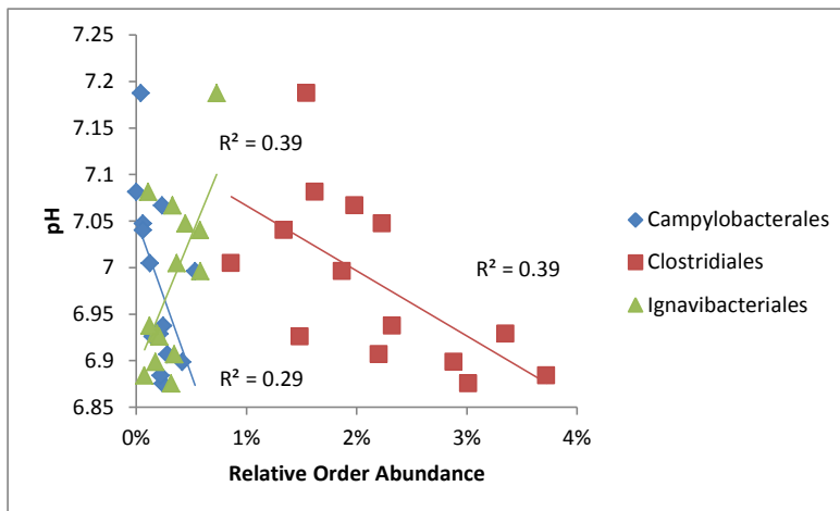
Figure 7.9: The relationship between pH and significantly correlated ( \alpha < 0.05 ) \epsilon -Proteobacteria, Firmicutes and Chloroflexi relative abundance
