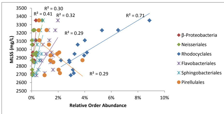
Figure 7.7: The relationship between MLSS and significantly correlated ( \alpha < 0.05 ) \beta -Proteobacteria (diamonds), Bacteroidetes (asterisks), and Planctomycetes (circle) relative abundance
