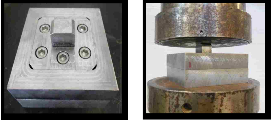
Figure 3.6: Compaction Apparatus and compaction loading
