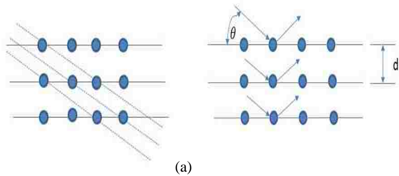
Figure 3.19: (a) Crystalline structure of atomic planes (b) Bragg's Law diffractive x-rays
