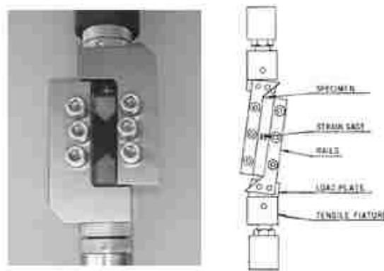
Figure 2.12: Double rain shear fixture (ASTM D4255).
