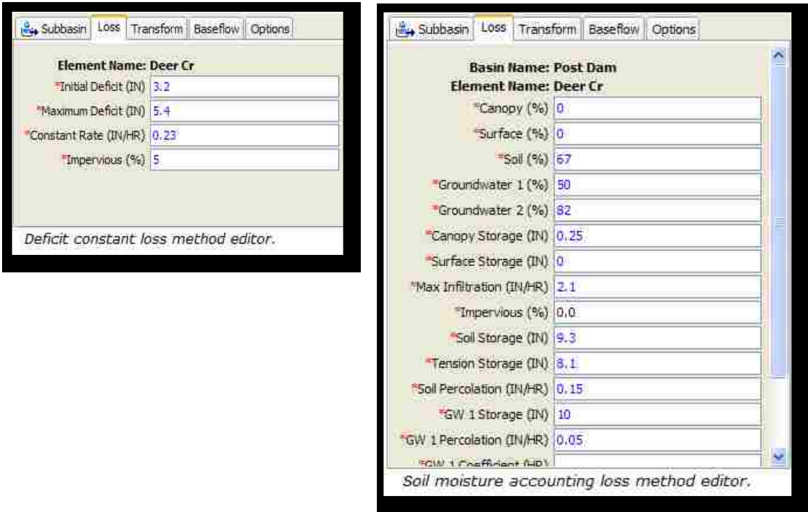
Figure 21: Parameters for Loss Methods (HEC-HMS 3.4 User’s Manual)
