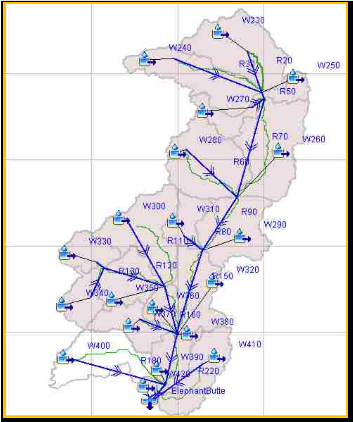
Figure 8: Watershed Delineation using HEC-GeoHMS
