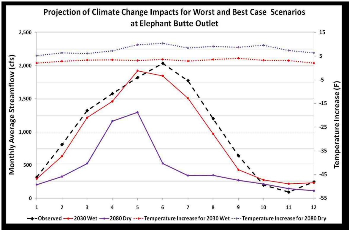
Figure 40: Streamflow Projection for Worst and Best Case Scenarios at Elephant Butte Outlet
