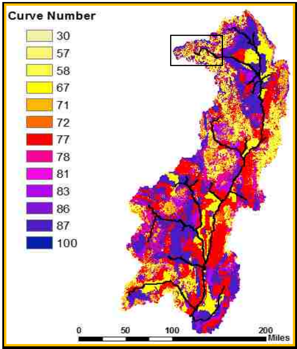
Figure 13: Gridded Curve Number of the Delineated Watershed
