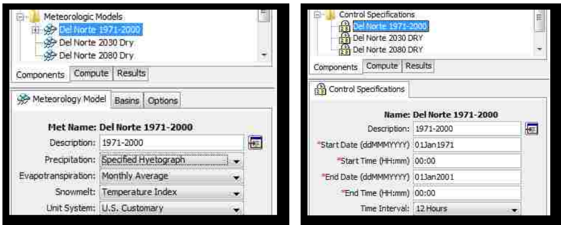
Figure 4: Examples of a Meteorologic Model and the Control Specifications
