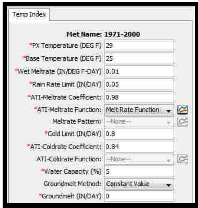
Figure 19: Selection of Temperature Index Parameters
