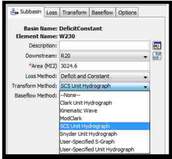
Figure 22: Selection of Transform Method
