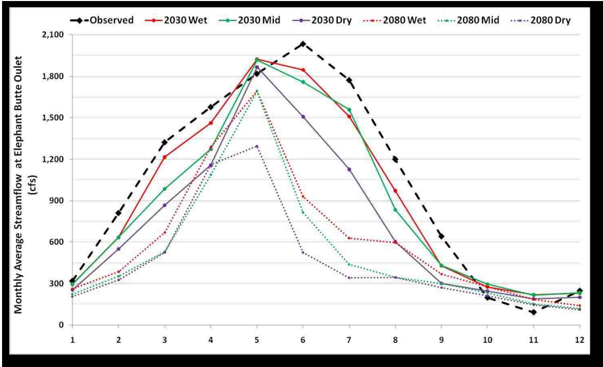
Figure 37: Projection of Streamflows at Elephant Butte Outlet
