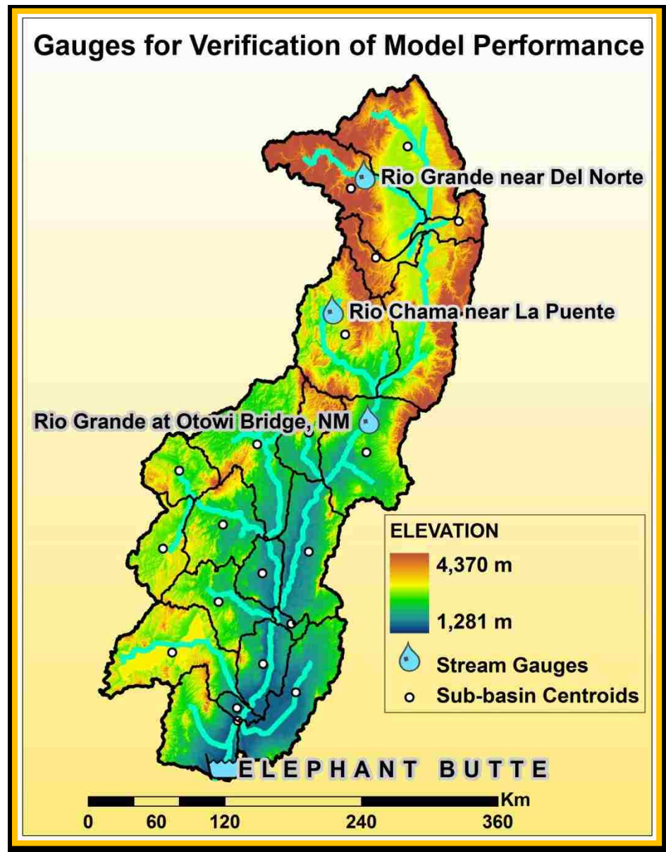
Figure 15: Control Gauges
