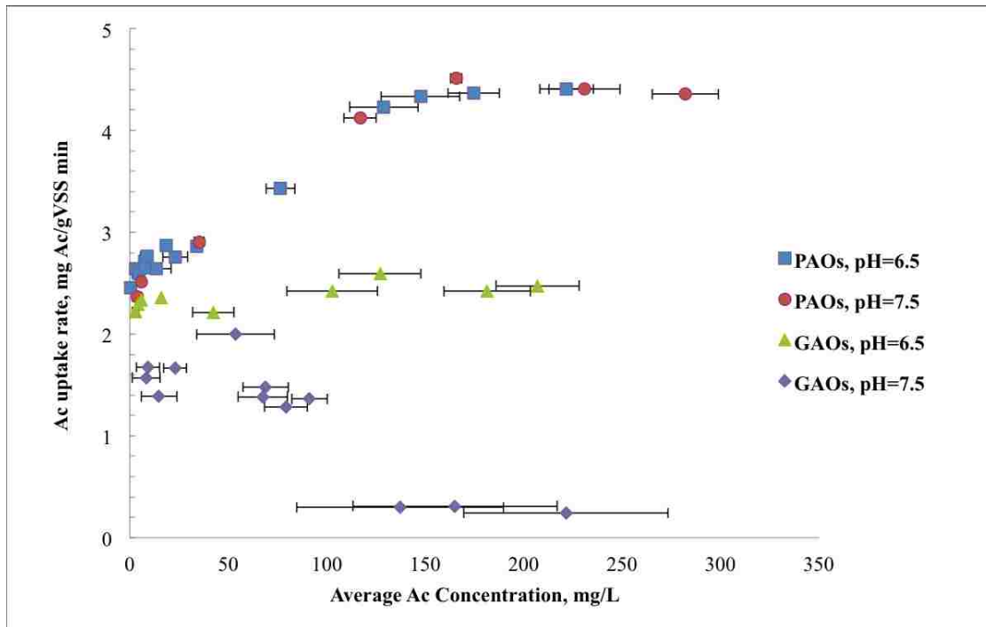
Figure 6.9 Acetate uptake rates in Accumulibacter spp. and Defluviicoccus spp. enriched culture under different pH values.
