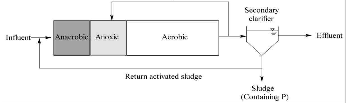
Figure 2.14 A 2 /O process
