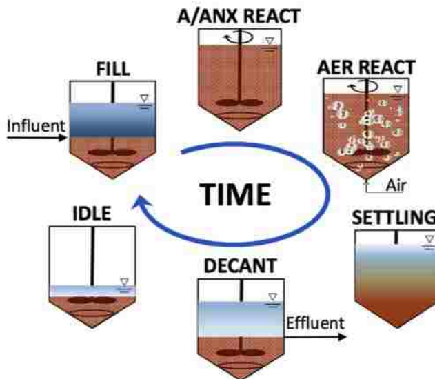
Figure 2.2 Activated sludge with anaerobic/aerobic reactor
