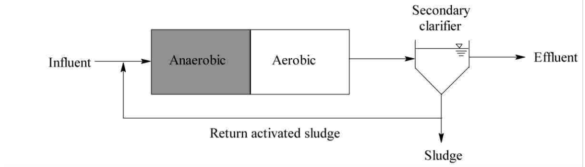
Figure 2.13 A/O process
