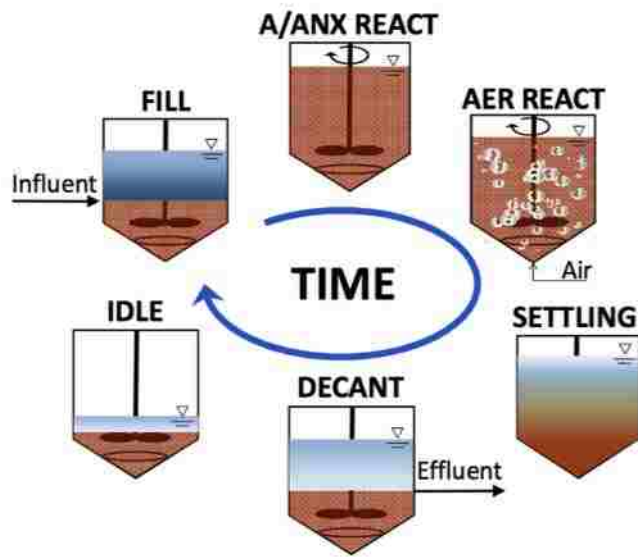
Figure 2.17 SBR process
