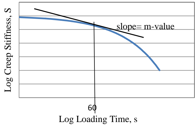
Figure 2.13: Example log creep stiffness vs log loading time showing line of m-value slope.
