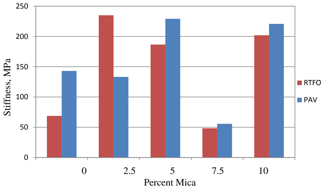
(b) Average stiffness vs mica concentration
