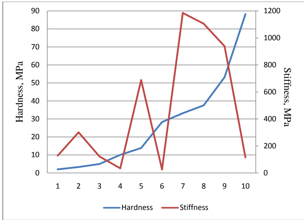
Figure 6.6: Stiffness and Hardness compared to each other, 10% mica mastic, RTFO
