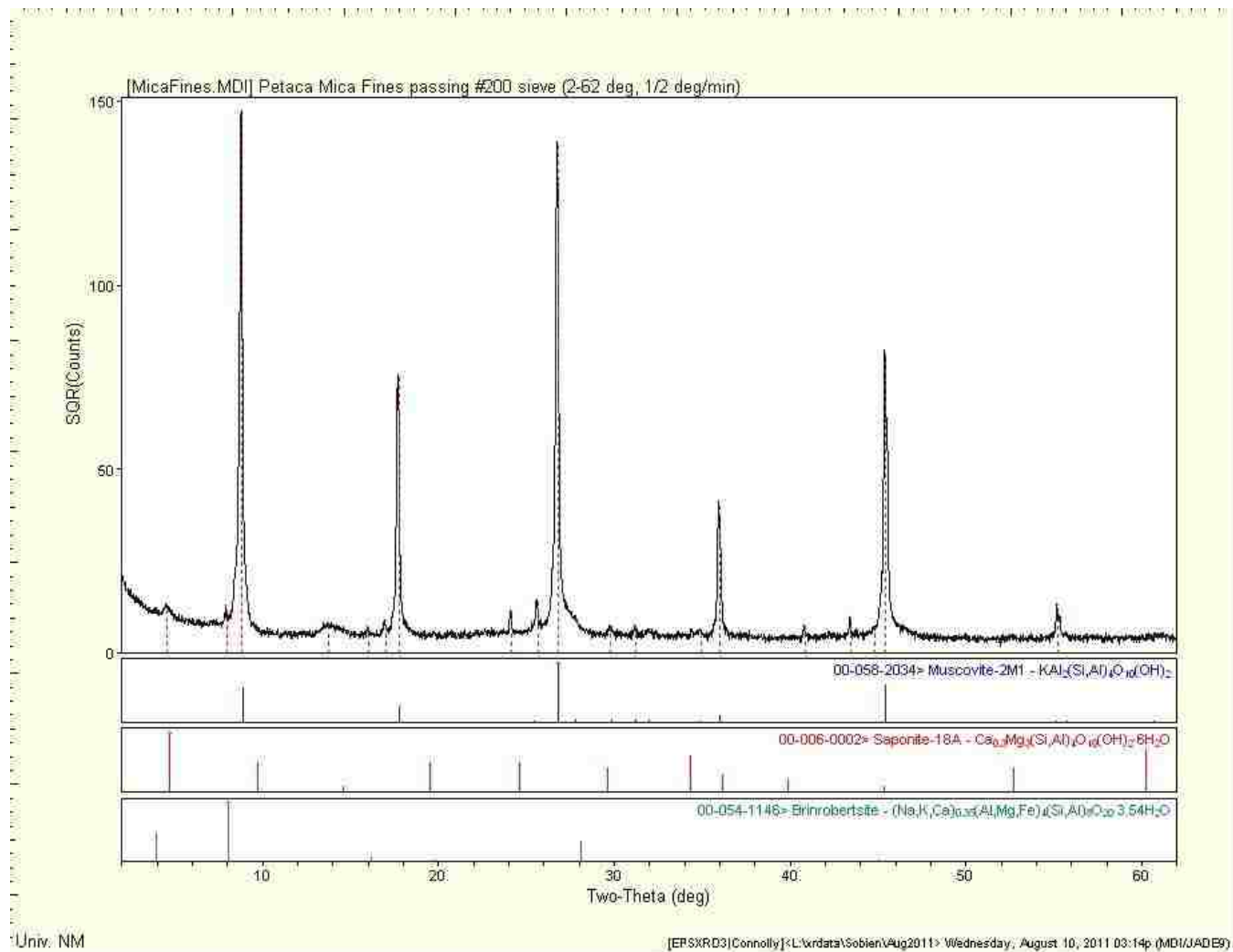
Figure 5. 1: XRD pattern of mica alone
